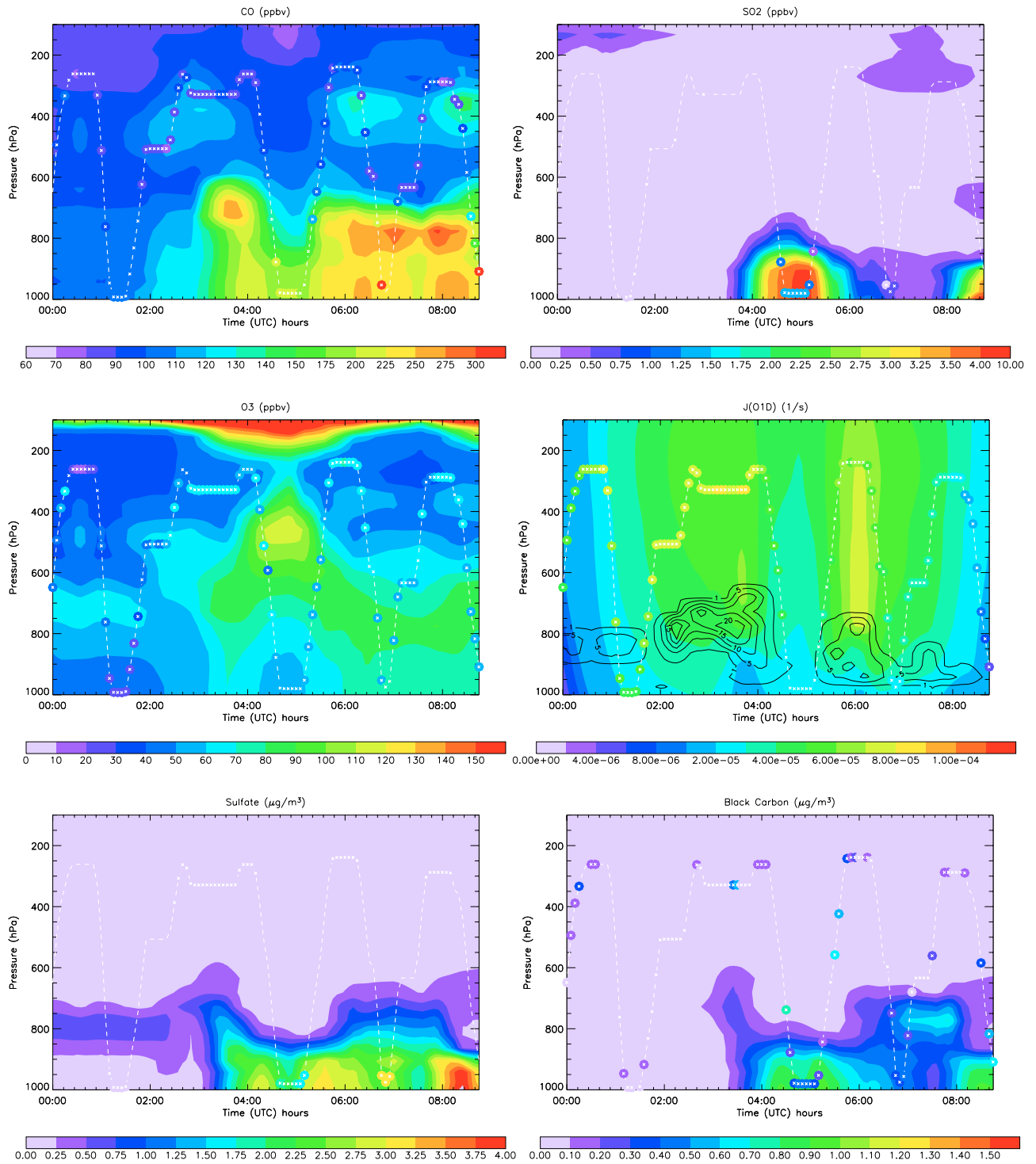
Figure 9. CO, SO 2 , O 3 , J 01D , sulfate and black carbon vertical columns calculated by the model along the DC8-06 flight track. The colored circles represent the 5 min averaged observations. The contour lines plotted over J 01D represent the cloud optical depth calculated by the model.
