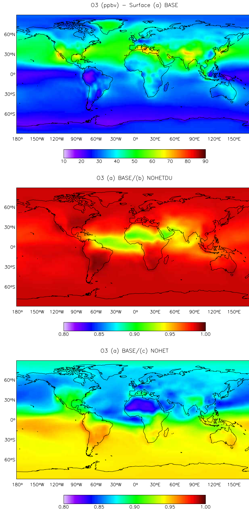
Figure 11. Annual mean O 3 surface concentration (ppbv) for the standard simulation BASE and the ratios BASE/NOHETDU and BASE/NOHET.
