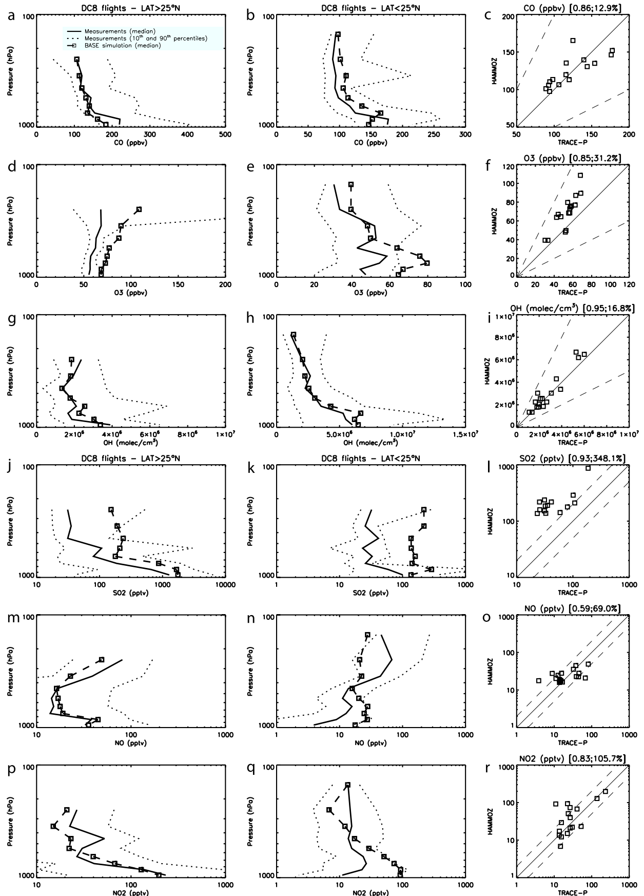
Figure 3. Same as Figure 2 for (a–c) CO (ppbv), (d–f) O 3 (ppbv), (g–i) OH (molecules/cm 3 ), (j–l) SO 2 (pptv), (m–o) NO (pptv) and (p–r) NO 2 (pptv).
