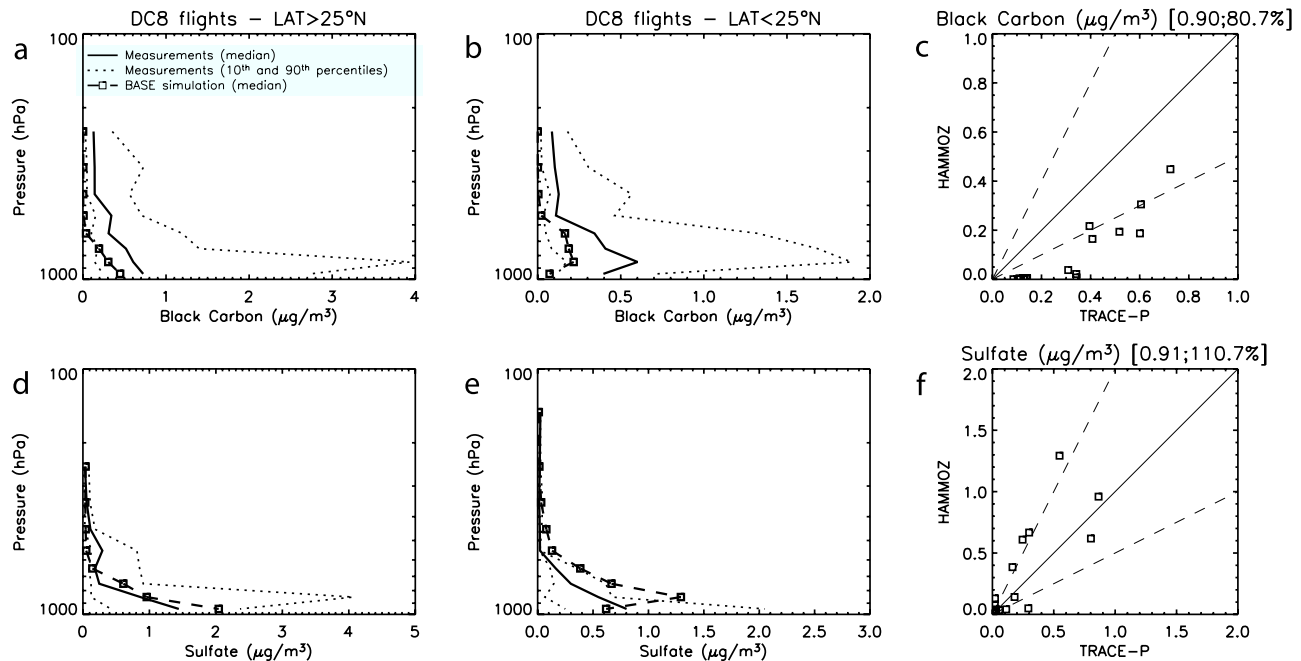
Figure 5. Same as Figure 2 for (a–c) black carbon and (d–f) sulfate aerosol concentrations ( \mu\text{g}/\text{m}^3 ).
