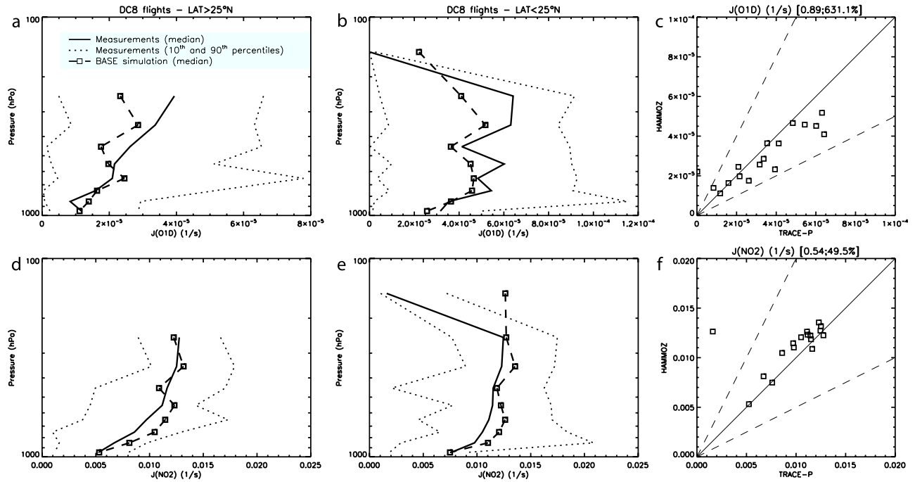
Figure 4. Same as Figure 2 for (a–c) J_{O1D} (1/s) and (d–f) J_{NO2} (1/s).
