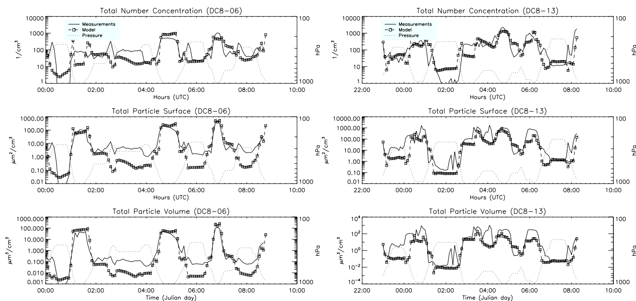
Figure 8. Observed (black line) and calculated (black dashed line and open squares) particle ( 0.05 > r > 1 \mu\text{m} ) number concentrations, surfaces and volumes along the DC8-06 and DC8-13 TRACE-P flights. The dotted black lines show the pressure levels along the flight tracks (right y axis).
