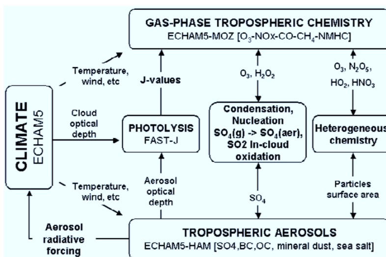
Figure 1. Schematic of the aerosol-chemistry-climate model ECHAM5-HAMMOZ.
