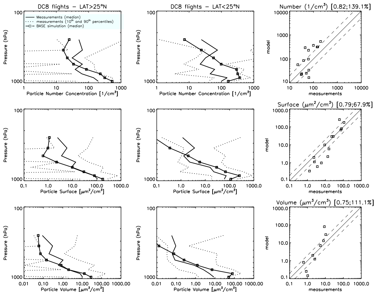
Figure 7. Same as Figure 2 for (a–c) particle number concentrations ( 1/\text{cm}^3 ), (d–f) particle surface ( \mu\text{m}^2/\text{cm}^3 ) and (g–i) particle volume ( \mu\text{m}^3/\text{cm}^3 ).
