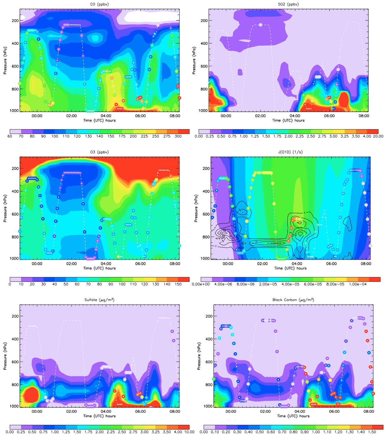
Figure 10. CO, SO 2 , O 3 , J O1D , sulfate and black carbon vertical columns calculated by the model along the DC8-13 flight track. The colored circles represent the 5 min averaged observations. The contour lines plotted over J O1D represent the cloud optical depth calculated by the model.
