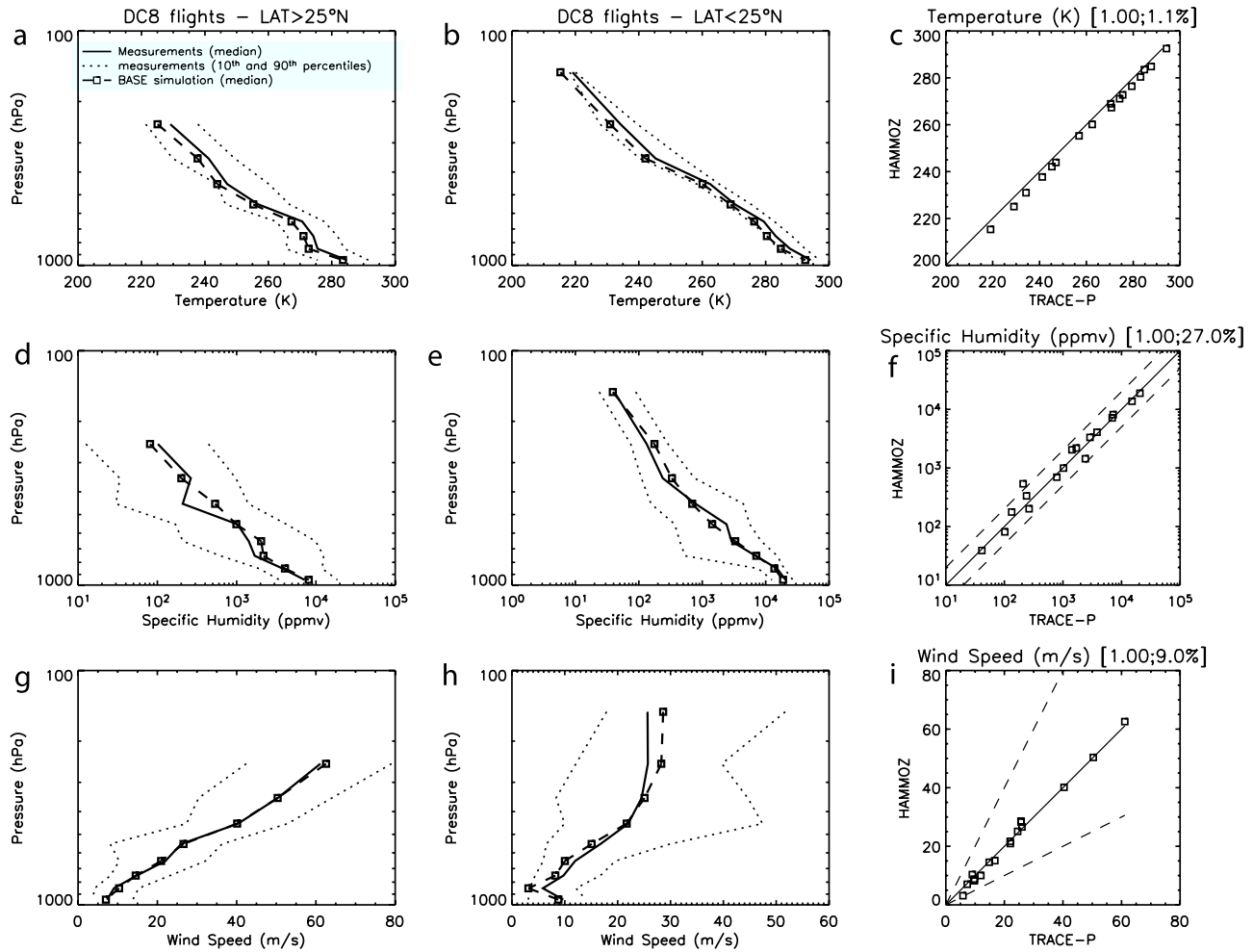
Figure 2. Vertical profiles of simulated (open square and dashed line) versus observed (solid line) medians of (a–c) temperature (K), (d–f) specific humidity (ppmv) and (g–i) wind speed (m/s) for the ensemble of TRACE-P DC8 observations (flights 6 to 17) in two different regions, latitude > 25^\circ\text{N} (Figures 2a, 2d, and 2g) and latitude < 25^\circ\text{N} (Figures 2b, 2e, and 2h). The model results (output every 3 h) were interpolated along the aircraft flight tracks and the data (mean averaged every 5 min) were binned in 100-hPa vertical intervals. The dotted lines represent the 10th and 90th percentiles of the observed quantities. The correlation between observed and simulated variables for the entire region (dashed lines represent the 1:2 and 2:1 ratios) is shown in Figures 2c, 2f, and 2i. The correlation coefficient and the mean absolute bias (%) are indicated in square brackets.
