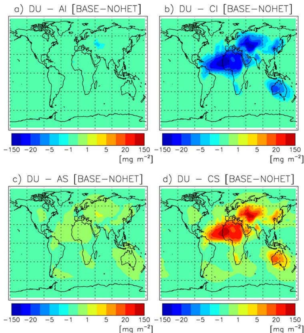
Figure 4. Annual mean burdens differences ( \text{mg}/\text{m}^2 ) between BASE and NOHET simulations of mineral dust in the (a) accumulation (DU-AI) and (b) coarse hydrophobic (DU-CI) modes and in the (c) accumulation (DU-AS) and (d) coarse (DU-CS) hydrophilic modes.
