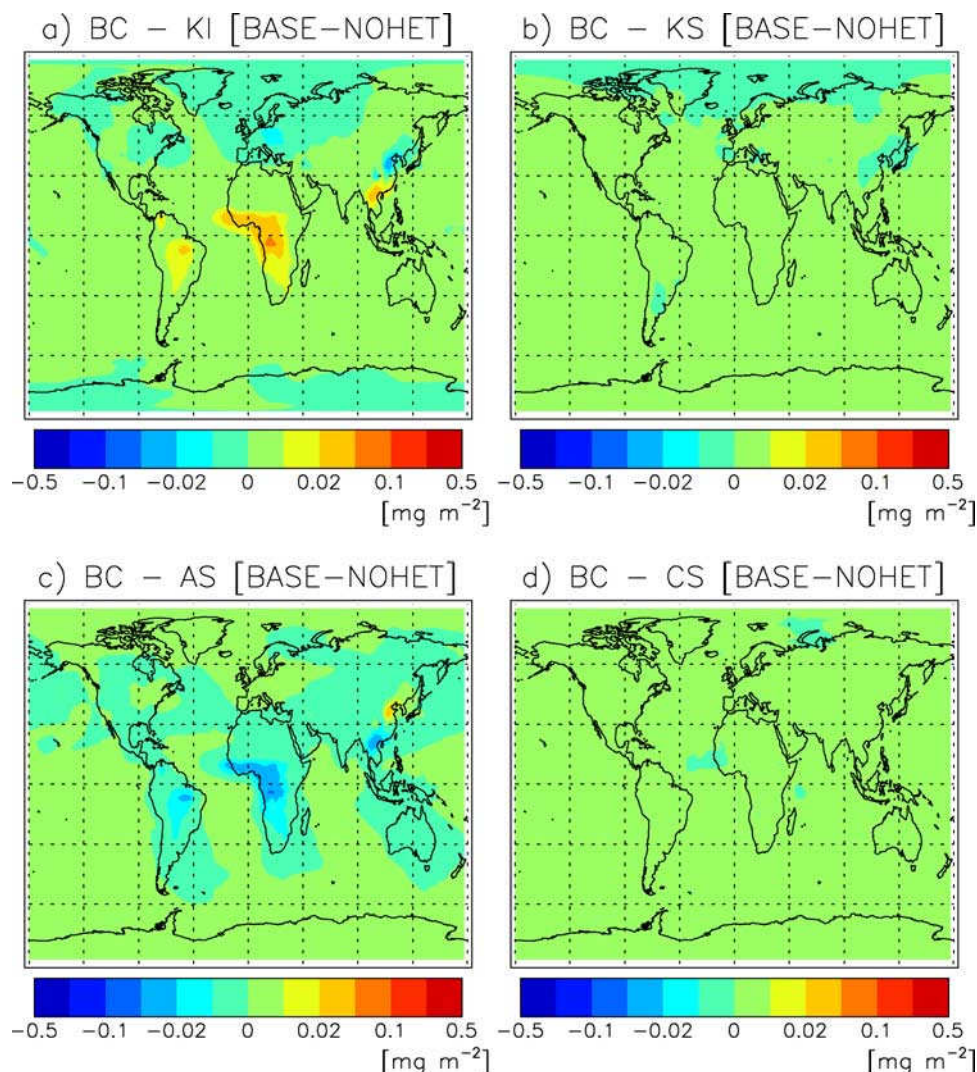
Figure 5. Annual mean burdens differences ( \text{mg}/\text{m}^2 ) between BASE and NOHET simulations of black carbon in the (a) Aitken hydrophobic (BC-KI) mode and in the (b) Aitken (BC-KS), (c) accumulation (BC-AS), and (d) coarse (BC-CS) hydrophilic modes.
