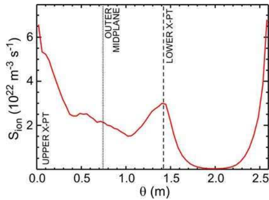
Figure 3: Calculated poloidal distribution of ionisation in the confined plasma (volume averaged) for 17469. The OSM-Eirene model is highly constrained by experimental data.
