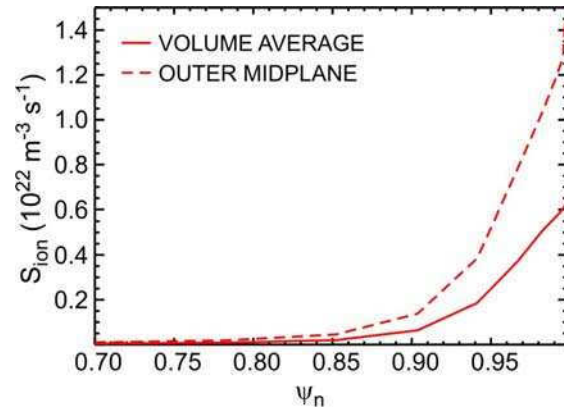
Figure 4: Radial distributions of ionisation in the confined plasma, with the volume averaged profile (solid) compared to the outer midplane profile (dashed).
