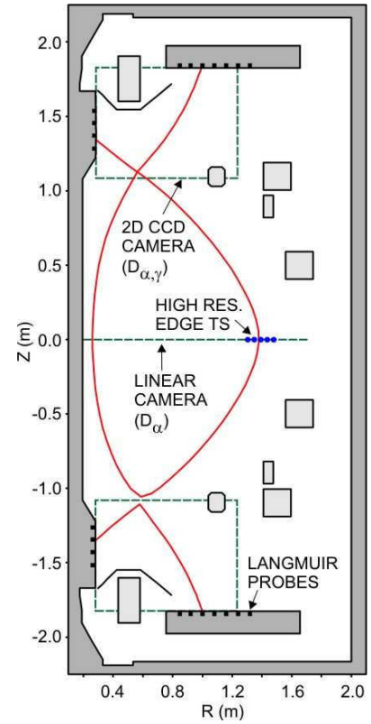
Figure 1: MAST poloidal cross section and relevant diagnostics. The separatrix location for 17469 at 259 ms is also shown.
