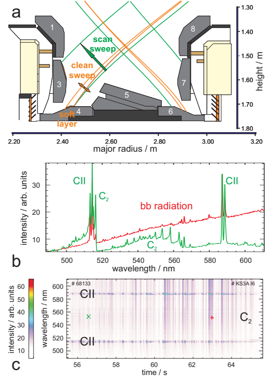
Figure 1: a) Magnetic configuration in the layer detection sweep and the cleaning discharge. b) C_2 and thermal emission induced by ELMs in a CLD. c) Time evolution of the optical emission spectrum (480nm-620nm) during a CLD.
