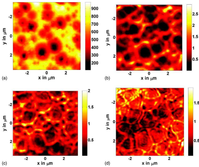
FIG. 1. (Color online) Measured topography in nanometer for a randomly textured surface of ZnO on top of a quartz substrate (a). The near-field intensity in arbitrary units slightly above this textured surface as measured with a scanning near-field optical microscope is shown for wavelengths of 780 nm (b), 658 nm (c), and 488 nm (d), respectively.
