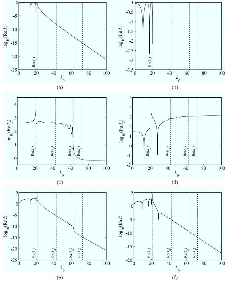
Figure 2. Real and imaginary parts of integrand components (a and b) I_1 and (c and d) I_2 and (e and f) full integrand I along the real k_\rho axis. The dashed lines correspond to the zeros of the vertical wavenumbers projected on the real axis.
