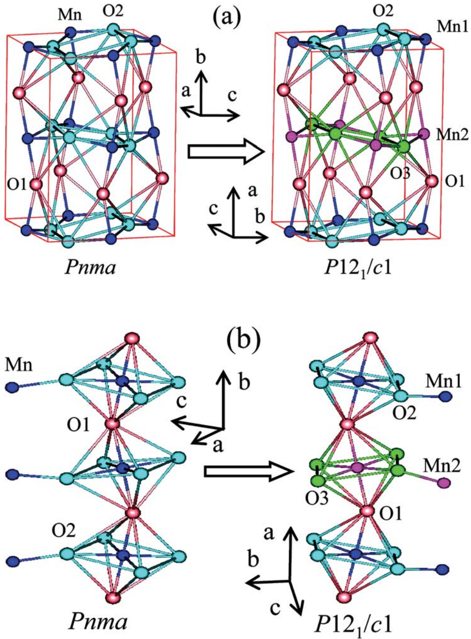
Figure 8.4: Schematic illustrations of (a) the crystal structure unit-cells and (b) the corresponding \text{MnO}_6 octahedra in orthorhombic ( Pnma ) and monoclinic ( P12_1/c1 ) models.
