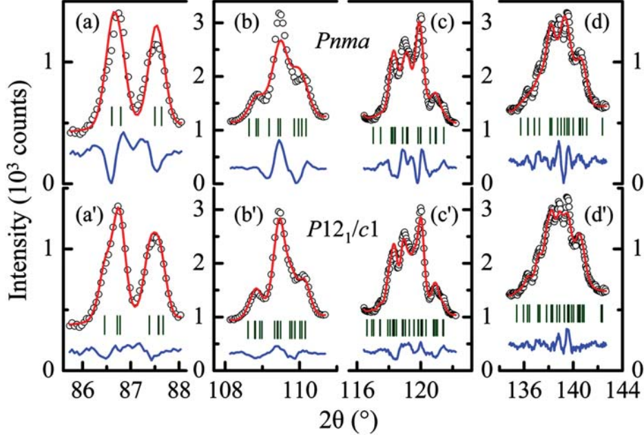
Figure 8.3: Observed NPD data (circles) of a powdered \text{La}_{1-x}\text{Sr}_x\text{MnO}_3 ( x \approx 1/8 ) single crystal within four 2\theta regions and the corresponding calculated intensities (solid lines) with space groups of Pnma (a, b, c and d) and P12_1/c1 (a', b', c' and d') at 220 K. The vertical lines mark the positions of Bragg reflections automatically generated from the space groups. The lower curve in each panel represents the difference between experimental and calculated patterns.
