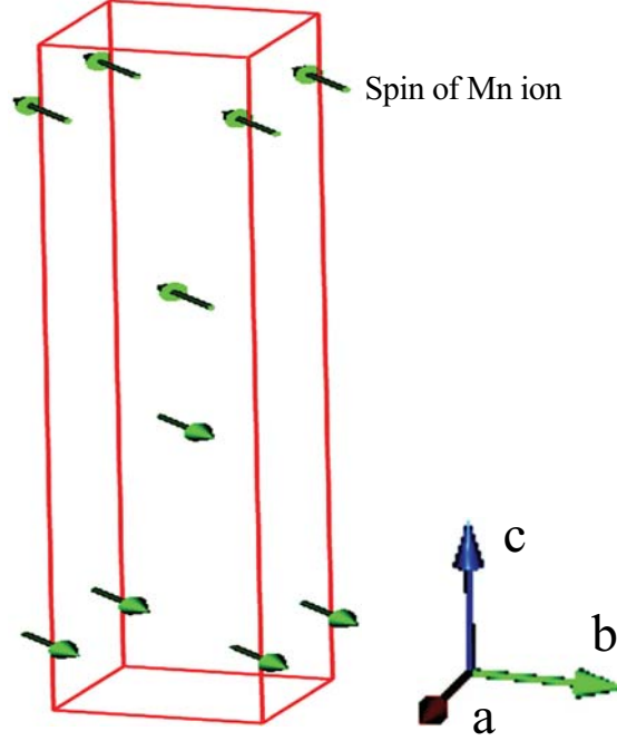
Figure 9.2: Arrangement of the A -AFM magnetic spins of Mn ions in \text{La}_1\text{Sr}_2\text{Mn}_2\text{O}_7 .
