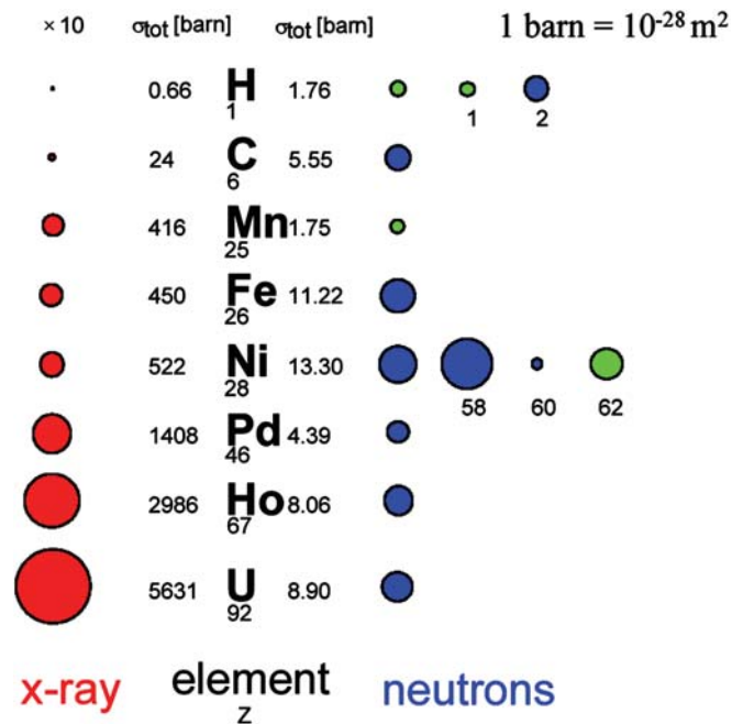
Figure 3.10 taken from [14]: Comparison of the coherent scattering cross-sections for x-rays and neutrons for a selection of elements. The area of the coloured circles represent the scattering cross section, where in the case of x-rays a scale factor 10 has to be applied. For neutrons, the green and blue coloured circles distinguish the cases where the scattering occurs with or without a phase shift of \pi .
