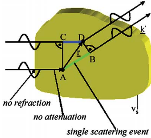
Figure 3.2: A sketch illustrating the phase difference between a beam scattered at the origin of the coordinate system and a beam scattered at the position \underline{r} taken from [14].
