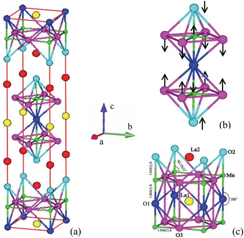
Figure 9.1: (a) Structural ( I4/mmm ; Z = 2 ) unit-cell of \text{La}_1\text{Sr}_2\text{Mn}_2\text{O}_7 at RT, where Mn: (0 0 z = 0.098(1) ), La1/Sr1: (0 0 \frac{1}{2} ), La2/Sr2: (0 0 z = 0.3161(7) ), O1: (0 0 0), O2: (0 0 z = 0.195(1) ) and O3: (0 \frac{1}{2} z = 0.0944(6) ). The structural parameters were taken from [198]. (b) \text{MnO}_6 octahedra along the c axis and the corresponding distortion mode. (c) Local environments for La1 and La2 sites.
