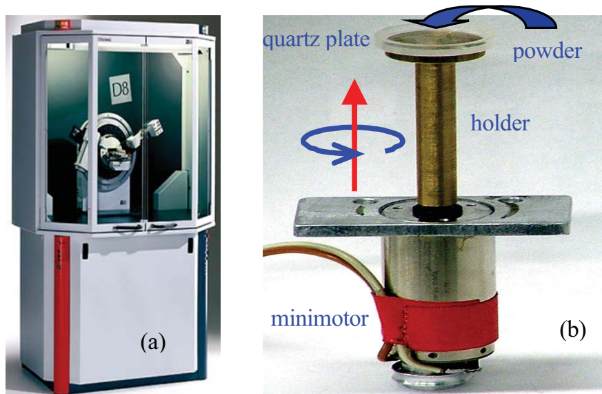
Figure 4.1: (a) Photograph of the BRUKER AXS D8 ADVANCE system used in this dissertation [126]. (b) The system of rotating specimen holder consists of a minimotor, a holder and a cavitary quartz plate.
