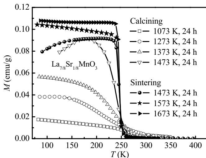
Figure 5.7: Zero-field cooling (ZFC) magnetization M measurements (10 Oe) for calcined and sintered \text{La}_{7/8}\text{Sr}_{1/8}\text{MnO}_3 at different temperatures for 24 h at each temperature.
