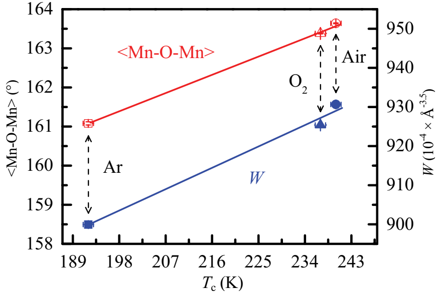
Figure 7.4: Mean Mn-O-Mn bond angle and one-electron bandwidth W of the e_g -band versus Curie temperature T_c for Ar, O 2 annealed and air sintered \text{La}_{0.875}\text{Sr}_{0.125}\text{Mn}_{1-\gamma}\text{O}_{3+\delta} samples. The solid lines are guides to the eye.
