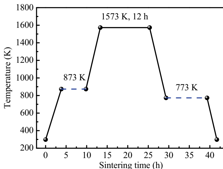
Figure 5.2: Schematic of the heating-cooling process of sintering.
