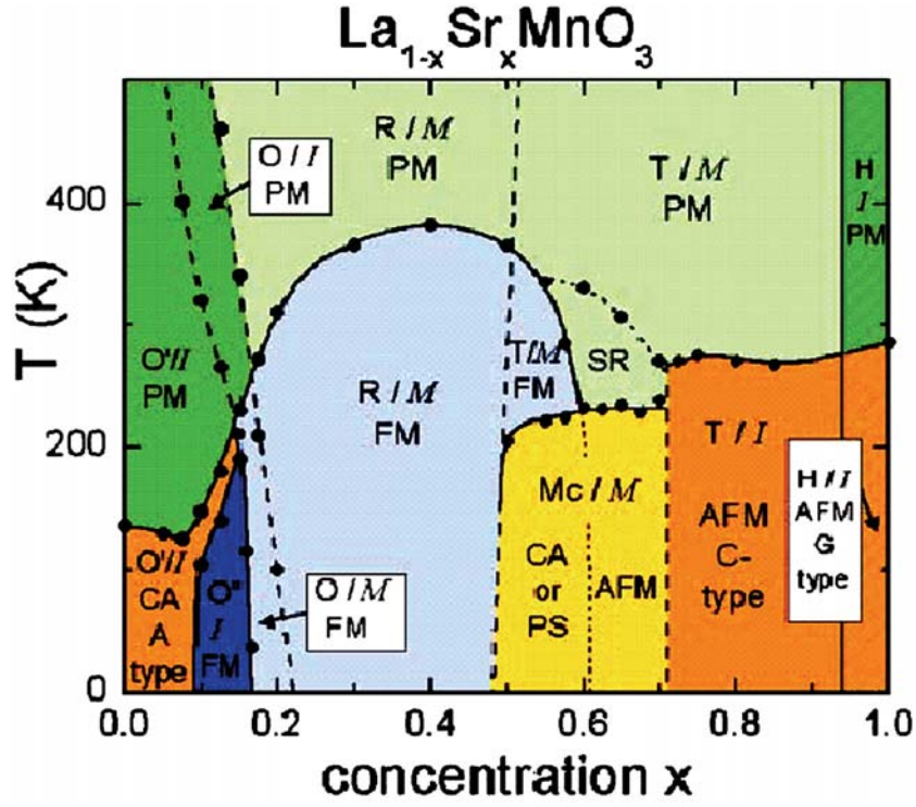
Figure 7.1: Proposed phase diagram for \text{La}_{1-x}\text{Sr}_x\text{MnO}_3 manganites [7]. R, O, T, H label the crystallographic phases rhombohedral, orthorhombic, tetragonal and hexagonal. M stands for metal, I for insulator. Magnetic order is indicated by PM, FM, AFM, CA or PS for paramagnetic, ferromagnetic, antiferromagnetic, canted or phase separated, respectively.
