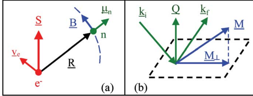
Figure 3.7: (a) Geometry for the derivation of the interaction between neutron and electron. (b) Scattering geometry for the magnetic neutron scattering, only the component \underline{M}_\perp of the magnetization \underline{M} perpendicular to the scattering vector \underline{Q} is of relevance.
