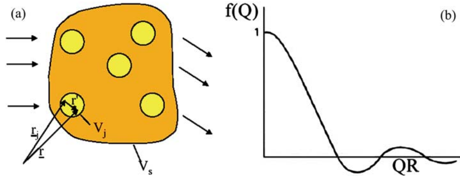
Figure 3.3 taken from [14]: (a) Sketch showing the assembly of N scatterers of finite size and defining the quantities needed for the introduction of the form factor. (b) Form-factor for a homogeneous sphere according to equation 3.15.
