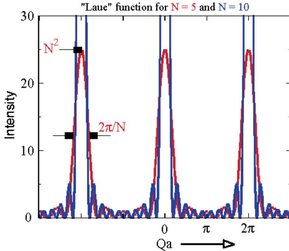
Figure 3.4 taken from [14]: Laue function along the lattice direction \underline{a} for a lattice with five and ten periods, respectively.
