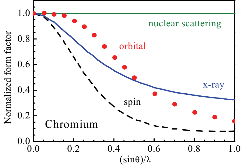
Figure 3.8: Nuclear scattering power, atomic form factor (x-ray) and magnetic form factor (spin and orbital) of Cr (see text) [116, 117].
