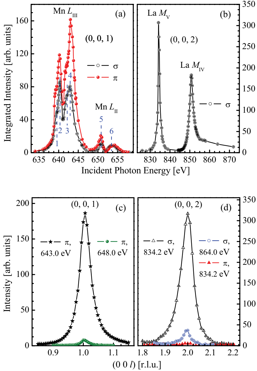
Figure 9.4: (a) Energy dependence of A -AFM (0, 0, 1) reflection in \text{La}_1\text{Sr}_2\text{Mn}_2\text{O}_7 recorded over the \text{Mn } L_{\text{II, III}} -edges and (b) Bragg (0, 0, 2) reflection over the \text{La } M_{\text{IV, V}} -edges with incident linear \sigma and \pi polarizations at 15 K. The intensity was integrated from the longitudinal scan. (c) and (d) Corresponding longitudinal scans of two reflections at and off their strongest resonance energies \sim 643.0 eV ( \text{Mn } L_{\text{III}} -edge) and \sim 834.2 eV ( \text{La } M_{\text{V}} -edge).
