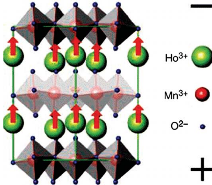
Figure 2.3: Hexagonal \text{HoMnO}_3 is ferroelectric, because the oxygen bipyramids surrounding each \text{Mn}^{3+} ion are tilted and shifted relative to the \text{Ho}^{3+} ions. It is also magnetic, with ferromagnetic alignment of the \text{Ho}^{3+} magnetic moments combined with antiferromagnetic \text{Mn}^{3+} ordering. Therefore, hexagonal \text{HoMnO}_3 is multiferroic [44].
