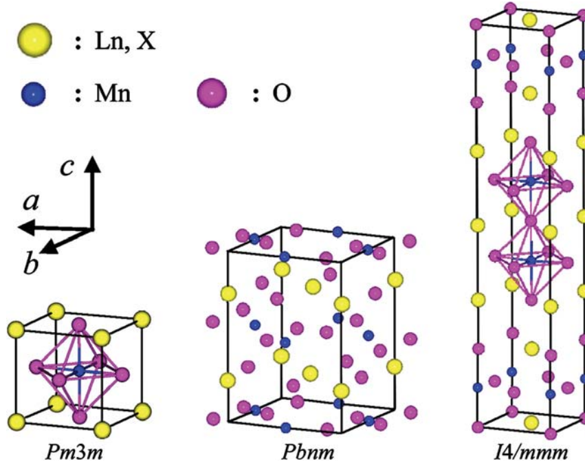
Figure 2.6: Unit cells of ideal cubic perovskite structure (left), distorted orthorhombic structure in most (\text{Ln}_{1-x}\text{X}_x)\text{MnO}_3 (middle) and distorted tetragonal structure in most (\text{Ln}_{1-x}\text{X}_x)_3\text{Mn}_2\text{O}_7 (right).
