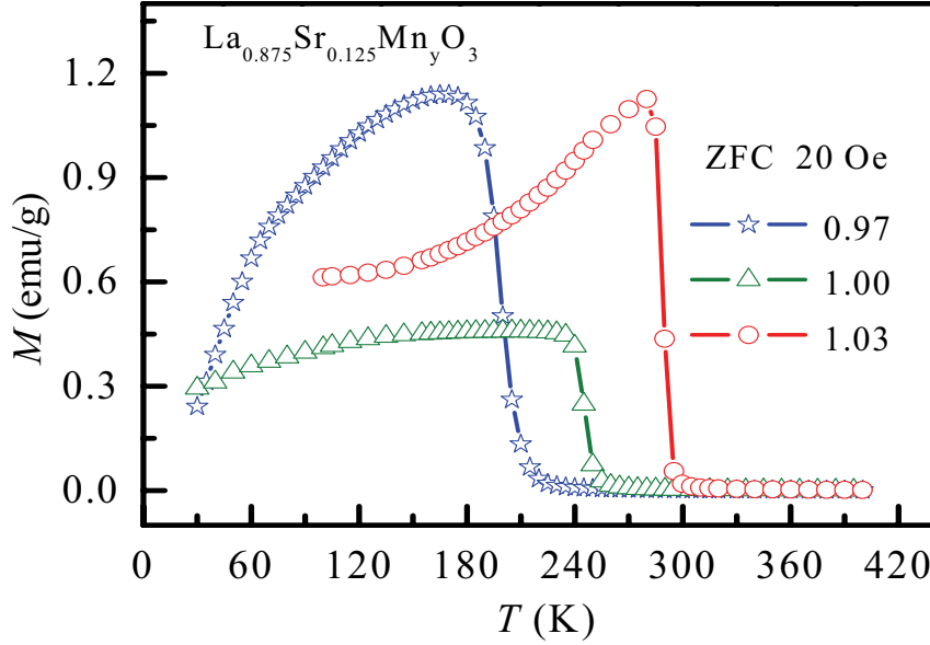
Figure 7.6: ZFC magnetization M versus temperature measured at H = 20 Oe for the three air sintered \text{La}_{0.875}\text{Sr}_{0.125}\text{Mn}_y\text{O}_3 samples with initial y = 0.97, 1.00 and 1.03 , belonging to the rhombohedral structure at room temperature. The solid lines are guides to the eye.
