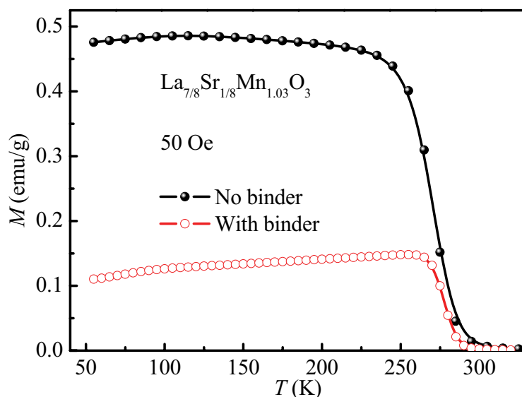
Figure 5.9: ZFC magnetization M measurements of two sintered \text{La}_{7/8}\text{Sr}_{1/8}\text{Mn}_{1.03}\text{O}_3 polycrystals. In the processes: with (circles) and without (solid circles) binder.
