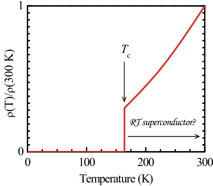
Figure 2.1: The electrical resistivity of a superconductor decreases to zero sharply at the Curie temperature T_c , entering into the superconducting state. The room-temperature (RT) superconductor has not been found yet.
