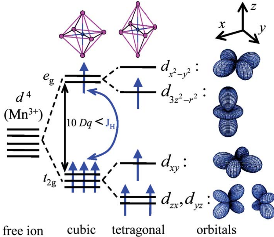
Figure 2.8: Crystal field splitting of fivefold degenerate d orbitals of 3d^4 free ions ( \text{Mn}^{3+} ) in octahedral geometry as well as the corresponding approximate orbital shapes in real space. Since the crystal field splitting ( 10 Dq \sim 1 eV [67, 68]) is smaller than the Hund's coupling ( J_H \sim 2-3 eV [69, 70]), the e_g spin is aligned to the t_{2g} spins, realizing a high-spin state.
