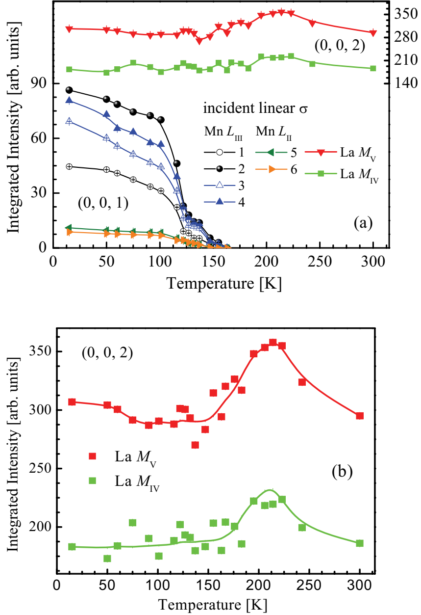
Figure 9.5: (a) Temperature dependent integrated intensity (measured in the longitudinal direction) of A -AFM (0\ 0\ 1) reflection in \text{La}_1\text{Sr}_2\text{Mn}_2\text{O}_7 recorded at six energies corresponding to the six clear features 1, 2, 3, 4, 5 and 6 as labeled in the energy spectra in figure 9.4(a), and (0\ 0\ 2) reflection at the \text{La } M_{IV, V} -edges. (b) Magnified temperature dependence of Bragg (0\ 0\ 2) reflection.
