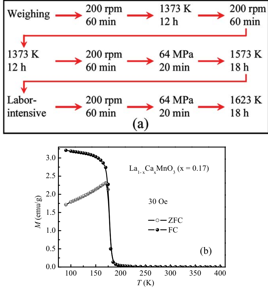
Figure 5.12: (a) Processing parameters for \text{La}_{0.83}\text{Ca}_{0.17}\text{MnO}_3 . (b) ZFC cooling and field cooling (FC) magnetization M measurements for \text{La}_{0.83}\text{Ca}_{0.17}\text{MnO}_3 .
