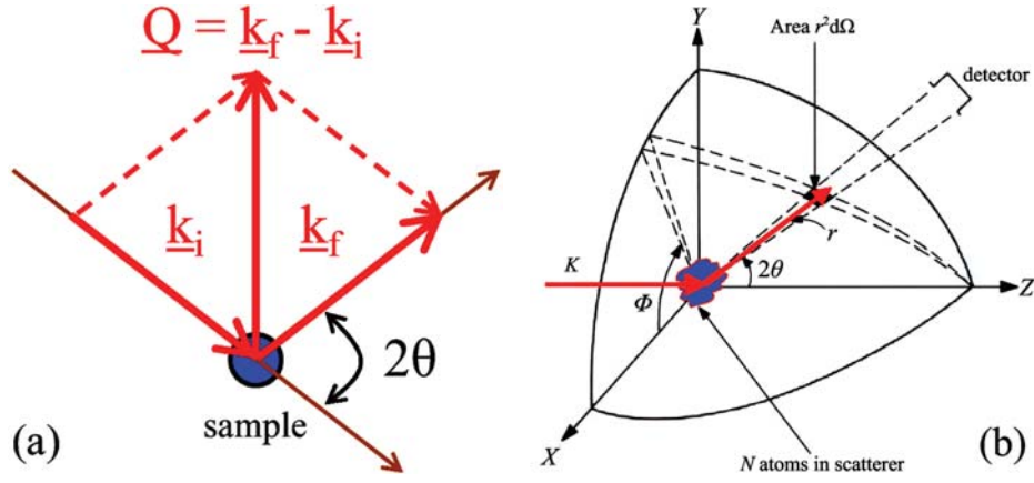
Figure 3.1: (a) A sketch of the scattering process in the Fraunhofer approximation in which the sample is viewed as a ‘point’ object due to the fact that the distance source-sample and sample-detector, respectively, is significantly larger than the size of the sample. (b) Geometry used for the definition of the scattering cross section taken from [14].
