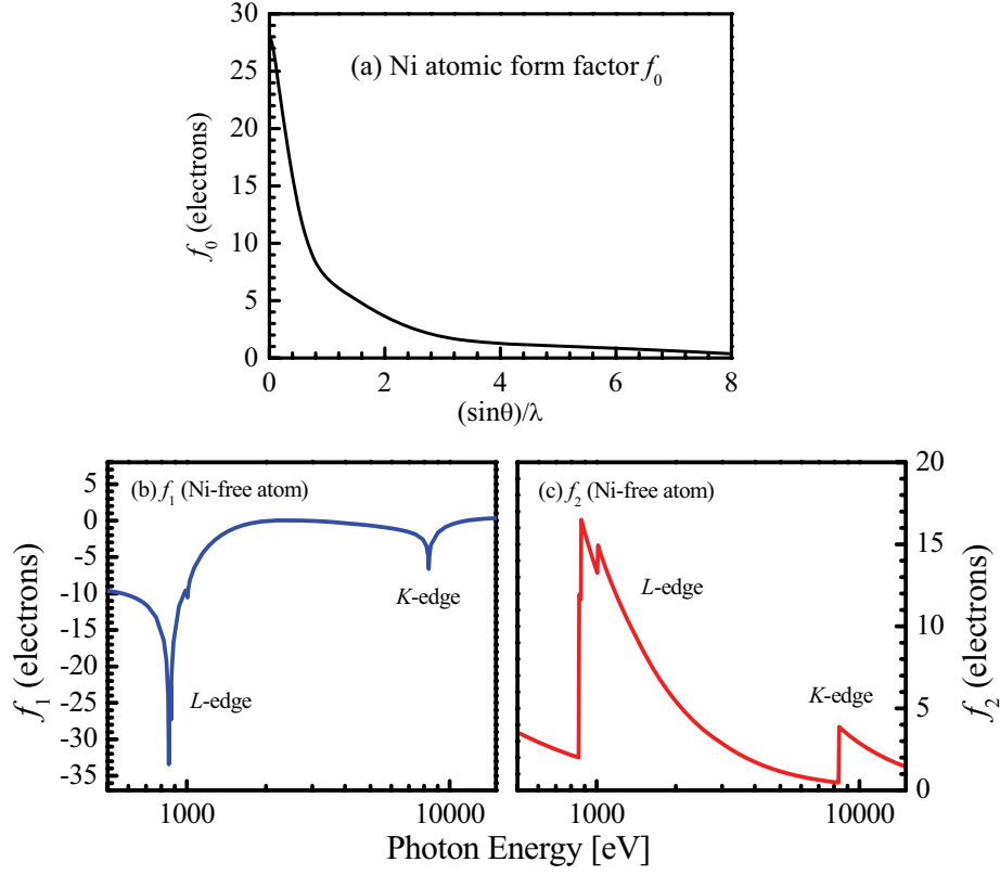
Figure 3.6: (a) X-ray atomic form factor of Ni. (b) and (c) The real ( f_1 ) and imaginary ( f_2 ) components of the anomalous atomic scattering factor of Ni for the free atom [115].
