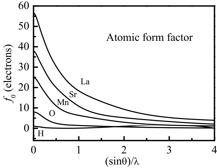
Figure 3.5: X-ray atomic form factors of La, Sr, Mn, O and H as a function of (\sin\theta)/\lambda plotted in order from the top to the bottom.
