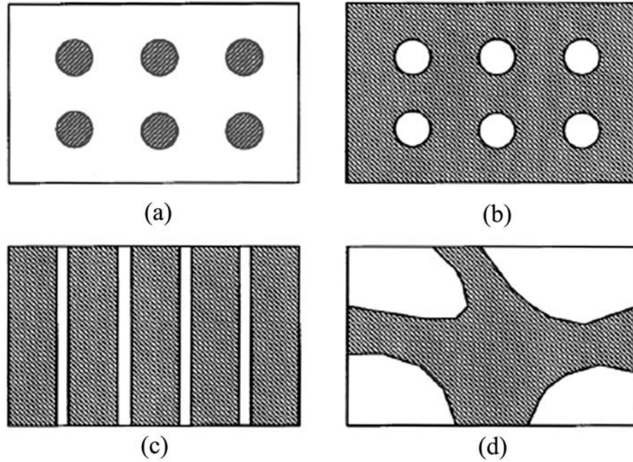
Figure 2.14: Schematic of the electronic phase separation [110]. Shaded portions indicate FM metallic regions; the unshaded portions correspond to AFM insulating regions. (a) FM metallic puddles in an insulating AFM background. (b) Metallic regions with insulating droplets. (c) Charged stripes. (d) Phase separation on the mesoscopic scale.
