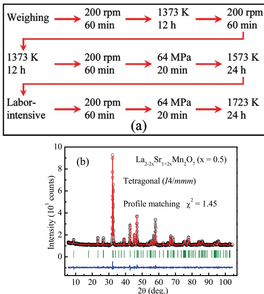
Figure 5.11: (a) Processing parameters for \text{La}_1\text{Sr}_2\text{Mn}_2\text{O}_7 . (b) Profile matching of the XRPD data of \text{La}_1\text{Sr}_2\text{Mn}_2\text{O}_7 at room temperature shows no appearance of impurity phases within the detection accuracy.
