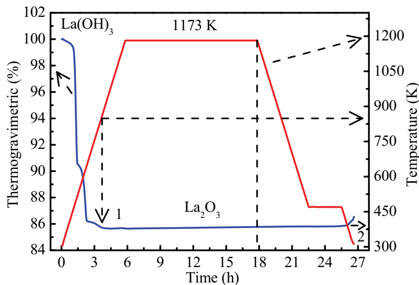
Figure 5.4: Thermogravimetric analysis of \text{La}(\text{OH})_3 transformed from \text{La}_2\text{O}_3 through the ~2 h exposure to air.
