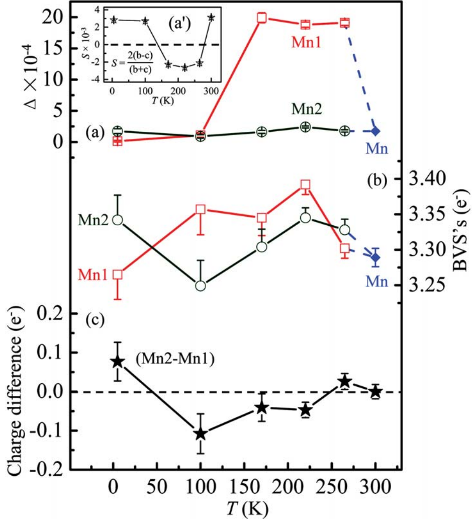
Figure 8.7: Temperature variations of (a) the size of cooperative JT distortion of \text{MnO}_6 octahedra \Delta (defined in equation 7.1), (b) the BVS's of the Mn ( Pnma ) and Mn1, Mn2 ( P12_1/c1 ) calculated from the refined parameters and (c) the charge difference between Mn1 and Mn2. Inset (a') shows the orthorhombic strain in the b - c plane, namely S = 2(b-c)/(b+c) , in P12_1/c1 symmetry.
