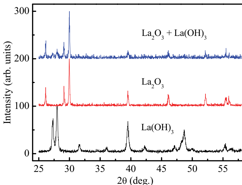
Figure 5.3: XRPD patterns of (top) \text{La}_2\text{O}_3 normally stored in a plastic bottle in air; (middle) just dried \text{La}_2\text{O}_3 at 1173 K for 12 h; (bottom) after ~2 h exposure of dried \text{La}_2\text{O}_3 to air.
