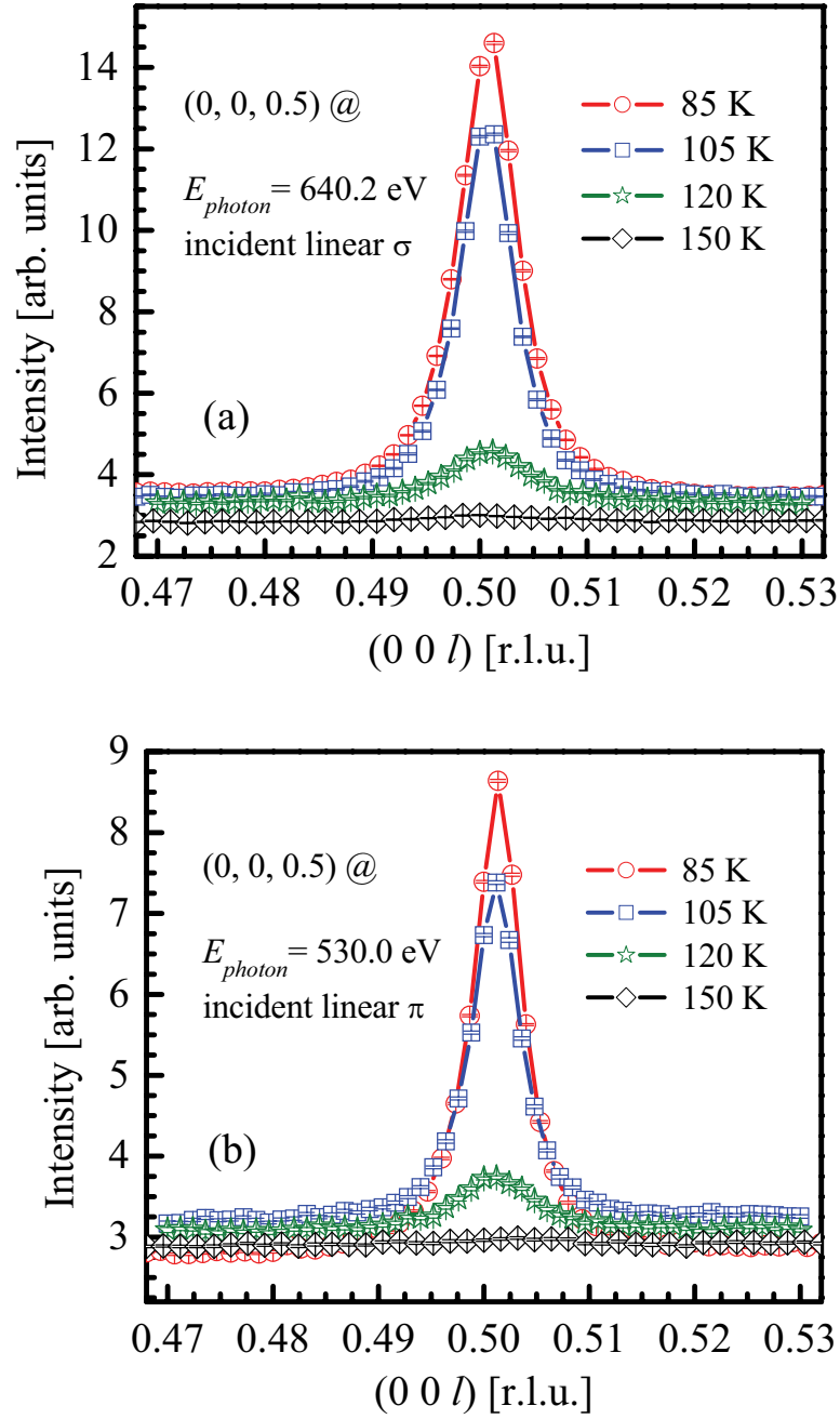
Figure 8.13: Temperature dependence of the CO reflection (0, 0, \frac{1}{2}) in Pbnm symmetry in \text{La}_{1-x}\text{Sr}_x\text{MnO}_3 ( x \approx 1/8 ) at: (a) 640.2 eV (Mn L_{\text{III}} -edge) with incident \sigma polarization and (b) 530.0 eV (oxygen K -edge) with incident \pi polarization.
