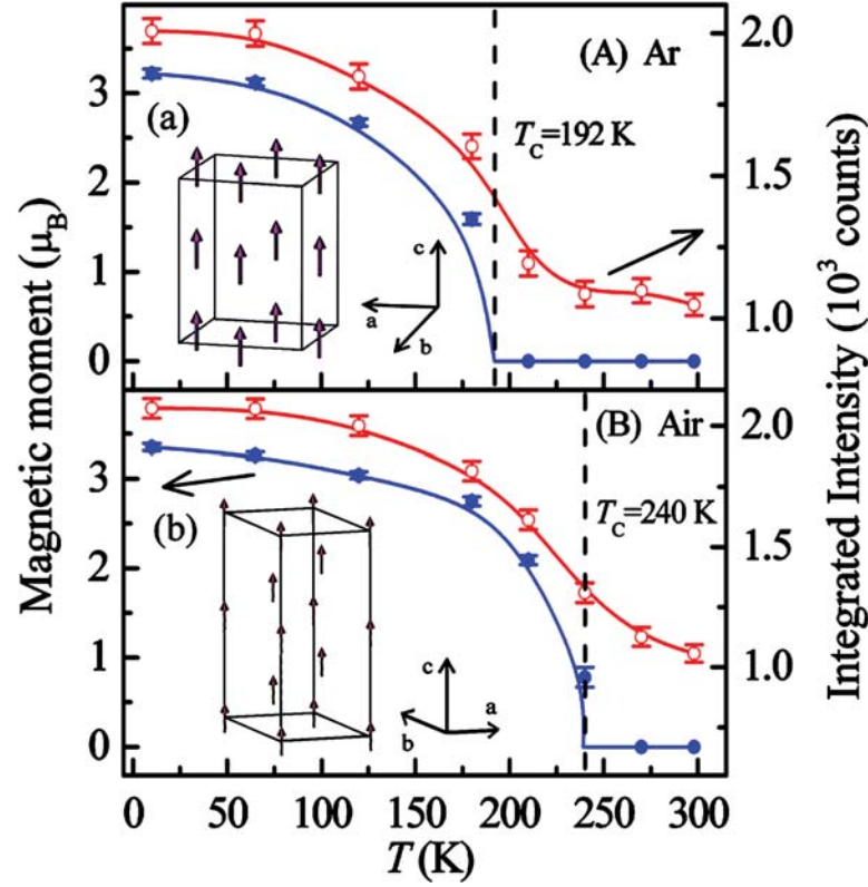
Figure 7.10: Refined Mn moment (left) and integrated intensity (right) observed at Q = (1\ 1\ 0) and (0\ 0\ 2) of the O structure and Q = (0\ 1\ 2) of the R (hexagonal setting) structure versus temperature for (A) the Ar annealed and (B) the air sintered \text{La}_{0.875}\text{Sr}_{0.125}\text{Mn}_{1-\gamma}\text{O}_{3+\delta} samples. Insets (a) and (b) show schematic illustrations of the ordered moments in the FM space groups of Pb'n'm and P1 , respectively. T_c is the onset temperature of FM ordering based on SQUID measurements. The solid lines are guides to the eye.
