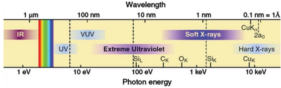
Figure 3.11: The short wavelength region of the electromagnetic spectrum taken from [122]. The oxygen K -edge ( 1s \rightarrow 2p ), the transition-metal L_{II,III} -edges ( 2p \rightarrow 3d ) and the rare-earth M_{IV,V} -edges ( 3d \rightarrow 4f ), are located in the soft x-ray spectral region.
