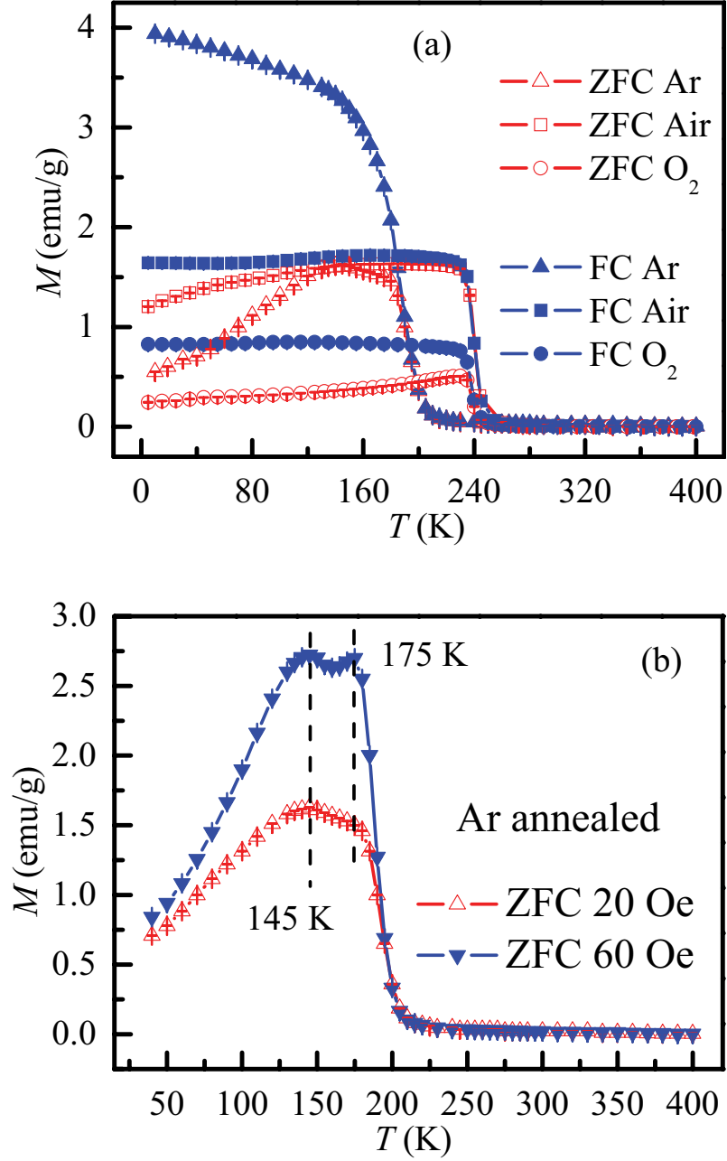
Figure 7.3: (a) ZFC and FC magnetization M versus temperature measured at H = 20 Oe for three \text{La}_{0.875}\text{Sr}_{0.125}\text{Mn}_{1-\gamma}\text{O}_{3+\delta} samples and (b) ZFC M at 20 and 60 Oe for the Ar annealed sample. The lines are guides to the eye.
