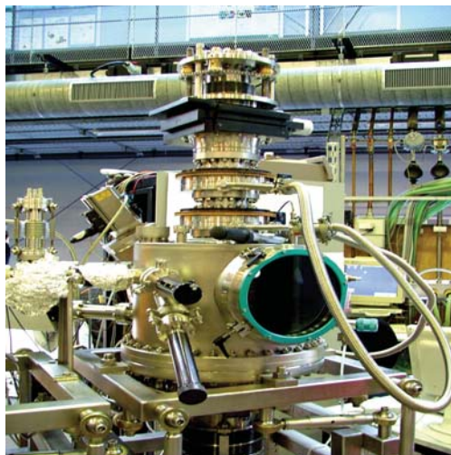
Figure 4.3: The soft x-ray scattering UHV chamber ALICE designed and built in horizontal scattering geometry by Bochum University, Germany, and installed at BESSY II.
