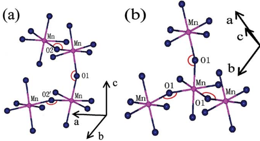
Figure 7.9: Schematic illustration of (a) Mn-O1-Mn, Mn-O2-Mn and Mn-O2'-Mn (= Mn-O2-Mn) bond angles in the O structure of the Ar annealed sample at 180 K and (b) Mn-O1-Mn in the R (hexagonal setting) structure of the air sintered sample at 180 K.
