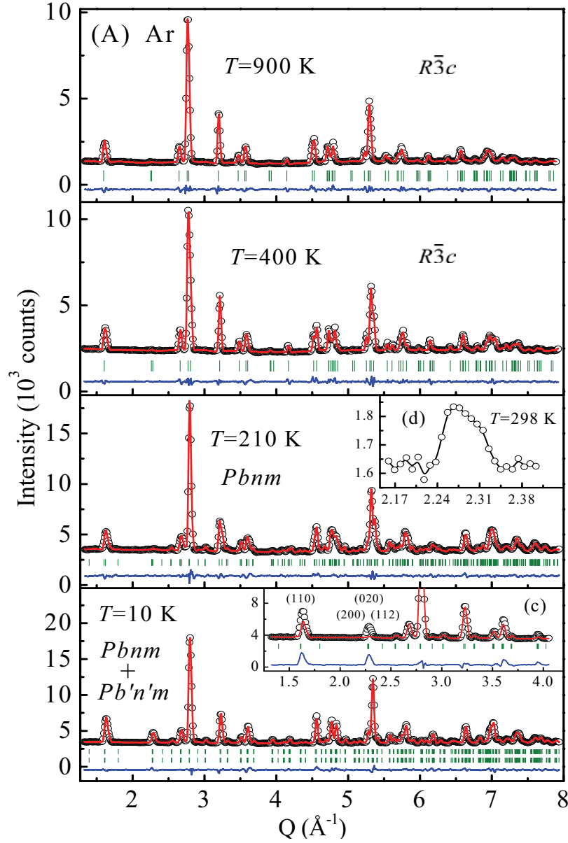
Figure 7.7: Observed (circles) and calculated (solid lines) NPD patterns of (A) the Ar annealed ( T=10, 210, 400 and 900 K) and (B) the air sintered ( T=10, 120, 180 and 270 K) \text{La}_{0.875}\text{Sr}_{0.125}\text{Mn}_{1+\gamma}\text{O}_{3+\delta} samples. The vertical bars mark the Bragg (top) and magnetic (bottom) peak positions automatically generated from the space group. The line in the bottom of each diagram is the difference between the observed and calculated patterns. Inset (a) shows five observed patterns of air sintered sample in certain Q regions for the temperatures of 10, 65, 120, 180 and 270 K, respectively (to be continued).
