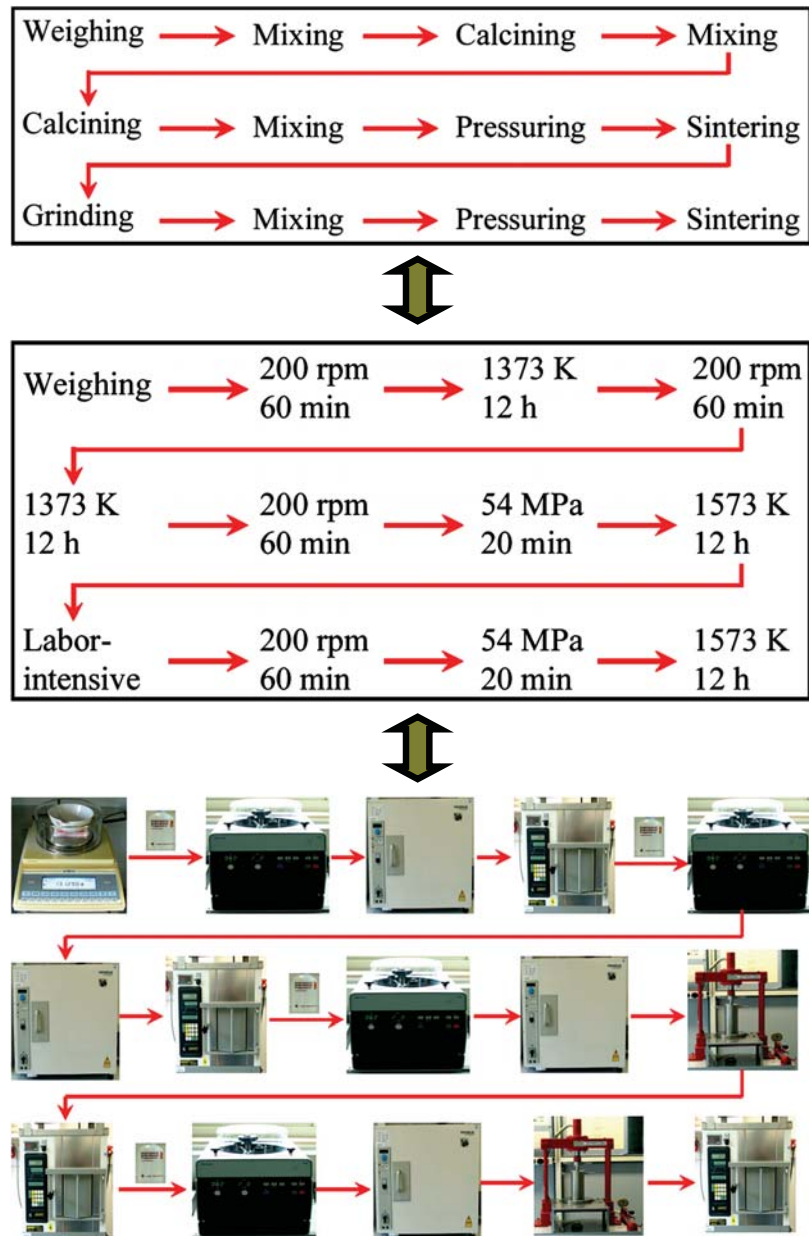
Figure 5.10: (top) Optimum processing route for the synthesis of \text{La}_{7/8}\text{Sr}_{1/8}\text{MnO}_3 . (middle) Corresponding processing parameters. (bottom) Corresponding apparatuses used in the laboratory for the preparation of electroceramic materials at FZJ GmbH, Germany.
