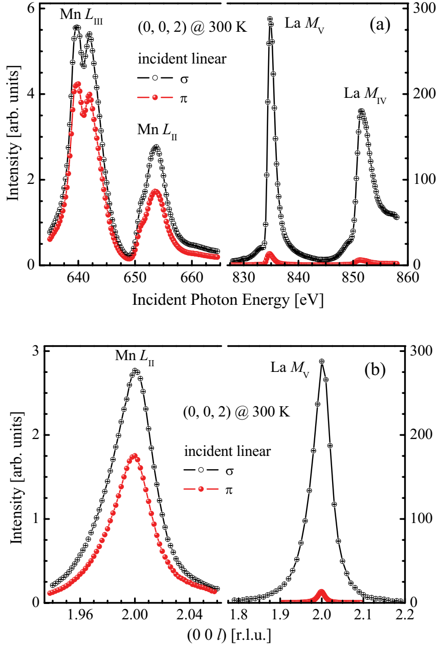
Figure 9.3: (a) Energy dependence of Bragg (0 0 2) reflection in \text{La}_1\text{Sr}_2\text{Mn}_2\text{O}_7 recorded over the \text{Mn } L_{\text{II,III}} - and the \text{La } M_{\text{IV,V}} - edges at constant wave vector with incident linear \sigma and \pi polarizations at 300 K. (b) Corresponding longitudinal scans at the \text{Mn } L_{\text{II}} - and the \text{La } M_{\text{V}} -edges.
