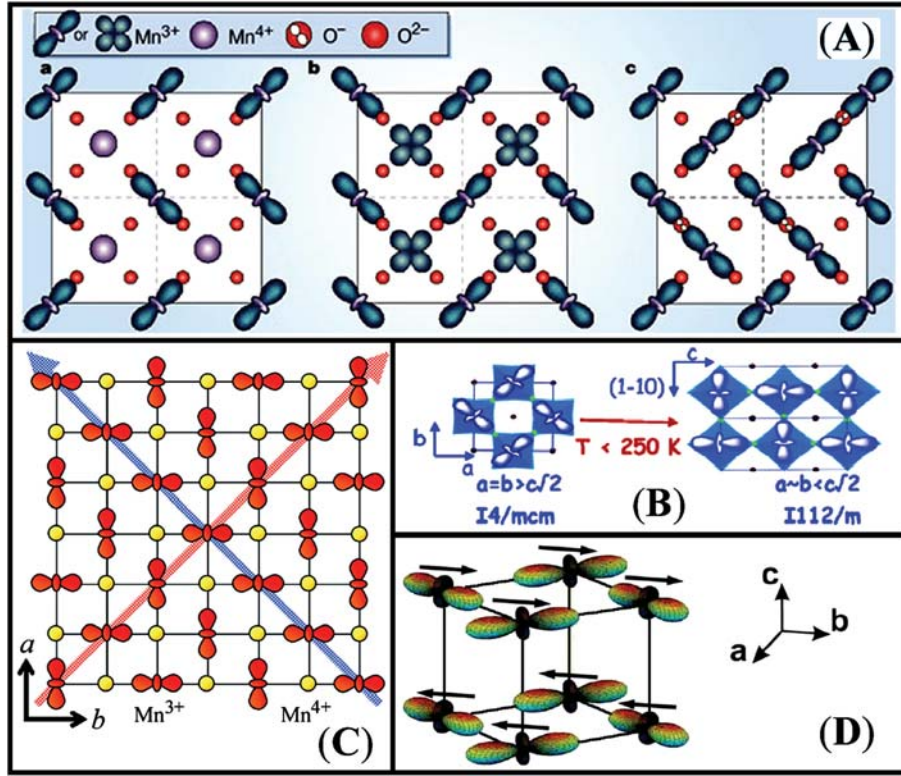
Figure 2.12: (A) \text{La}_{0.5}\text{Ca}_{0.5}\text{MnO}_3 : the checkerboard charge order originally proposed by Goodenough [77] for \text{Mn}^{3+} and \text{Mn}^{4+} ions (a), in which the oxygen 2p shells are fully filled; CE-type orbital order for two distinct \text{Mn}^{3+} sublattices [101], one of which corresponds to 3d_{3x^2-r^2}/3y^2-r^2 orbitals and another to the 3d_{x^2-y^2} orbital (b). This pattern implies that there is incomplete occupancy of the oxygen 2p shell; the ordered arrangement of \text{O}^- ions between \text{Mn}^{3+} pairs in the Zener polaron model (c), suggesting the invalidation of the traditional \text{Mn}^{3+}/\text{Mn}^{4+} CO pattern [16, 102, 103]. Three patterns are projected on the \text{MnO}_2 sheet ( a - b plane). (B) \text{KCrF}_3 : 3d_{z^2} OO schemes in different structures [104]. (C) \text{Pr}_{0.5}\text{Ca}_{0.5}\text{MnO}_3 : orbital order 3d_{3x^2-r^2}/3y^2-r^2 and charge order of the CE type projected on the \text{MnO}_2 sheet ( a - b plane) [71]. (D) \text{LaMnO}_3 : orbital order 3d_{3x^2-r^2}/3y^2-r^2 and A-type AFM spin order [105].
