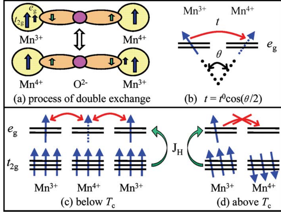
Figure 2.9: Illustration of the double exchange mechanism for Mn ions with different valencies ( \text{Mn}^{3+} and \text{Mn}^{4+} ). Here t is the hopping parameter of the e_g electron and J_H is the FM Hund's coupling between e_g and t_{2g} electrons.
