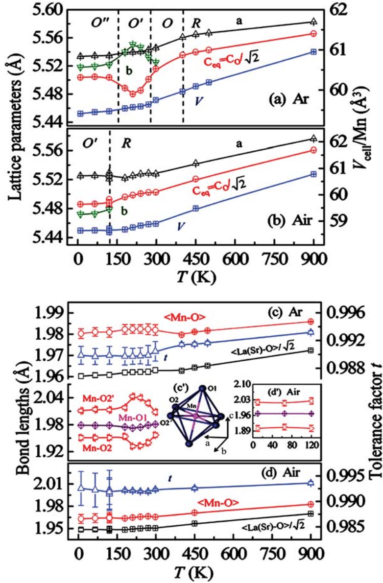
Figure 7.8: (a, b): refined lattice parameters (left) and unit-cell volume V per Mn ion (right) versus temperature for (a) the Ar annealed and (b) the air sintered \text{La}_{0.875}\text{Sr}_{0.125}\text{Mn}_{1-\gamma}\text{O}_{3+\delta} samples. The equivalent lattice parameter c_{\text{eq}} for the O and R (hexagonal setting) structures is obtained by c_{\text{eq}} = c_o / \sqrt{2} ( O structure: c_o = c_o and R structure: a_h = (a_o - b_o - c_o)/2 , b_h = b_o , c_h = 2a_o + c_o and c_o = c_o , so 9c_o \cdot c_o = c_h \cdot c_h + 12a_h \cdot a_h . Ital. subscripts h and o stand for hexagonal and orthorhombic, respectively). (c, d): mean Mn-O and La(Sr)-O/ \sqrt{2} bond lengths (left) and tolerance factor t (right) versus temperature for (c) the Ar annealed and (d) the air sintered samples (to be continued).
