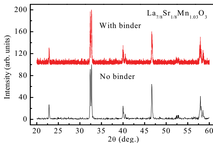
Figure 5.8: XRPD patterns of two sintered \text{La}_{7/8}\text{Sr}_{1/8}\text{Mn}_{1.03}\text{O}_3 polycrystals. In the processes: with (top) and without (bottom) binder.
