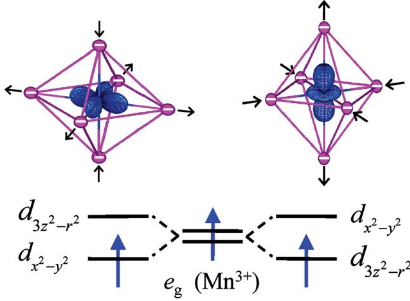
Figure 2.7: Effect of the JT distortion on the electronic structure of \text{Mn}^{3+} e_g states.
