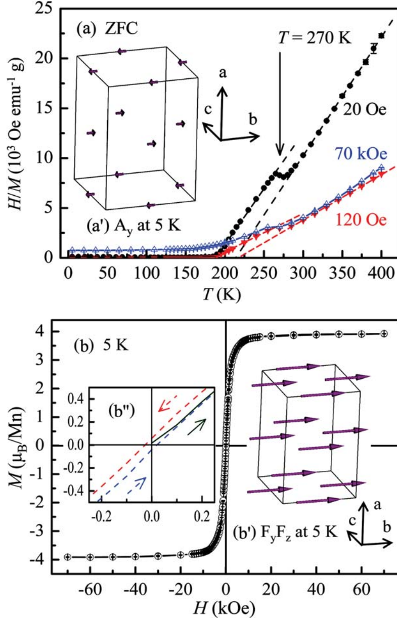
Figure 8.9: (a) Temperature variation of the ZFC H/M at 20, 120 and 7 \times 10^4 Oe with the dashed lines showing the fits of the data at 20 and 120 Oe to the Curie-Weiss law below and above T_{JT} . (b) A hysteresis loop at 5 K. Insets (a') and (b') illustrate the magnetic structure unit-cells A_y and F_y F_z at 5 K in P12_1/c1 symmetry, respectively. Inset (b'') depicts the enlarged view of the hysteresis loop in a limited region. A_y , F_y and F_z denote the A -AFM moment along the b axis and the FM moments along the b and c axes, respectively.
