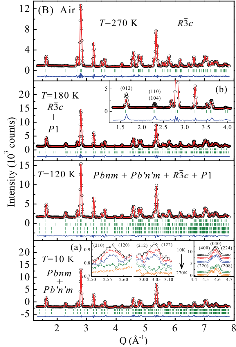
Figure 7.7 (continued): For clarity, the patterns were shifted along the intensity axis with the highest corresponding to the lowest temperature. Insets (b) and (c) show the calculation of the scattering from the nuclear structure only for the air sintered ( T = 180 K) and Ar annealed ( T = 10 K) samples, respectively, indicating the major magnetic diffraction peaks. Inset (d) shows the existence of the Bragg peaks indexed as (2 0 0), (0 2 0) and (1 1 2) in the Pbnm symmetry at 298 K for the Ar annealed sample. For the air sintered sample, a coexistence of magnetically ordered O with magnetically ordered R structures occurs.
