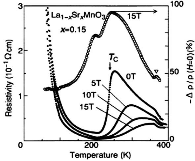
Figure 2.2: Temperature dependence of resistivity for \text{La}_{1-x}\text{Sr}_x\text{MnO}_3 ( x = 0.15 ) under various magnetic fields. Open circles represent the magnitude of negative magnetoresistance -\Delta\rho/\rho(T, 0) with a magnetic field of 15 T [38].
