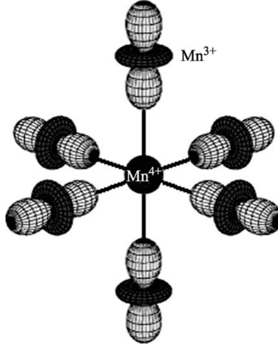
Figure 8.2: The orbitals of \text{Mn}^{3+} ions are directed towards a hole forming an orbital polaron around a \text{Mn}^{4+} site (sphere). The formation of an orbital polaron not only leads to a FM object that is stabilized by the double-exchange mechanism, but also traps a hole reducing the kinetic energy of the charge carriers, which consequently could lead to the FMI state. Taken from [9].
