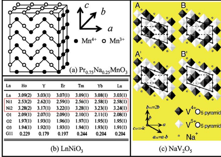
Figure 2.11: (a) Charge-ordered states in \text{Pr}_{0.75}\text{Na}_{0.25}\text{MnO}_3 below 220 K, where the \text{Mn}^{3+} and \text{Mn}^{4+} cations form zigzag chains in crystallographic a - c plane [82]. (b) Valencies determined from the bond valence model for Ln, Ni, and O within the \text{LnO}_8 and \text{NiO}_6 coordination polyhedra in \text{LnNiO}_3 [83]. (c) Zigzag-type charge-order pattern with respect to the configuration of \text{V}^{4+}\text{O}_5 (black) and \text{V}^{5+}\text{O}_5 (white) pyramids lying in the a - b plane [84, 85]. There are four types of possible in-plane configuration denoted as A, A', B and B'. Dotted and solid lines represent crystallographic unit cells: orthorhombic ( a \times b \times c ) above T_c = 35 K and monoclinic ( a_m \times b_m \times c_m ) below T_c [86].
