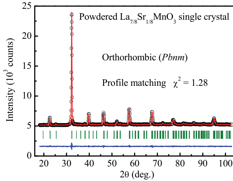
Figure 6.7: Profile matching of the XRPD data of a powdered \text{La}_{7/8}\text{Sr}_{1/8}\text{MnO}_3 single crystal at room temperature shows no appearance of impurity phase within the detection accuracy.
