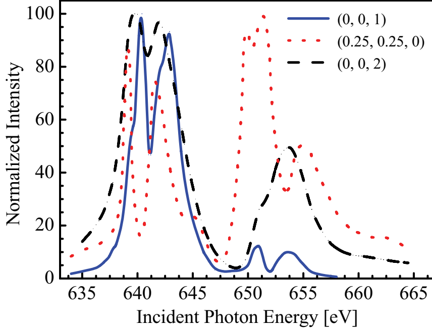
Figure 9.6: Comparison between three resonant energy spectra through the Mn L_{II,III} -edges for \text{La}_1\text{Sr}_2\text{Mn}_2\text{O}_7 : A -AFM (0 0 1) reflection at 15 K; OO (0.25 0.25 0) reflection at \sim 20 K [203]; Bragg (0 0 2) reflection at 300 K. Incident photon energy of (0.25 0.25 0) was calibrated by the difference between energy dependent intensity of (0 0 1) in [203] and the corresponding one observed here. Observed intensity was normalized to 100.
