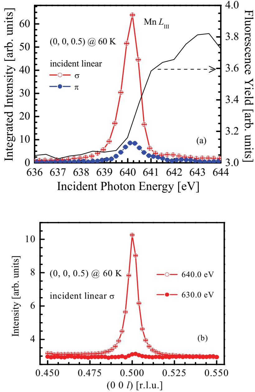
Figure 8.11: (a) A significant resonant enhancement of the CO reflection (0\ 0\ 1/2) in Pbnm symmetry in \text{La}_{1-x}\text{Sr}_x\text{MnO}_3 ( x \approx 1/8 ) is clearly seen at the Mn L_{\text{III}} -edge at 60 K. (b) Longitudinal scans of (0\ 0\ 1/2) in Pbnm symmetry at different incident photon energies with incident \sigma polarization at 60 K.
