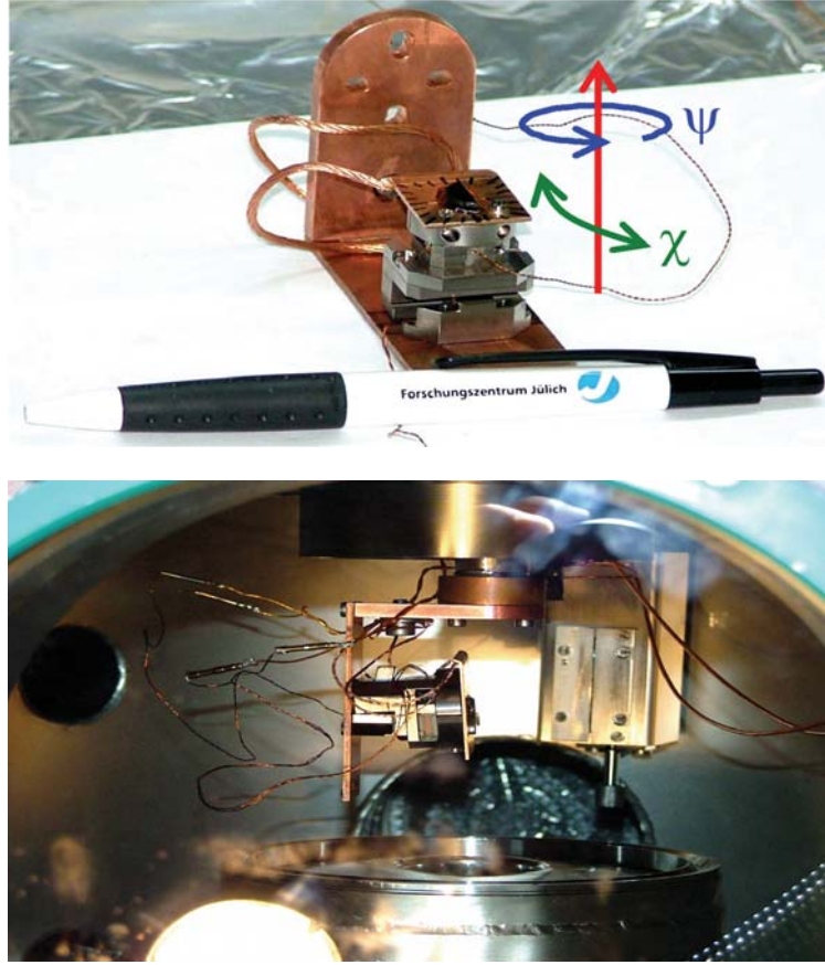
Figure 4.4: (top) The miniature goniometer for sample rotation and tilt in the \psi and \chi angles, respectively. (bottom) View into the heart of ALICE chamber through the load-lock window. The x-rays enter from the left window, through a set of slits, and then scatter off the sample (mounted on our goniometer, \theta shown here at about -80^\circ ) in the centre of the chamber, and are then detected by a photodiode mounted on the 2\theta arm (shown here at \sim 70^\circ ) without polarization analysis.
