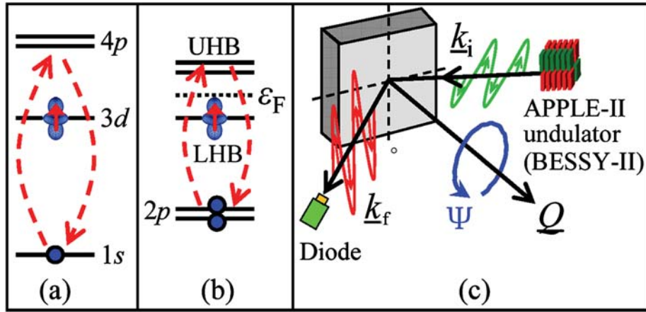
Figure 3.12: A schematic presentation of RXS at the different Mn absorption edges: (a) K -edge and (b) L_{II,III} -edges. (c) Basic notations for the RSXS set-up at the UHV ALICE diffractometer at Berliner Elektronenspeicherring-Gesellschaft für Synchrotronstrahlung (BESSY).
