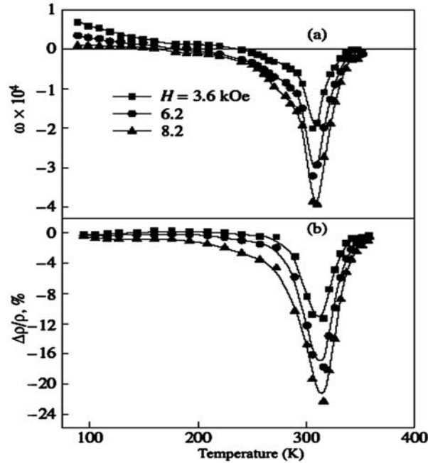
Figure 2.5: Temperature dependence of (a) volume magnetostriction \omega(H) and (b) magneto-resistance measured in various magnetic fields for \text{La}_{0.7}\text{Ba}_{0.3}\text{MnO}_3 [54].
