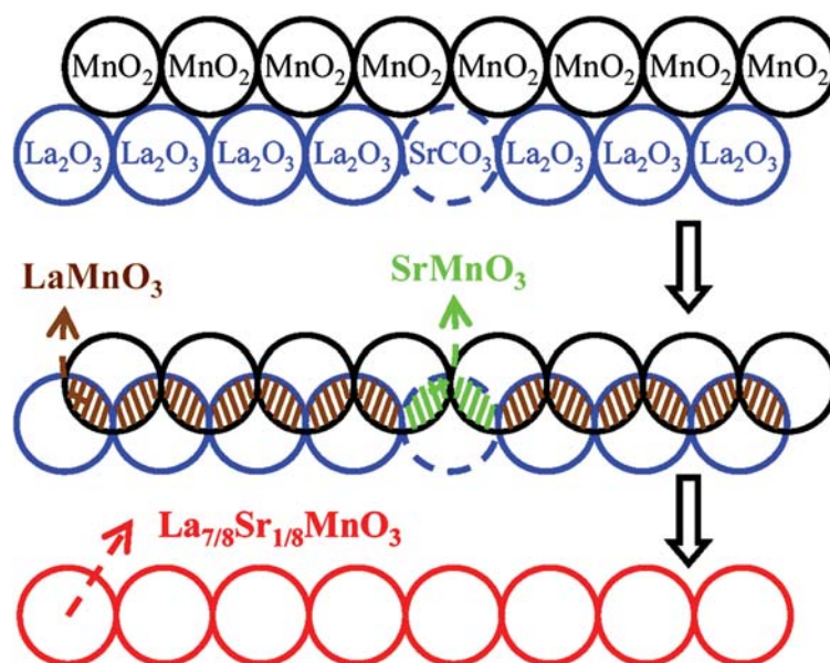
Figure 5.1: The ideal reaction process of raw materials ( \text{La}_2\text{O}_3 + \text{SrCO}_3 + \text{MnO}_2 ) for the formation of \text{La}_{7/8}\text{Sr}_{1/8}\text{MnO}_3 . In order to incarnate the doping level 1/8 , the particles are schematically depicted as spheres with an identical size and periodically arranged. This is actually hard to realize as discussed in the following part 5.2.2.
