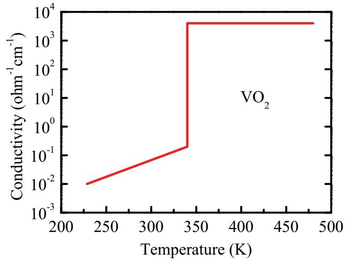
Figure 2.4: Temperature dependence of the conductivity of VO 2 [46].
