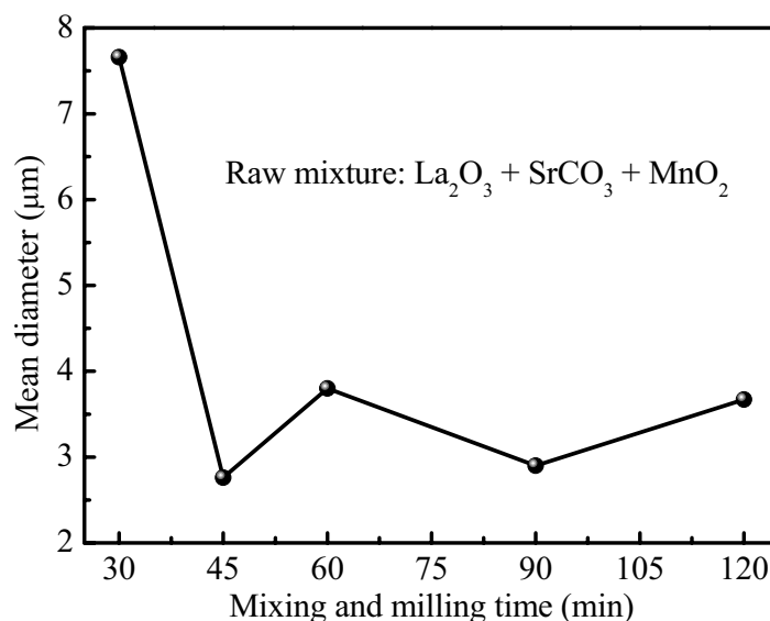
Figure 5.5: Mean diameter of a raw mixture of \text{La}_2\text{O}_3 , \text{SrCO}_3 and \text{MnO}_2 for the synthesis of \text{La}_{7/8}\text{Sr}_{1/8}\text{MnO}_3 versus ball mixing and milling time.
