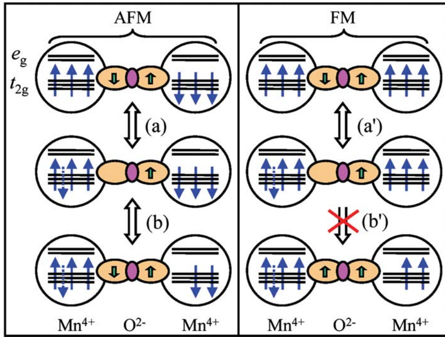
Figure 2.10: Illustration of the superexchange mechanism for \text{Mn}^{4+} ( 3d^3: e_g^0 t_{2g}^3 ) ions with the straight bonds. (left) Antiferromagnetism is indeed realized. (right) Ferromagnetism is rejected assuming non-orthogonal \text{Mn}^{4+} orbitals. It is stressed that the bottom configuration in the right is forbidden (see text).
