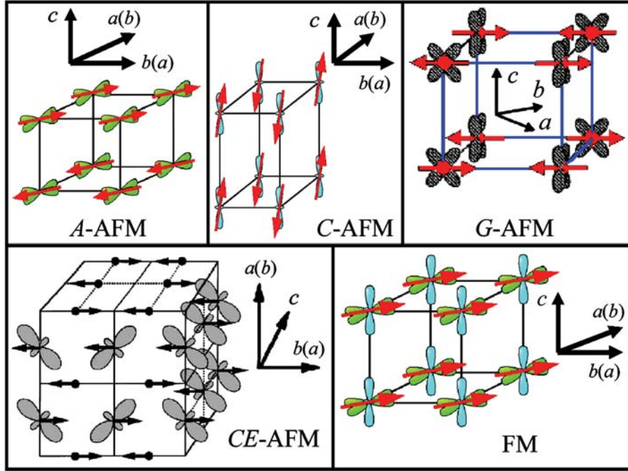
Figure 2.13: Spin order in \text{Nd}_{1-x}\text{Sr}_x\text{MnO}_3 at room temperature: ferromagnetic (FM) ( 0.3 < x < 0.5 ), A -type antiferromagnetic ( A -AFM) ( 0.5 < x < 0.7 ) and C -type antiferromagnetic ( C -AFM) ( x > 0.7 ) [71]. G -type antiferromagnetic ( G -AFM) spin order in \text{YVO}_3 below 77 K [108]. CE -type antiferromagnetic ( CE -AFM) spin order in most of the half-doped manganites [27].
