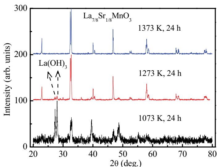
Figure 5.6: XRPD patterns of \text{La}_{7/8}\text{Sr}_{1/8}\text{MnO}_3 calcined at temperatures of 1073 K (bottom), 1273 K (middle) and 1373 K (top), respectively, for 24 h at each temperature.
