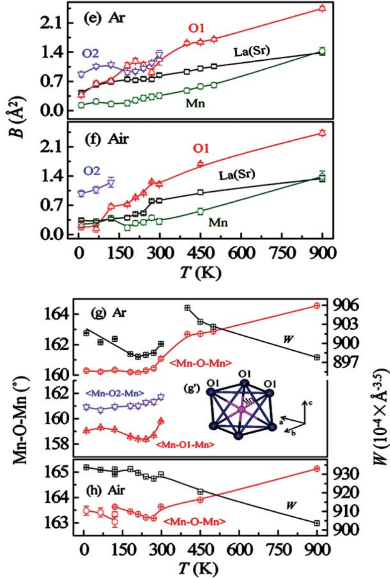
Figure 7.8 (continued): (e, f): temperature variation of the isotropic thermal parameters of La/Sr, Mn and O atoms for (e) the Ar annealed and (f) the air sintered samples. (g, h): mean Mn-O-Mn bond angle (left) and one-electron bandwidth W of the e_g -band (right) versus temperature for (g) the Ar annealed and (h) the air sintered samples. Bottoms of (c) and (g) show the individual Mn-O bond length and Mn-O-Mn bond angle of the Ar annealed sample, respectively. Insets (c') and (g') show schematic illustrations of \text{MnO}_6 octahedra in the O and R structures, respectively, illustrating the relevant bond lengths. Inset (d') shows the individual Mn-O bond length of the air sintered sample in the O structural region. The solid lines are guides to the eye.
