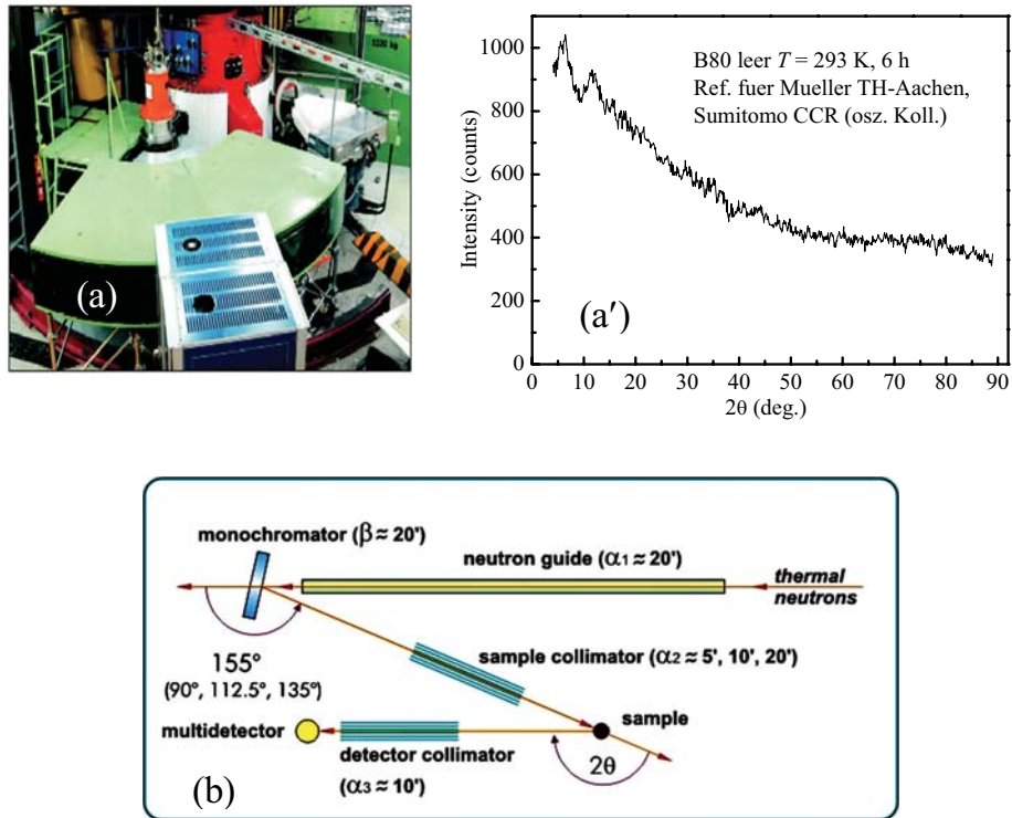
Figure 4.2: (a) Photograph of the SV7-a neutron powder diffractometer at the FRJ-2 [127]. (a') Background measurement at the SV7-a. (b) Principle of the structure powder diffractometer SPODI at the FRM-II [128].
