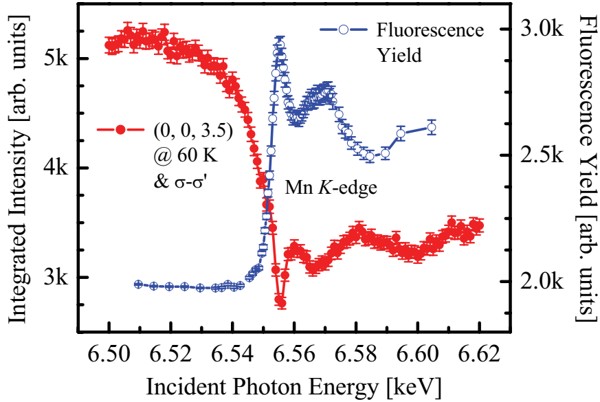
Figure 8.10: No appreciable resonant enhancement of the CO reflection (0 0 3.5) in Pbnm symmetry in \text{La}_{1-x}\text{Sr}_x\text{MnO}_3 ( x \approx 1/8 ) can be observed at the Mn K -edge at 60 K.
