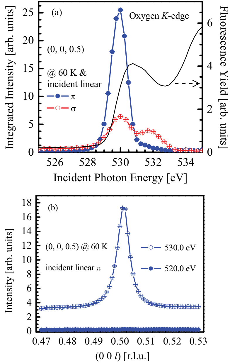
Figure 8.12: (a) A significant resonance enhancement of the CO reflection (0, 0, \frac{1}{2}) in Pbnm symmetry in \text{La}_{1-x}\text{Sr}_x\text{MnO}_3 ( x \approx \frac{1}{8} ) is clearly seen at the oxygen K -edge at 60 K. (b) Longitudinal scans of (0, 0, \frac{1}{2}) in Pbnm symmetry at different incident photon energies with incident \pi polarization at 60 K.
