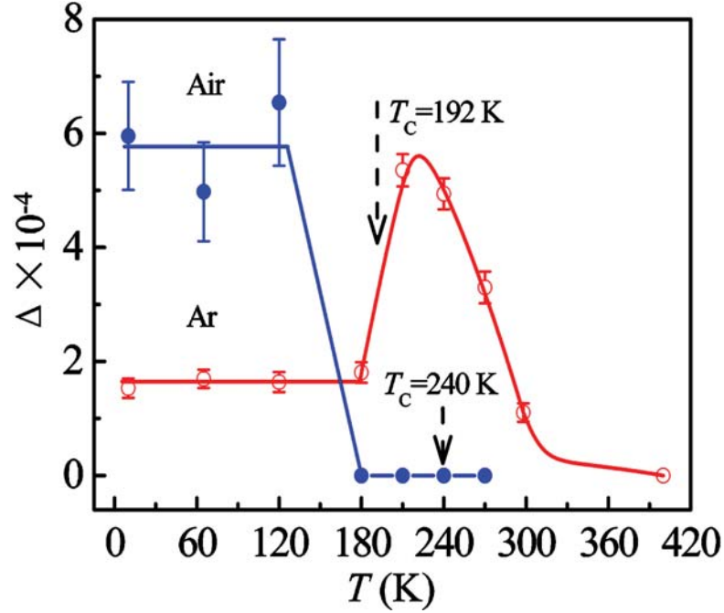
Figure 7.11: Temperature variation of the coherent JT distortion parameter \Delta of \text{MnO}_6 octahedra for Ar annealed and air sintered \text{La}_{0.875}\text{Sr}_{0.125}\text{Mn}_{1-\gamma}\text{O}_{3+\delta} samples. T_c (Ar) = 192 K and T_c (Air) = 240 K are based on the SQUID measurements. The solid lines are guides to the eye.
