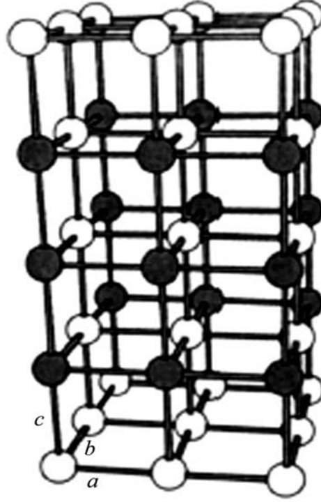
Figure 8.1: The pattern of hole order proposed for \text{La}_{1-x}\text{Sr}_x\text{MnO}_3 ( x \approx 1/8 ) in its FMI state. The holes are distributed over three-line stripes in every second a - c plane along the a axis. Hole rich planes are separated by undoped planes. Solid circles represent Mn sites containing the hole states, circles \text{Mn}^{3+} ions. Taken from [179].
