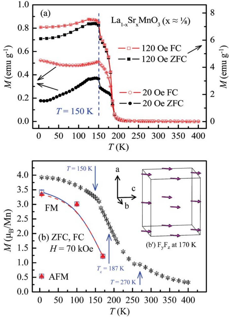
Figure 8.8: (a) ZFC and FC magnetization M at 20 and 120 Oe versus temperature for a powdered \text{La}_{1-x}\text{Sr}_x\text{MnO}_3 ( x \approx 1/8 ) single crystal. (b) Temperature dependence of the ZFC (up triangles) and FC (down triangles) magnetic moment \mu_B per Mn ion at 70 kOe and the refined FM (5, 100 and 170 K) and A-AFM (5 K) moments ( P12_1/c1 : squares; Pnma : solid triangles). Insets (b') illustrates the magnetic structure unit-cell F_y F_z in P12_1/c1 symmetry at 170 K. F_y and F_z denote the FM moments along the b and c axes, respectively.
