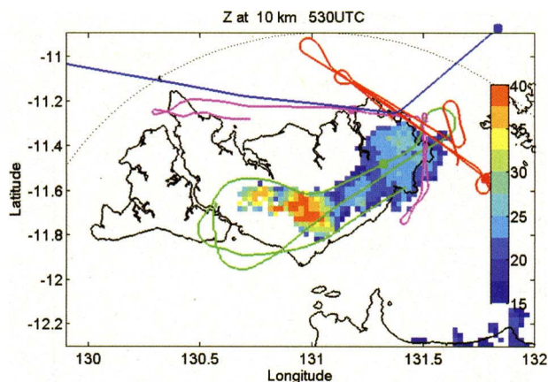
FIG. 10. Aircraft flight tracks superimposed on radar reflectivity (dBZ) at 10 km, for 0530 UTC (1500 LT) 30 Nov. Geophysica (green; probing the convective cores), Egrett (red; probing outflow), Falcon (blue), and Dornier (magenta). Solid circle denotes exact position of plane at the time of the image; Geophysica and Falcon tracks are shown at 20 min on either side of this time and Egrett and Dornier at \pm 40 min.
