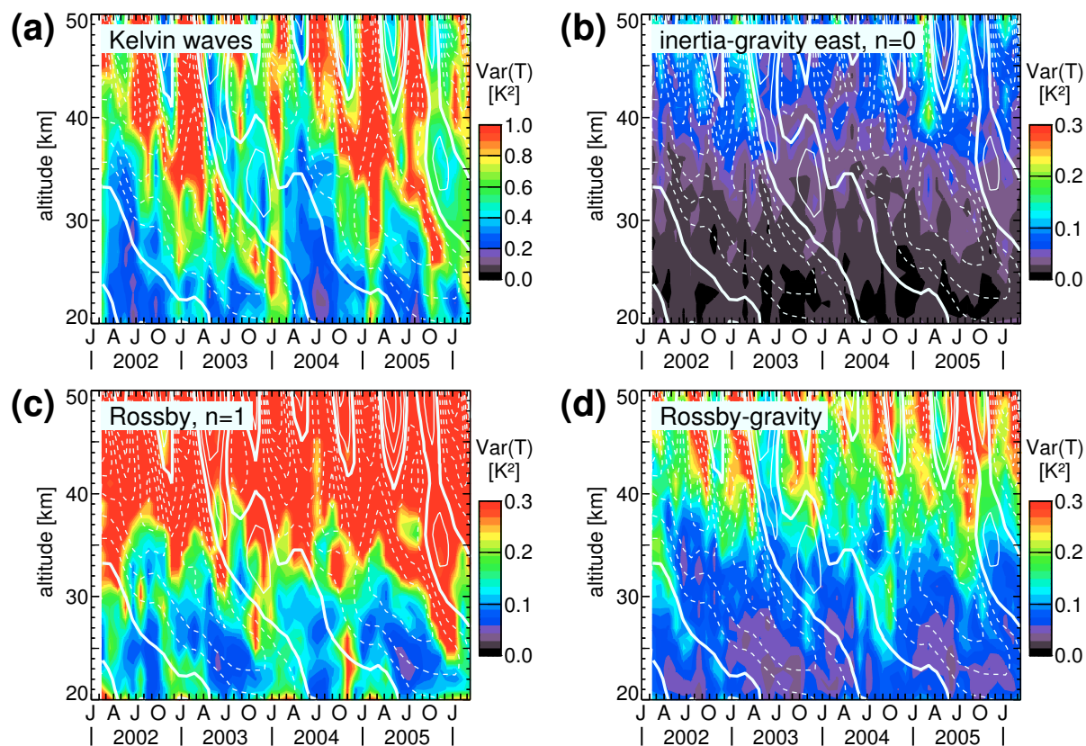
Fig. 9. Altitude-time cross-sections of SABER temperature variances integrated over the “fast” wave bands between 90 and 2000 m equivalent depth for (a) Kelvin waves, (b) inertia-gravity waves ( n=0 ), (c) equatorial Rossby waves ( n=1 ), and (d) Rossby-gravity waves. Overplotted contour lines are zonal mean zonal wind from ECMWF averaged over the latitudes 15°S–15°N. Contour interval is 10 m/s, solid lines indicate eastward, dashed lines westward wind. The zero wind line is highlighted by a boldface solid line.
