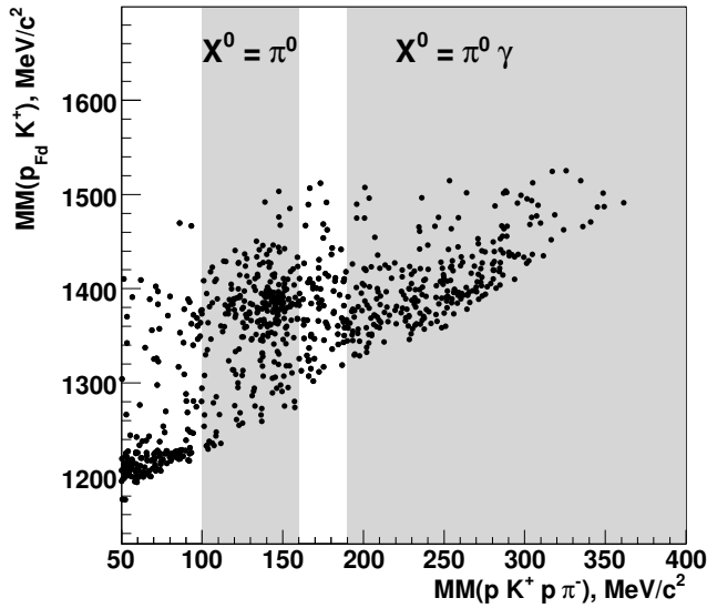
Fig. 2. Missing mass MM(p_{Fd}K^+) versus MM(pK^+p\pi^-) . A clear concentration of \pi^0 events is seen, though with a central value of the mass \sim 8 \text{ MeV}/c^2 too high, a deviation that is consistent with the resolution expected for a four-particle missing mass. The left shaded vertical box covers this \pi^0 region and the right one has MM(pK^+p\pi^-) > 190 \text{ MeV}/c^2 originating, e.g., from \pi^0\gamma and \pi\pi .
