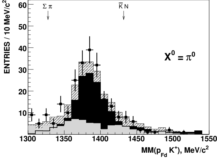
Fig. 3. Missing-mass MM(p_{Fd}K^+) distribution for the pp \rightarrow pK^+p\pi^-X^0 reaction for events with M(p_{Sd}\pi^-) \approx m(\Lambda) and for MM(pK^+p\pi^-) \approx m(\pi^0) . Experimental points with statistical errors are compared to the shaded histogram of the fitted overall Monte Carlo simulations. The simulation includes resonant contributions (solid-black) and non-resonant phase-space production (solid-grey). The structure in the latter arises from the various channels considered. Arrows indicate the \Sigma\pi and \bar{K}N thresholds.
