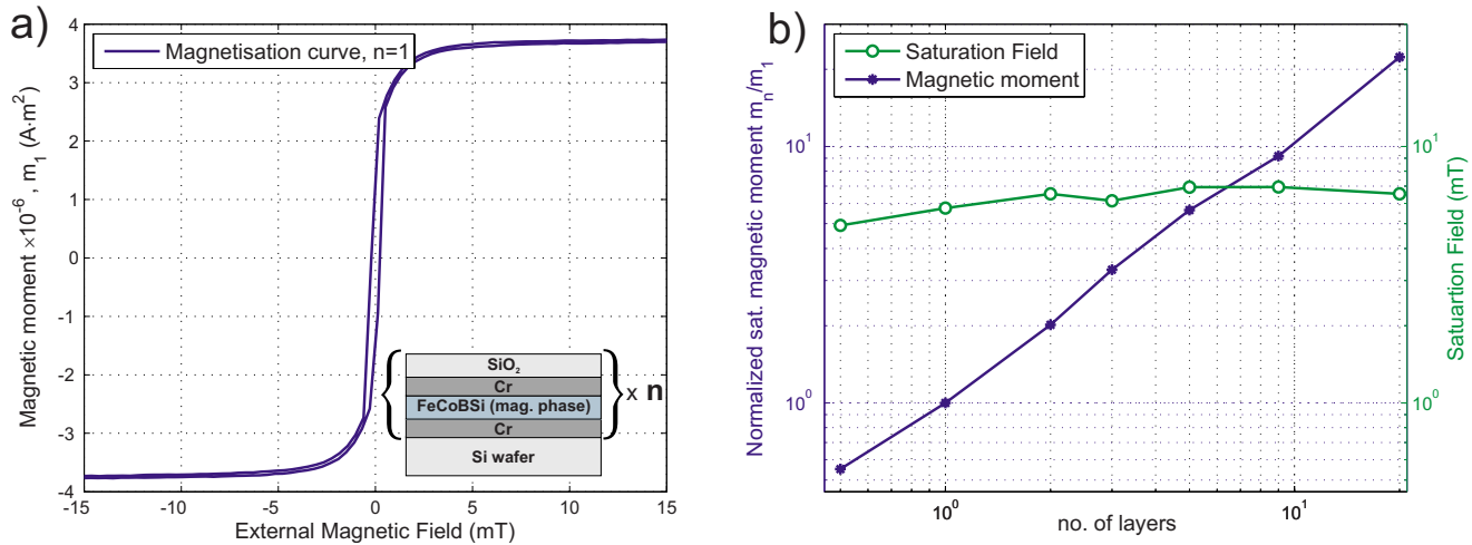
FIG. 3. (Color online) Magnetic properties of multilayer samples used to investigate the sensor performance. As magnetic phase \text{Fe}_{67}\text{Co}_{18}\text{B}_{14}\text{Si}_1 has been used. (a) The magnetization curve measured using a vibrating sample magnetometer for one layer sample. (b) The dependence of the saturation magnetic moment on the number of magnetic layers is linear, whereas the saturation field remains unchanged.
