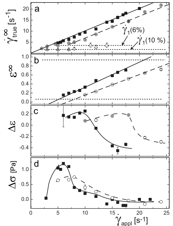
FIG. 3: Steady state values of (a) the true shear rate \dot{\gamma}_{\text{true}}^\infty and (b) the proportion of the high SB \varepsilon^\infty , and amplitudes of the relaxations of (c) the proportion of the high SB \Delta\varepsilon and (d) the excess shear stress \Delta\sigma as a function of the imposed shear rate \dot{\gamma}_{\text{appl}} . Solid (open) symbols refer to stick (slip) BC. All data are for 6 wt. % CPyCl–NaSal except for the triangles in (a) which are for 10 wt. % CPyCl–NaSal with slip BC. In (a) the solid line is \dot{\gamma}_{\text{true}} = \dot{\gamma}_{\text{appl}} , while the dashed line is \dot{\gamma}_{\text{true}} = \dot{\gamma}_{\text{appl}} - 3.4 \text{ s}^{-1} and the dotted lines indicate \dot{\gamma}_1 for 6 and 10 wt. % CPyCl–NaSal. The dotted lines in (b) show the resolution limit for SB detection [19]. The lines in (c) and (d) are to guide the eye.
