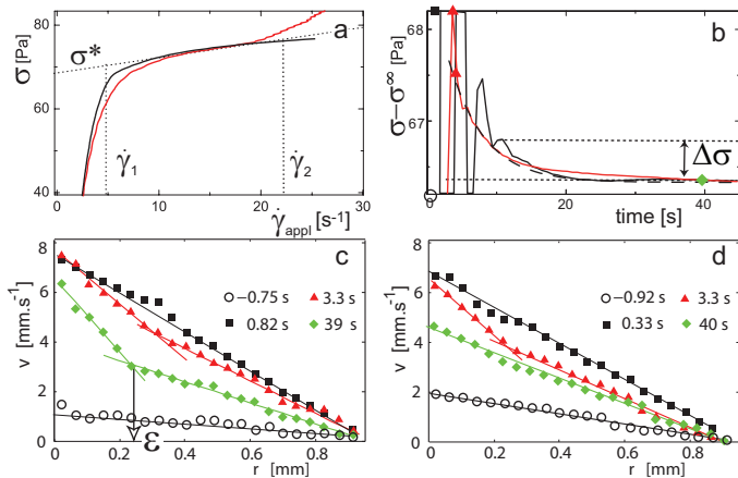
FIG. 1: (a) Steady-state flow curves of 6 wt. % CPyCl-NaSal for stick (black) and slip BC (red) for a shear rate sweep of 1200 s. (b) Stress responses \sigma(t) - \sigma^\infty after a shear rate quench to \dot{\gamma}_{\text{appl}} = 8 \text{ s}^{-1} at t = 0 for stick (black, \dot{\gamma}_{\text{init}} = 0.8 \text{ s}^{-1} ) and slip BC (red, \dot{\gamma}_{\text{init}} = 2 \text{ s}^{-1} ). The dashed line indicates an exponential decay with a characteristic time of 10 s. (c) Velocity profiles v(r, t) for stick BC at various times during the quench shown in (b) (see colored dots in (b)). r denotes the radial position from the inner rotating cylinder. (d) Same as (c) for slip BC.
