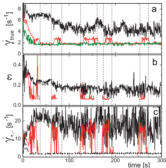
FIG. 4: Responses to shear rate quenches from \dot{\gamma}_{\text{init}} = 0.8 \text{ s}^{-1} to \dot{\gamma}_{\text{appl}} = 8 \text{ s}^{-1} for stick (black) and slip BC (red) in 10 wt. % CPyCl-NaSal. (a) True shear rate \dot{\gamma}_{\text{true}}(t) . The green line is the response to a quench to \dot{\gamma}_{\text{appl}} = 5 \text{ s}^{-1} for slip BC. (b) Proportion of the high SB \epsilon(t) . (c) Shear rate in the high SB \dot{\gamma}_{+}(t) (solid) and low SB \dot{\gamma}_{-}(t) (dashed, only stick BC). The vertical dashed lines indicate the times where SB nucleate and melt (see text). The gaps in the slip data in (b) and (c) are due to the lack of SB [19].
