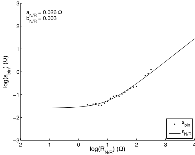
Figure 2. The standard deviation s_{bin} of the N/R misfits which were collected in bins and the corresponding error model fit \varepsilon_{N/R} for the first of the 48 ERT frames. The error model parameters a_{N/R} and b_{N/R} are shown at the top left.
