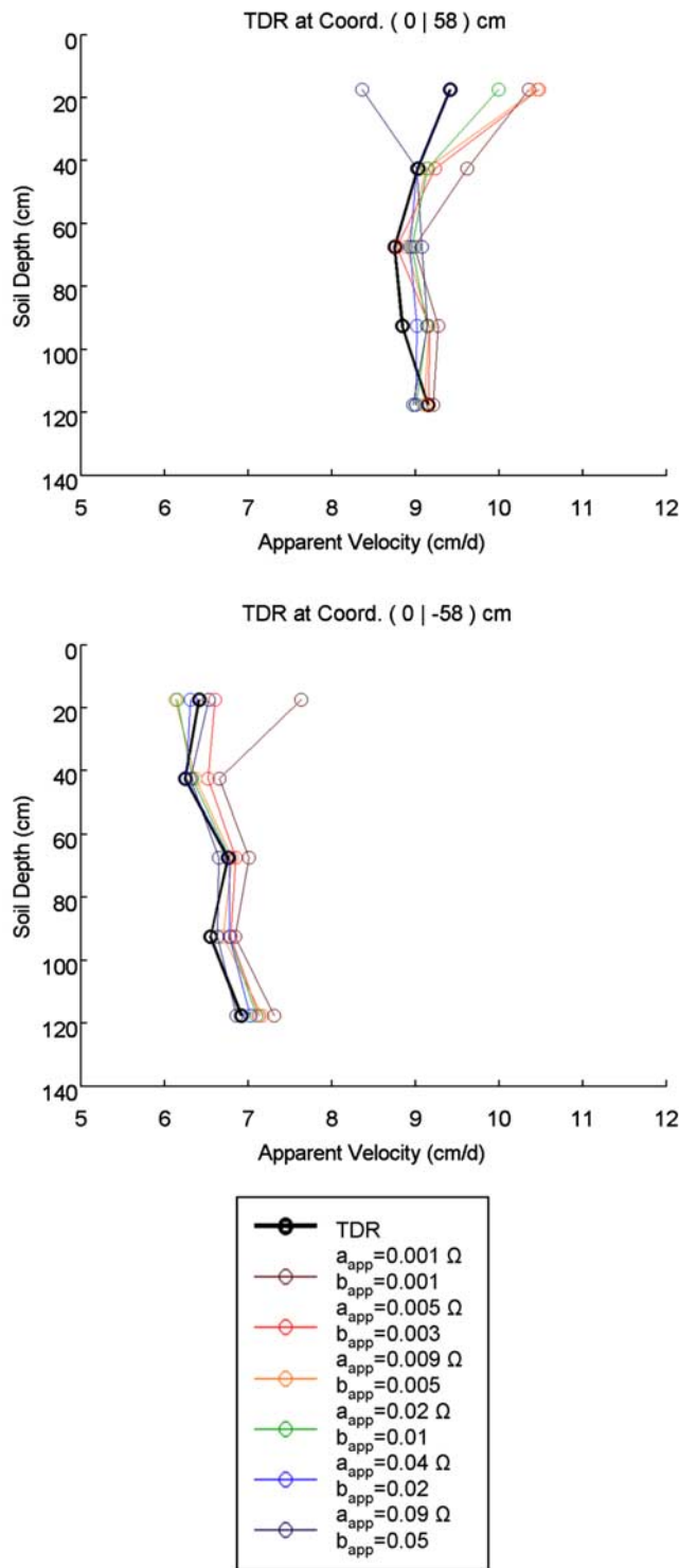
Figure 10. Apparent velocities v_a (cm/d) from TDR and the corresponding mean of the ERT voxel BTCs as a function of \varepsilon_{app} .
