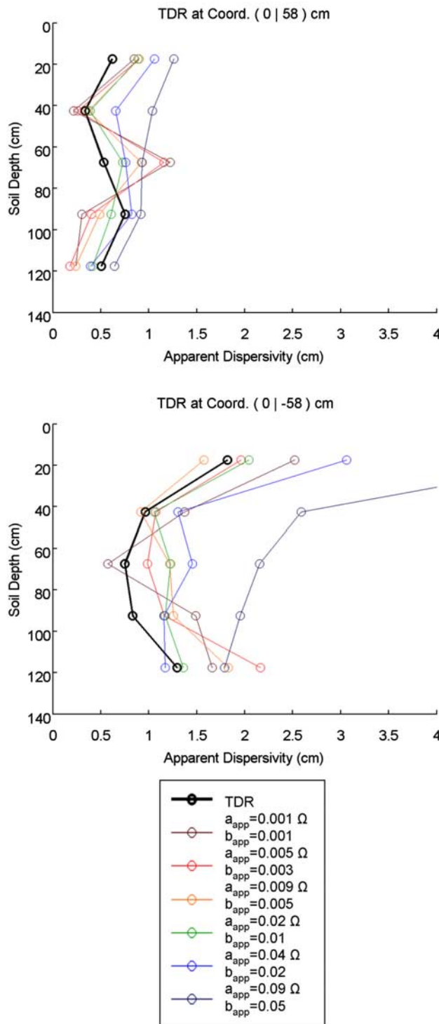
Figure 11. Apparent dispersivities \lambda_a (cm) from TDR and the corresponding mean of the ERT voxel BTCs as a function of \varepsilon_{app} .
