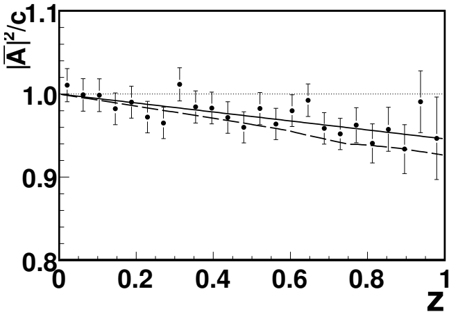
Figure 5: Extracted dependence of |\bar{A}|^2 on the z variable. The solid line is a c(1 + 2\alpha z) fit. The dashed line is a prediction of the cusp effect [37].
