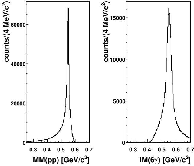
Figure 3: Missing mass of two protons, MM(pp) (left) and invariant mass of six photons, IM(6\gamma) (right) after selection of the pp6\gamma final state.
