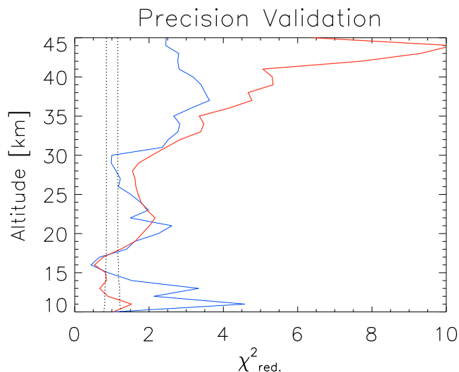
Fig. 15. \chi^2 analysis for precision validation for MIPAS and POAM III Southern hemispheric water vapour measurements. Blue: POAM III original profiles. Red: POAM III profiles smoothed with MIPAS averaging kernels. For details, see Fig. 3.
