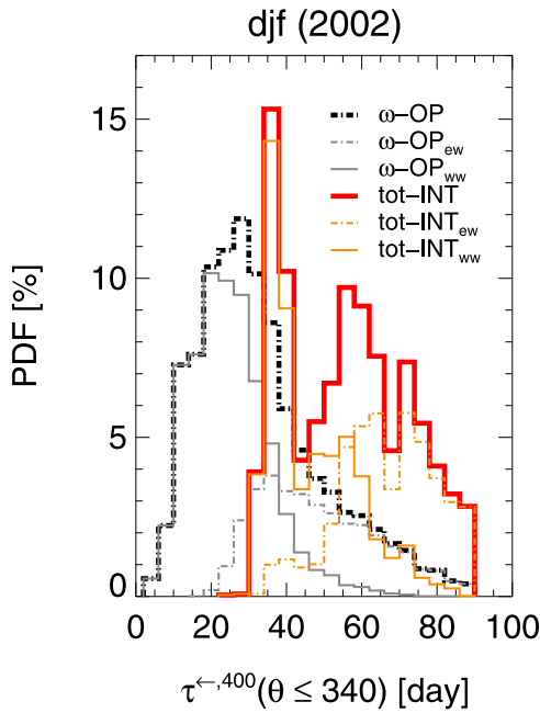
Figure 10. Formation of the two-peak shape of the transit time distribution of parcels at 400 K for ascending from 340 K. The thin gray and orange solid/dash-dotted lines denote the transit time distributions for net westward/eastward traveling trajectories. The bin size is 4 days.
