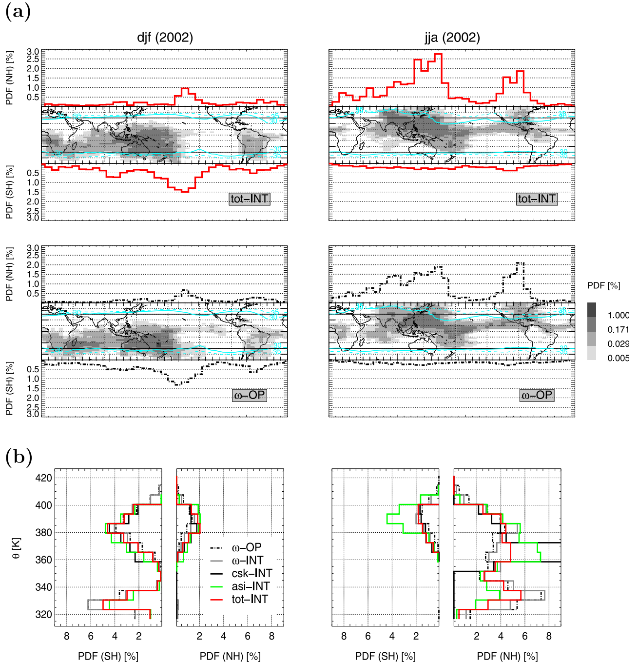
Figure 2. Vertical versus horizontal transport into the TTL for (left) December-January-February (djf) and (right) June-July-August (jja). (a) The gray color scheme shows regions of vertical transport into the TTL (PDF of entry locations at 350 K) for (top) tot-INT and (bottom) \omega -OP; notice the nonlinear color scale. The thin solid black/solid cyan and dashed cyan lines show the \pm 30^\circ latitude/ \pm 30^\circ and \pm 35^\circ equivalent latitude contours, as averages in the 350–400 K layer for the respective djf/jja period. The solid/dashed lines in the bottom and top areas of each plot describe PDFs of locations where the TTL trajectories crossed the meridional boundaries ( \pm 35^\circ N equivalent latitude), as functions of longitude. (b) PDFs of potential temperatures where the northern and southern hemispheric meridional boundaries are crossed (the peak value for csk-INT/jja is 27.5%). All distributions are normalized to the total number of trajectories initialized in the TTL.
