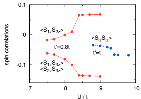
FIG. 2. (Color online) Nearest-neighbor spin correlations in isotropic and anisotropic triangular lattices for T = 0.05t , t' = t_{12} , and t = t_{13} = t_{23} . Strong enhancement of spin correlations occurs for moderate deviations from the isotropic limit.
