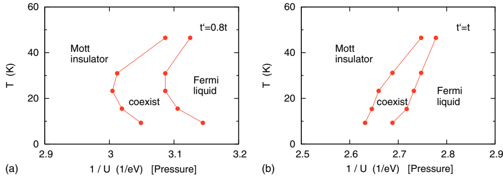
FIG. 1. (Color online) Phase diagrams of Hubbard model for anisotropic triangular lattice ( t' = 0.8t ) and isotropic triangular lattice ( t' = t ), evaluated within ED cluster DMFT for t = 0.04 eV. Plotted are the first-order metal-insulator phase boundaries as functions of inverse local Coulomb energy U . In the experimental setup increasing hydrostatic pressure P implies increasing bandwidth W or decreasing U . The re-entrant behavior found for t' = 0.8t is absent in the isotropic limit t' = t .
