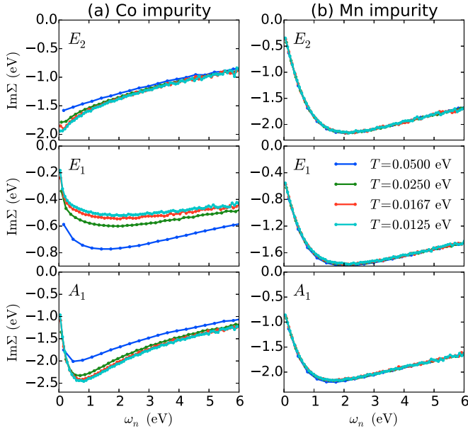
FIG. 4. The imaginary part of the self-energy as a function of Matsubara frequency at T = 1/20, 1/40, 1/60 , and 1/80 eV for Co impurity (column a) and Mn impurity (column b). Each row corresponds to a d orbital ( E_2 , E_1 , or A_1 ). The d occupancies are set at N_d = 7.86 for Co and 5.68 for Mn (close to the KKR values of N_d ). The on-site interaction is U = 4 eV. Orbital occupancies corresponding to E_2, E_1 and A_1 at T = 1/80 = 0.0125 eV are 0.53, 0.60 , and 0.56 for Mn, 0.75, 0.93 , and 0.57 for Co.
