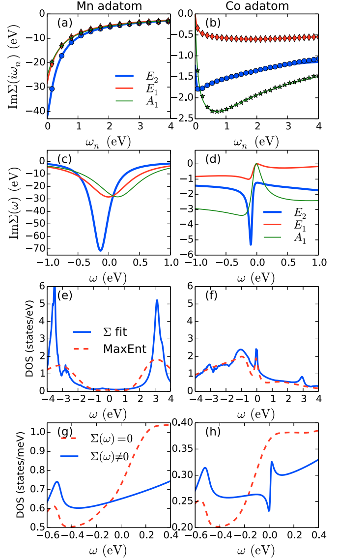
FIG. 8. First line: comparison of the rational fit function [Eq. (10) with N = 3 ] (solid lines) to the CT-QMC data for \text{Im } \Sigma(i\omega_n) (symbols) for Mn (a) and Co (b). Second line: analytical continuation of the CT-QMC \Sigma(i\omega_n) to real frequency \text{Im } \Sigma(\omega + i0) using the rational fit function [Eq. (10)] for Mn (c) and Co (d). Third line: local d DOS for the adatoms, via MaxEnt and by solving the KKR Dyson equation with the results from (c) and (d) for Mn (e) and Co (f). Fourth line: STM spectra in vacuum 4.2 Å vertically above the adatom [Eq. (2)] for Mn (g) and Co (h). The impact of the self-energy is highlighted by comparing the DOS before and after the self-energy is taken into account. The following parameters are used: U = 4 eV, J = 0.9 eV, T = 0.025 eV at N_d = 5.04 for Mn and N_d = 7.85 for Co.
