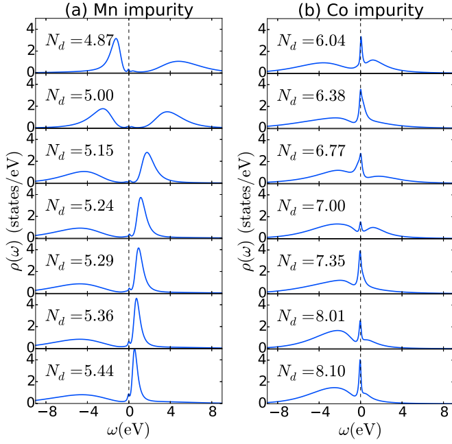
FIG. 6. The evolution of spectral functions \rho_m(\omega) with increasing filling N_d for Mn (a) and Co (b). The on-site interaction parameters are U = 4 eV, J = 0.9 eV, and the temperature is T = 0.05 eV.
