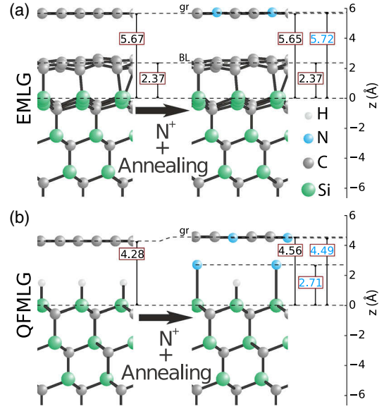
FIG. 2. Summary of the vertical positions (in Å) measured by the NIXSW technique for each atomic species in (a) EMLG and in (b) QFMLG, before and after N doping.
