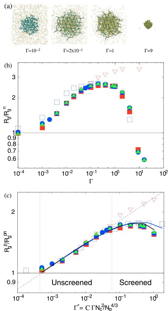
Figure 1. (a) Snapshots of gel particles in the presence of counterions (yellow) for various Coulomb interaction strengths \Gamma as indicated. (b) Dependence of the nanogel radius of gyration R_g on the interaction strength \Gamma for N_c = 147 and the system sizes L/l = 200 (■), 300 (●), 400 (▲), and N_c = 729 for the system size L/l = 400 (□). The symbols \nabla indicated simulation results without counterions for N_c = 147 . R_g^n is the radius of gyration of a neutral gel, where R_g^n/l = 17.6 for N_c = 147 and 31.0 for N_c = 729 . (c) Average radii of gyration of individual polymers R_g^p as function of the effective interaction strength \Gamma^* . The dashed line is proportional to (\Gamma^*)^{0.12} . The solid lines are the numerical solutions of the equation \partial F / \partial R_E = 0 , with F of Eq. (12). C = 0.032 for N_c = 147 (black) and 0.045 for N_c = 729 (red). R_g^{pn} ( = 2.6l ) denotes the average radius of gyration of individual polymers.
