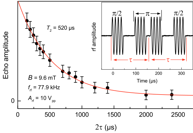
FIG. 3. Nuclear spin echo amplitude in dependence on the total time delay 2\tau . The red line is an exponential fit. The inset illustrates the employed rf pulse scheme (time dependence of the normalized rf amplitude).
