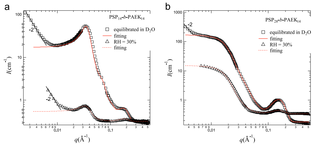
Fig. 1. Part (a) SANS profiles of PSP 14 - b -PAEK 14 membranes equilibrated at RH=30% (triangles) and fully D 2 O-swollen state (squares) at room temperature. The best-fitted theoretical curves ranging from the middle- q region based on HS model to the high- q region based on Eq. (6) for both membranes are also shown in the figure by red dashed and solid lines, respectively. Part (b) SANS profiles of PSP 28 - b -PAEK 14 membranes equilibrated at RH=30% (triangles) and fully D 2 O-swollen state (squares) at room temperature. The best-fitted theoretical curves ranging from the middle- q region based on HS model to the high- q region based on Eq. (6) for both membranes are also shown in the figure by red dashed and solid lines, respectively.
