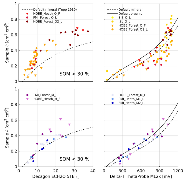
Figure 2. Decagon 5TE apparent relative permittivity \epsilon_a (left panels) and ThetaProbe voltage (mV) (right column panels) against volumetric moisture content \theta for organic (SOM > 30\% , top row panels) and mineral soil horizons (SOM < 30\% , bottom row panels), laboratory \bullet and field \blacktriangledown data, with color codes from highest to lowest SOM content (yellow–dark red and purple–dark blue, respectively). For mineral horizons, blue and purple signatures mean SOM < 10 and > 10\% , respectively. Manufacturer’s default calibration curves (black dashed and continuous lines) are also included. Regarding the specifications of sample names and respective SOM fractions, please see Table 1.
