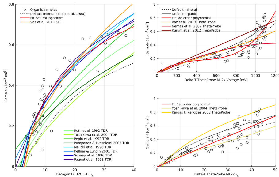
Figure 4. Comparison between reported petrophysical and empirical relationships applied to our data measured in organic soil layers for the Decagon 5TE apparent relative permittivity \epsilon_a (left panel), and ThetaProbe voltage (mV) (upper right panel) as well as \epsilon_a (lower right panel) against volumetric moisture content \theta including respective manufacturer's default calibration curves and best fits.
