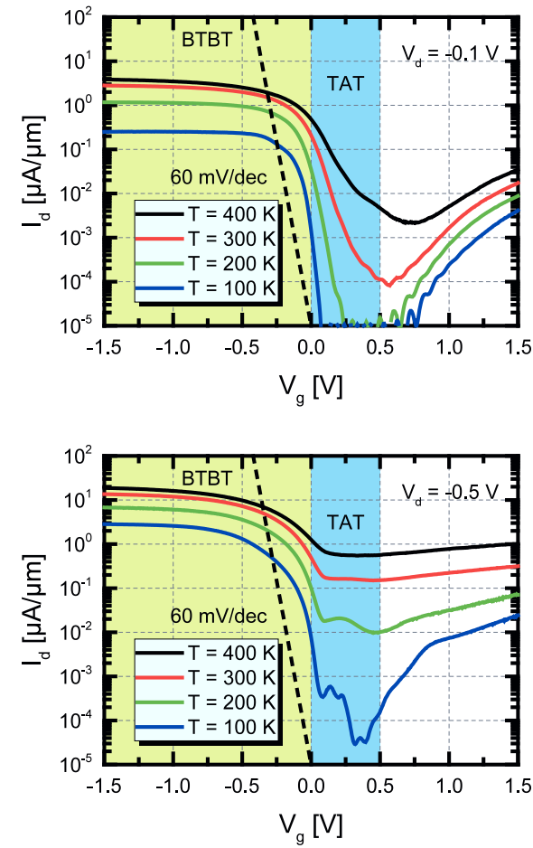
Figure 4.2.37: Measured transfer characteristics of the planar SiGe/Si heterostructure p-TFET at different temperatures T for drain voltages V_d of -0.1 V and -0.5 V in case of biasing in p-MOS mode, revealing switching of the planar SiGe/Si heterostructure p-TFET only at a drain voltage V_d of -0.1 V whereas at a drain voltage V_d of -0.5 V the transistor exhibits no more switching due to the (gated) tunnel diode biased in forward direction.
