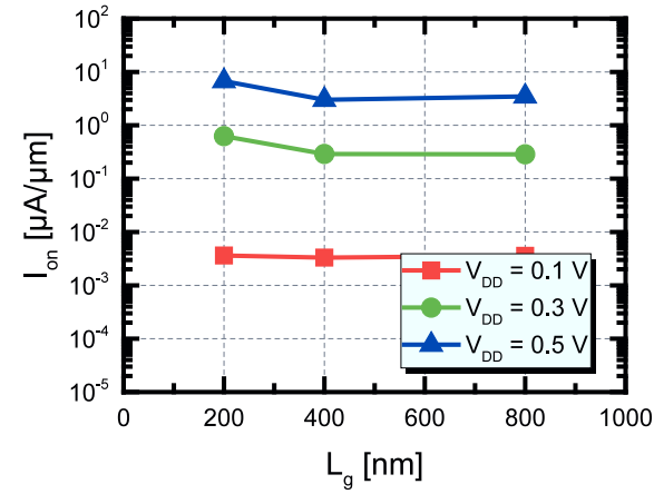
Figure 4.2.8: On-current I_{on} of the planar SiGe/Si heterostructure p-TFET as a function of the gate length L_g , revealing no pronounced dependency of the on-current I_{on} of the planar SiGe/Si heterostructure p-TFET as a function of the gate length L_g , thus excluding parasitic contributions from a SCHOTTKY junction at the interface between CoSi 2 and n ++ -SiGe.
