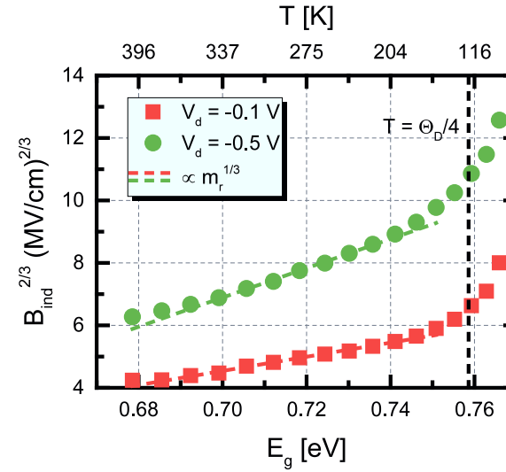
Figure 4.2.34: Third root squared of the material dependent parameter B_{\text{ind}}^{2/3} of the planar SiGe/Si heterostructure p-TFET as a function of the band gap E_g , revealing a linear dependency as a clear indication of BTBT dominating charge transport in the planar SiGe/Si heterostructure p-TFET. The slope of the curve is proportional to the third root of the reduced tunneling mass m_r^{1/3} . A freeze-out of phonons occurs at a temperature T of about 120 K, corresponding to one fourth of the DEBYE temperature T = \frac{\Theta_D}{4} as indicated by a dotted vertical line.
