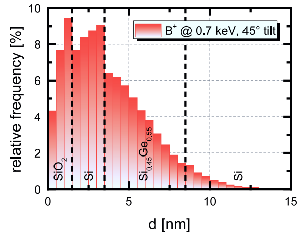
Figure 4.1.2: Simulated ion distribution within the sample after implantation with Boron ions at an energy of 0.7 keV at a tilt angle of 45° in order to form a shallow doping only in the SiGe layer and not in the SOI substrate underneath. The resulting implantation peak of the ion distribution is located at the interface between Si cap and SiGe layer.
