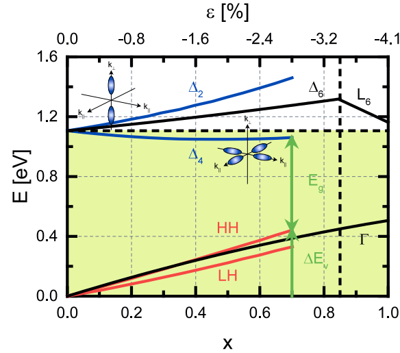
Figure 2.4.1: Schematic illustration of the band structures of relaxed and strained SiGe as a function of the Ge mole fraction x and the corresponding compressive biaxial strain \varepsilon within the SiGe layer based on nonlocal empirical pseudopotential method (EPM) calculations [41, 40, 42]. The band structure of relaxed SiGe changes from Si-like into Ge-like at a Ge mole fraction x of about 0.85 as indicated by a dashed vertical line. The dashed horizontal line in turn depicts the band gap E_g of Si at room temperature T = 300 K as a reference level for the valence band offset \Delta E_v . Compressive, biaxial strain \varepsilon introduced by the pseudomorphic growth breaks the lattice symmetry of the relaxed SiGe layer, lifting both the degeneracy of the \Delta_6 conduction band valleys as well as the degeneracy of LH and HH bands stemming from the \Gamma valley. The \Delta_6 conduction band valleys split into \Delta_4 and \Delta_2 valleys with the former lowered in energy whereas the HH band is increased in energy with respect to the LH band. Thus, the band gap E_g of compressively, biaxially strained SiGe is determined by the difference of the \Delta_4 conduction band valleys and the HH band.
