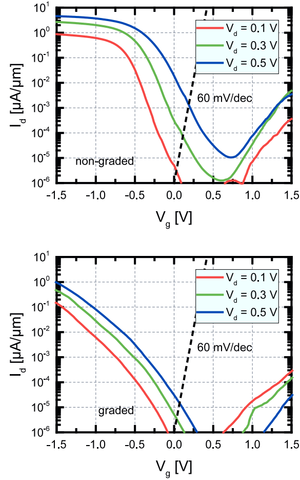
Figure 3.2.4: Measured transfer characteristics of a non-graded and a graded vertical SiGe/Si heterostructure n-TFET, exhibiting poor switching for positive gate voltages V_g > 0 , namely the n-branch of the transfer characteristics.
