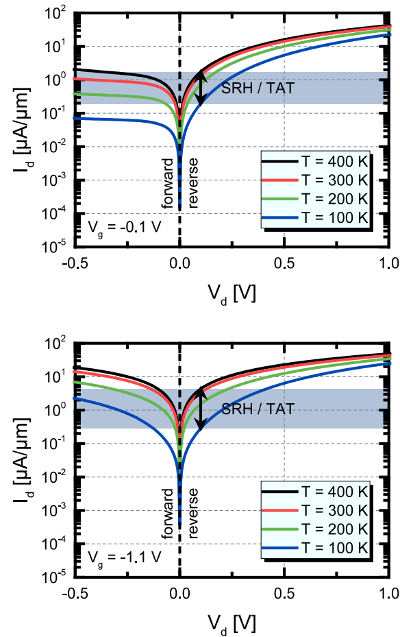
Figure 4.2.38: Measured output characteristics of the planar SiGe/Si heterostructure p-TFET at different temperatures T for gate voltages V_g of -0.1 V and -1.1 V in case of biasing in p-MOS mode, revealing a similar spreading of the drain current I_d as a function of the temperature T for both gate voltages V_g , thus confirming BTBT dominating over SRH and TAT in the planar SiGe/Si heterostructure p-TFET already at low absolute gate voltages |V_g| .
