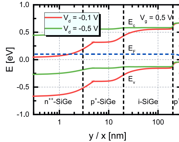
Figure 4.2.12: Simulated band structure of the planar SiGe/Si heterostructure p-TFET in case of biasing in p-MOS mode at a gate voltage V_g of 0.5 V for drain voltages V_d of -0.1 V and -0.5 V, allowing for thermionic emission in case of the latter due to prevailing flat-band conditions.
