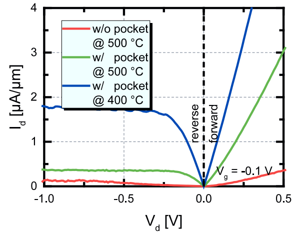
Figure 4.2.17: Measured output characteristics of the planar SiGe/Si heterostructure p-TFET at a gate voltage V_g of -0.1 V, comparing the influence of the counter doped pocket as well as the impact of the temperature T during DS on the overall device performance. The planar SiGe/Si heterostructure p-TFET drastically benefits from a counter doped pocket enabling a linear onset of the drain current I_d whereas the device without counter doped pocket suffers from a S-shaped, superlinear onset of the drain current I_d as a clear indication of a degraded source tunnel junction.
