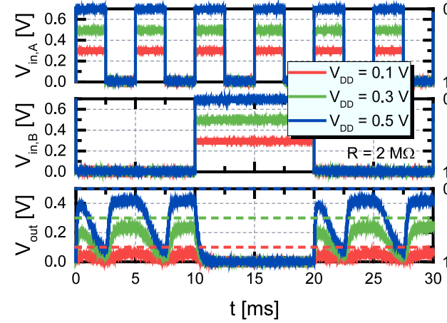
Figure 4.2.42: Measured time response of a NAND gate with both gates swept in parallel for a pull-down resistor exhibiting a resistance R of 2\text{ M}\Omega , revealing p-logic operation by means of two planar SiGe/Si heterostructure p-TFETs connected in series. Only in case of both inputs providing a logic 1, a logic 0 at the output is achieved. In all other cases, a logic 1 at the output is stabilized, thus accomplishing a NAND gate.
