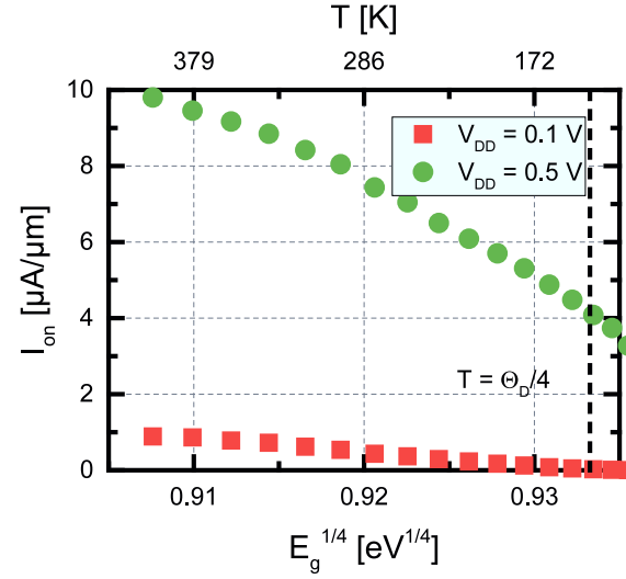
Figure 4.2.32: On-current I_{\text{on}} of the planar SiGe/Si heterostructure p-TFET as a function of the fourth root of the band gap E_g^{1/4} , revealing a linear dependency as a clear indication of line tunneling aligned with the gate electric field lines being the dominant contribution to BTBT. A freeze-out of phonons occurs at a temperature T of about 120 K, corresponding to one fourth of the DEBYE temperature T = \frac{\Theta_D}{4} as indicated by a dotted vertical line.
