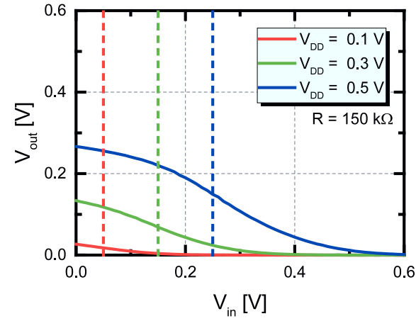
Figure 4.2.40: Measured VTC of a NAND gate with both gates swept in parallel in case of a pull-down resistor exhibiting a resistance R of 150 \text{ k}\Omega . For this particular case, switching of the output voltage V_{\text{out}} at an input voltage V_{\text{in}} of about \frac{V_{\text{DD}}}{2} is realized, but inverting of the input voltage V_{\text{in}} is degraded due to a broad transition of the output voltage V_{\text{out}} .
