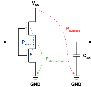
Figure 2.1.1: Schematic illustration of the different contributions to power consumption arising in integrated circuits. Dynamic power P_{\text{dynamic}} and short-circuit power P_{\text{short-circuit}} are consumed when transistors change their logic state due to charging and discharging of load capacitors C_{\text{load}} whereas static power P_{\text{static}} in turn dissipates due to different leakage contributions.
