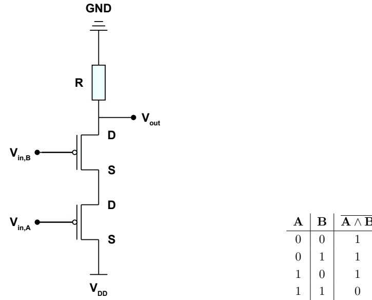
Figure 4.2.39: Schematic illustration of a NAND gate realized by p-logic.
