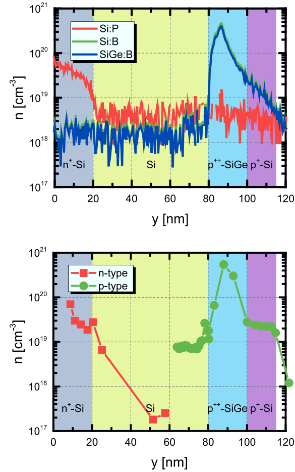
Figure 3.1.1: Doping profile of the vertical SiGe/Si heterostructure n-TFET measured by SIMS and ECV, revealing both a sharp doping profile with a steepness \lambda_s of about 3 nm/dec in direction to the Si channel and a high carrier concentration n up to 4 \times 10^{20} \text{ cm}^{-3} within the SiGe source.
