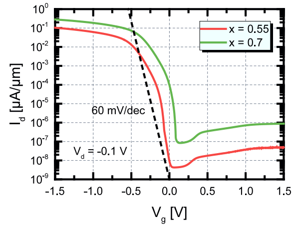
Figure 4.2.23: Simulated transfer characteristics of the planar SiGe/Si heterostructure p-TFET at a drain voltage V_d of -0.1 V when increasing the Ge mole fraction x from 0.55 to 0.7, enabling both an increased on-current I_{on} and an improved subthreshold swing SS .
