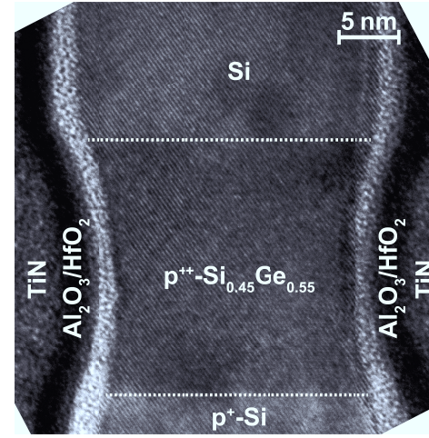
Figure 3.1.4: TEM image of the vertical SiGe/Si heterostructure n-TFET, revealing high crystalline quality of both the Si and the compressively, biaxially strained Si 0.45 Ge 0.55 layers.
