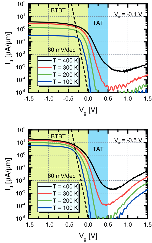
Figure 4.2.29: Measured transfer characteristics of the planar SiGe/Si heterostructure p-TFET at different temperatures T for drain voltages V_d of -0.1 V and -0.5 V in case of biasing in p-TFET mode, highlighting the different contributions from both TAT and BTBT to the overall drain current I_d of the planar SiGe/Si heterostructure p-TFET.
