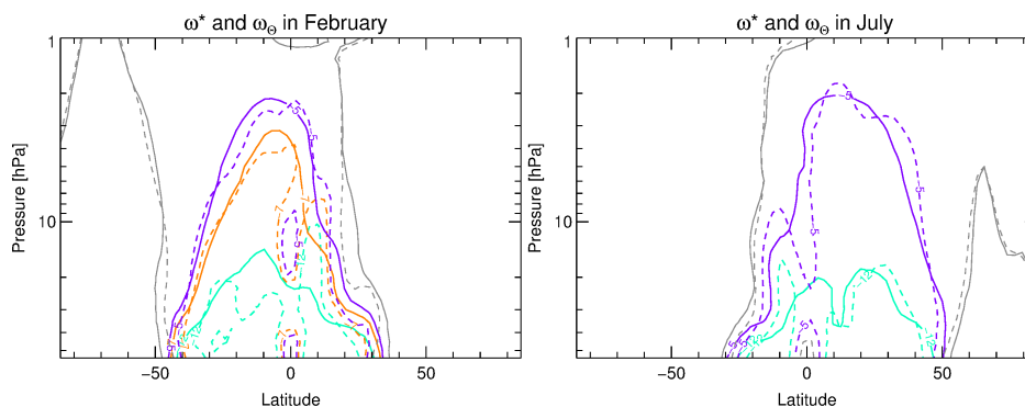
Figure 5. Kinematic vertical velocity ( \omega^* , dashed lines) and diabatic vertical velocity ( \omega_\theta , solid lines) for February (left panel) and July (right panel) in the 10-year climatology. Different contours for selected velocity values are shown: 0 \text{ Pa day}^{-1} (grey), -5 \text{ Pa day}^{-1} (violet), -7 \text{ Pa day}^{-1} (orange), and -12 \text{ Pa day}^{-1} (turquoise).
