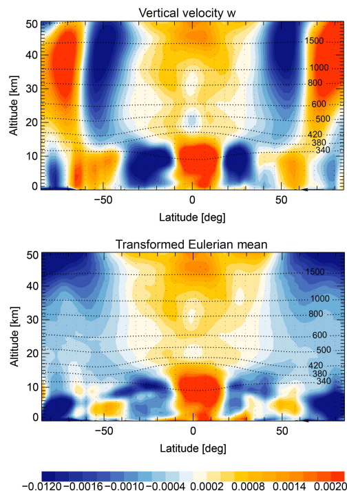
Figure 2. Annual, zonal mean vertical velocity \bar{w} ( \text{ms}^{-1} ) (top panel) and transformed Eulerian mean (TEM) vertical velocity \bar{w}^* ( \text{ms}^{-1} ) (bottom panel) from EMAC for the year 2005. Dotted lines display potential temperature levels (K). The vertical axis displays log-pressure height (km), calculated from Eq. (4).
