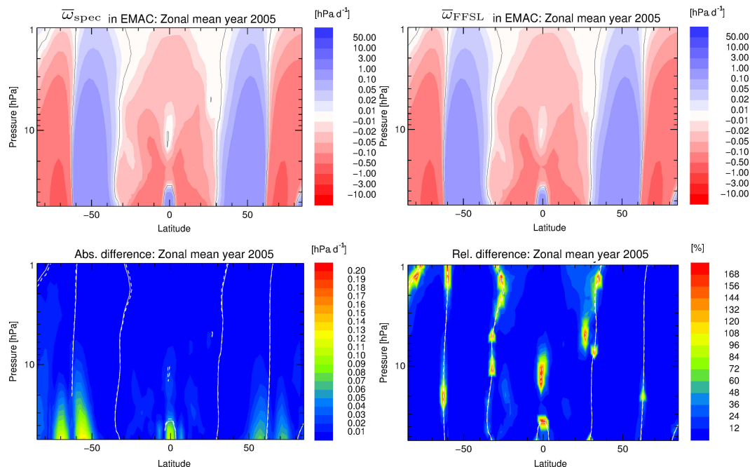
Figure 1. Annual, zonal mean \bar{\omega}_{\text{spec}} (top left panel) and \bar{\omega}_{\text{FFSL}} (top right panel) ( \text{hPa day}^{-1} ) for the year 2005. Here, black solid lines show the 0 \text{ hPa day}^{-1} contour of the respective vertical velocities. The bottom panels show absolute value of absolute difference ( \text{hPa day}^{-1} ) (left) and relative difference (right) between \bar{\omega}_{\text{spec}} and \bar{\omega}_{\text{FFSL}} . White dashed and solid lines in the bottom panels display the 0 \text{ hPa day}^{-1} contour of \bar{\omega}_{\text{spec}} and \bar{\omega}_{\text{FFSL}} , respectively.
