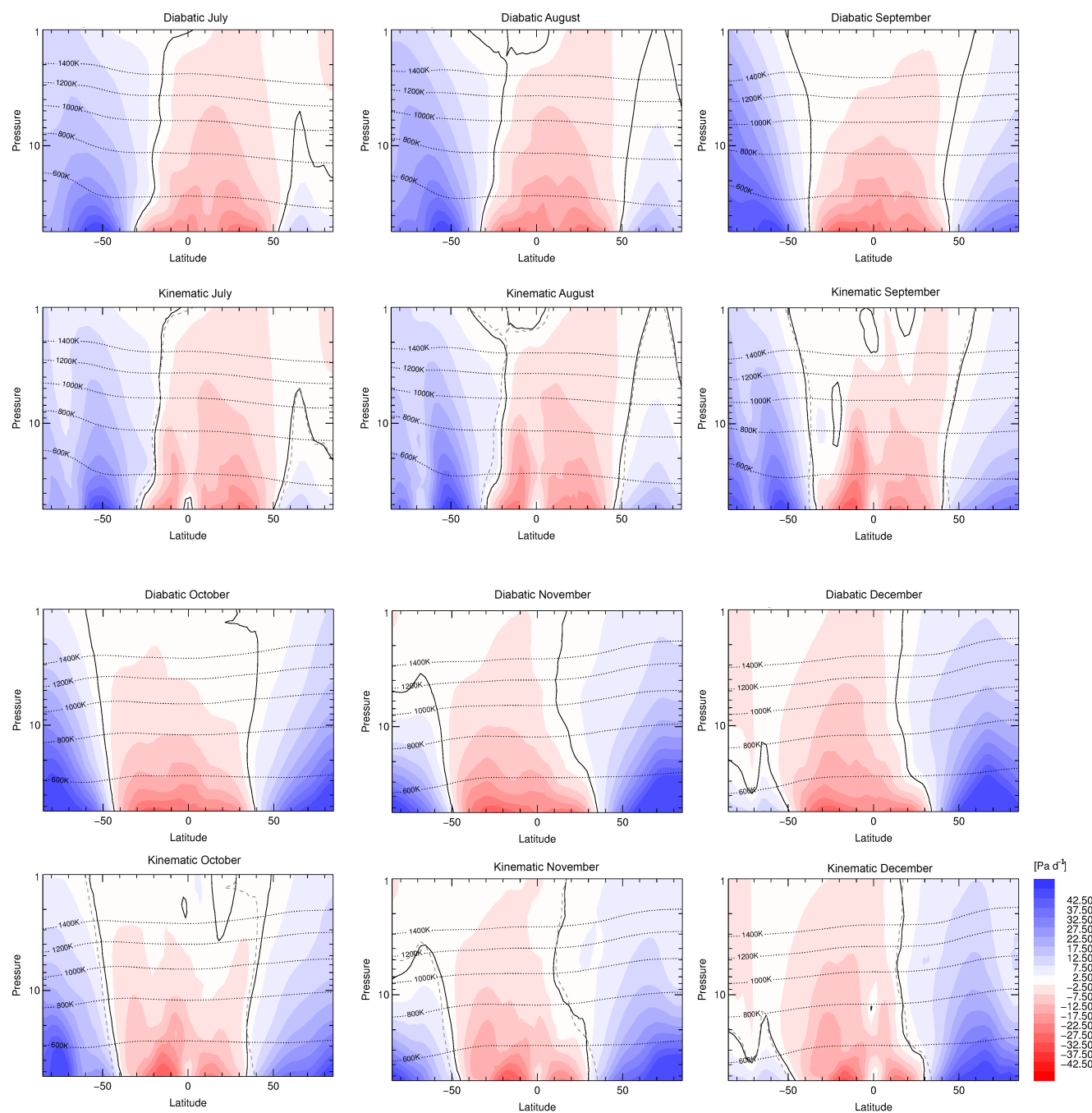
Figure B2. Vertical velocities \bar{\omega}_\theta from diabatic heating rates in ( \text{Pa day}^{-1} ) and transformed Eulerian mean (TEM) vertical velocity \bar{\omega}^* in ( \text{Pa day}^{-1} ) from the 10-year EMAC climatology for the months July–December.
