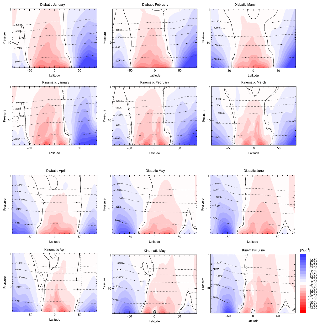
Figure B1. Vertical velocities \bar{\omega}_\theta from diabatic heating rates in (Pa day -1 ) and transformed Eulerian mean (TEM) vertical velocity \bar{\omega}^* in (Pa day -1 ) from the 10-year EMAC climatology for the months January–June.
