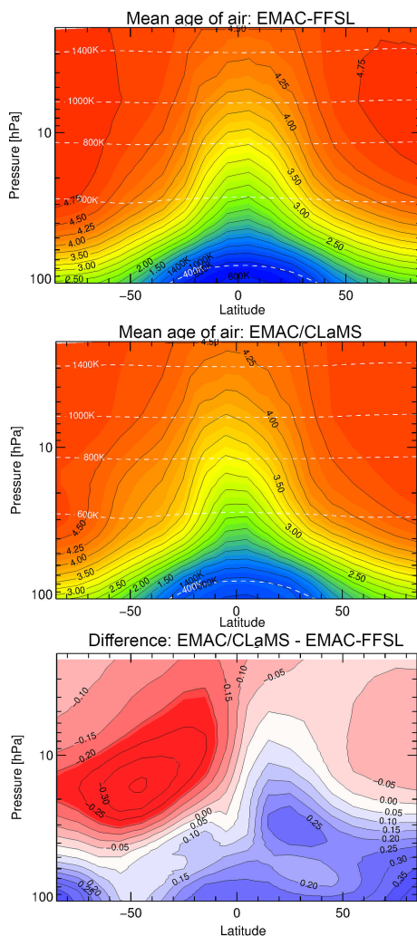
Figure 6. Annual, zonal mean age of air from 10-year climatologies for EMAC–FFSL (top panel) and EMAC–CLaMS (middle panel). Dashed lines show levels of constant potential temperature \theta . Absolute differences in age of air (EMAC–CLaMS – EMAC–FFSL) (years) are shown in the bottom panel. Blue colors indicate younger air in EMAC–FFSL, while red colors indicate younger air in EMAC–CLaMS.
