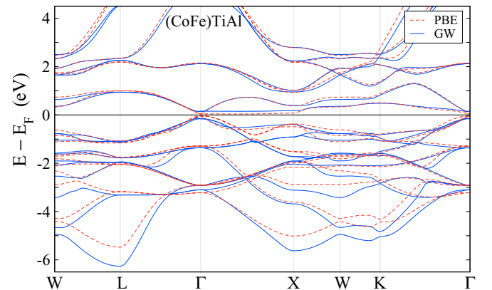
FIG. 2. Calculated electronic band structure of (CoFe)TiAl along the high-symmetry directions in the first Brillouin zone using either the PBE-GGA (red dashed line) or the GW (blue solid line) approximations.
