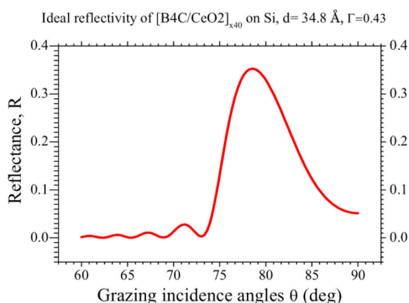
FIG. 10. Ideal reflectivity performance of B 4 C/CeO 2 ML with N = 40, d = 34.8 Å, \Gamma = 0.43 at incident photon energy of 183.82 eV (~6.75 nm).
