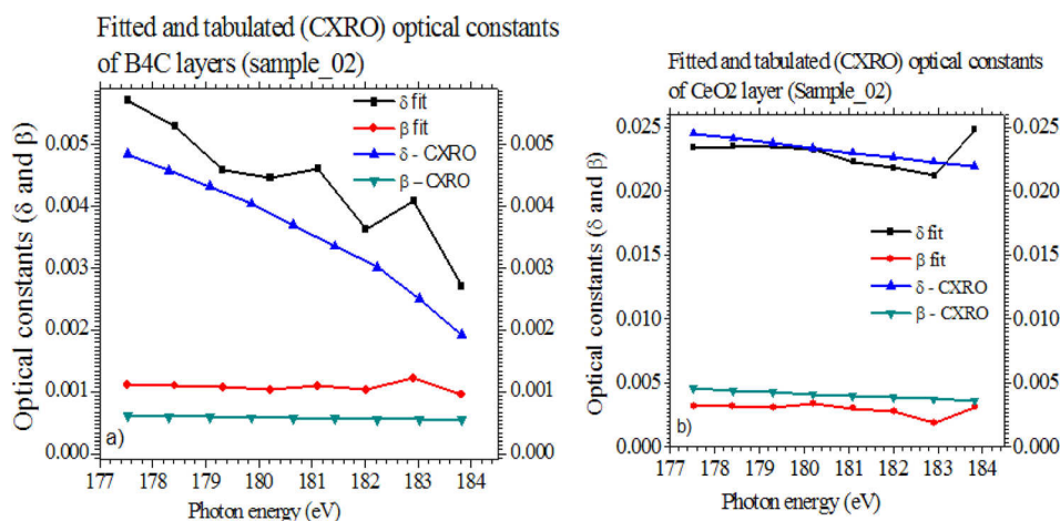
FIG. 8. Optical constants ( \delta and \beta ) retrieved from the GI-EUVR data fittings and tabulated values from CXRO database. (a) B 4 C layer and (b) CeO 2 layer. Note that optical constants of B 4 C and CeO 2 are also representative of sample_01.
