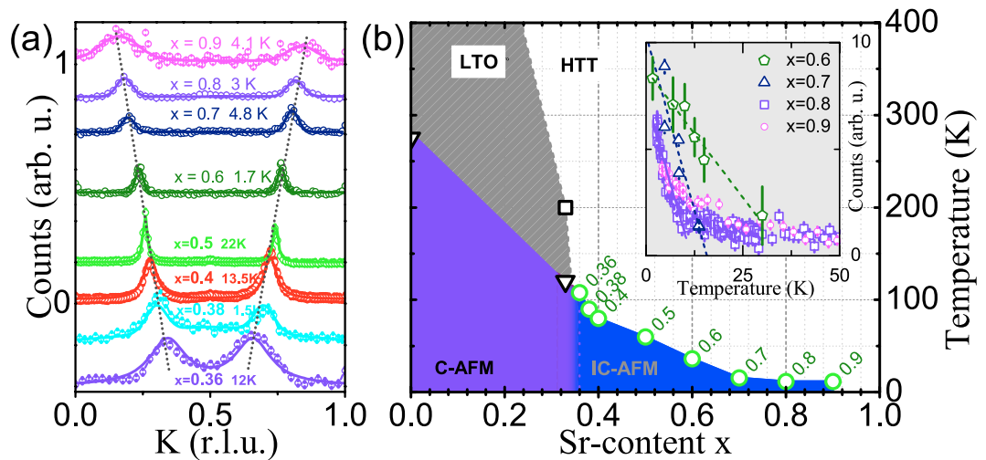
Figure 1. (a) Incommensurate magnetic peaks observed in \text{La}_{2-x}\text{Sr}_x\text{CoO}_4 within neutron scattering experiments at the 1T, 2T, IN3 and PUMA spectrometers. Diagonal (1 - K \text{ } K \text{ } 0) scans across the magnetic satellites were performed. The dotted lines follow the magnetic peak positions and act as guide to the eyes. The solid lines are fitted to the data. Sr-concentrations x and the measurement temperature are indicated. (b) Our \text{La}_{2-x}\text{Sr}_x\text{CoO}_4 phase diagram. Transition temperatures are the onset-temperatures based on the temperature-dependent neutron measurements of the elastic neutron scattering intensities shown in the inset. The data points for x \leq 0.5 were taken from 15 .
