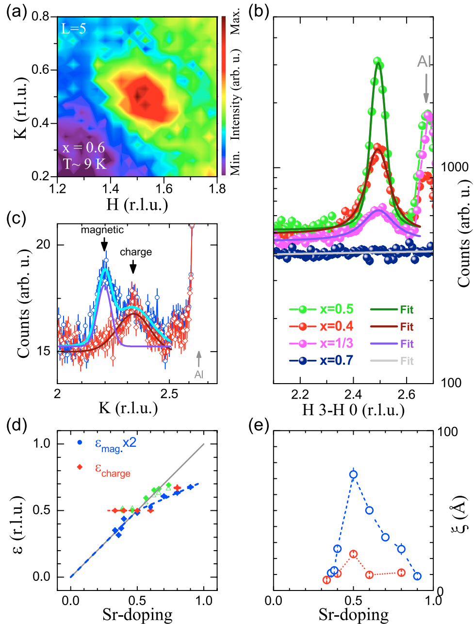
Figure 2. (a) Synchrotron radiation single crystal X-ray diffraction measurements reveal half-integer peaks in \text{La}_{1.4}\text{Sr}_{0.6}\text{CoO}_4 at \sim 9\text{ K} which are indicative for CBCO. (b) Neutron diffraction measurement of the charge correlations in \text{La}_{1.3}\text{Sr}_{0.7}\text{CoO}_4 . For direct comparison practically the same experimental conditions as for the study of the half- and underdoped cobaltates with x = 0.5, 0.4 and 1/3 published in ref. 17 were reproduced. (c) Neutron scattering intensities measured in a diagonal ( 3 - K\ K\ 0 ) scan for the sample with x = 0.8 at \sim 3\text{ K} (blue) and 100\text{ K} (red). As can be seen, the charge correlations are incommensurate at such high hole-doping. The magnetic and charge ordering peak positions at 3\text{ K} were determined by fitting two Gaussians (cyan dotted line), and they equal 2.196(3) and 2.320(15) , respectively. The charge ordering peak position at 100\text{ K} (solid magenta line) is 2.329(5) . The corresponding incommensurabilities for charge and magnetic peaks are 2 \cdot \varepsilon_{\text{mag}} = 0.608(6) , \varepsilon_{\text{charge}}(3\text{ K}) = 0.680(15) , and \varepsilon_{\text{charge}}(100\text{ K}) = 0.671(5) . (d) Sr-doping dependence of the charge and magnetic incommensurabilities, 2 \cdot \varepsilon_{\text{mag}} and \varepsilon_{\text{charge}} , respectively. Green data points are the corresponding values for \text{Pr}_{2-x}\text{Ca}_x\text{CoO}_4 taken from ref. 24; open/closed symbols: 2 \cdot \varepsilon_{\text{mag}}/\varepsilon_{\text{charge}} . (e) The correlation lengths \xi_{\parallel\vec{q}} (blue: magnetic; red: charge) for different values of x . Here, the \xi_{\perp\vec{q}} are greater than \xi_{\parallel\vec{q}} (e.g. 59(19)\% greater for x = 0.7 ). It should be noted that \xi_{\perp\vec{q}} and \xi_{\parallel\vec{q}} are defined as the correlation lengths perpendicular and parallel, respectively, to the direction of \vec{q} with incommensurate magnetic peak positions \vec{q} = \vec{Q}_{\text{mc}} - (1/2\ 1/2\ 0) and \vec{Q}_{\text{inc}} , respectively. The correlation lengths were obtained from the inverse of the (Lorentzian) peak widths. For better visibility the charge correlation lengths have been multiplied by a factor \times 3 . The dashed lines act as guide to the eyes. The data for x \leq 0.5 were taken from refs 15–17.
