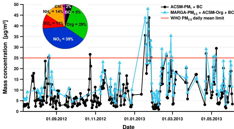
Figure 1. Time series of the daily mean. The black line represents the sum of BC and all ACSM species, the blue line the sum of BC, ACSM organics and all MARGA- \text{PM}_{2.5} species. The pie chart shows the fractional abundances of individual BC and ACSM species averaged over the whole campaign. Missing BC data was filled with zero values, thus deriving lower concentration limits.
