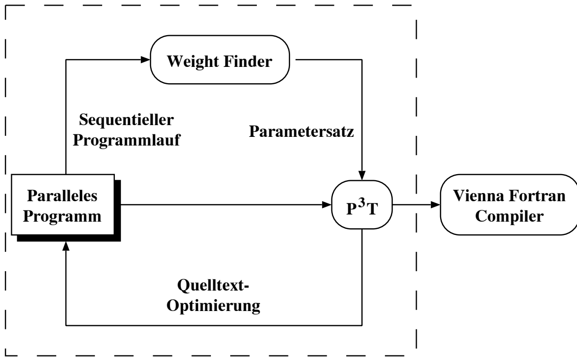
Abbildung 2.4: Parameter based Performance Prediction Tool P^3T
