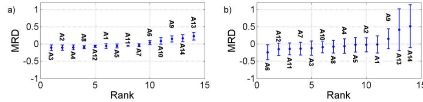
Fig. 2.12: Mean relative differences and their standard deviations for a) WaSiM-ETH relative soil moisture averaged over the extent of ASCAT pixels and b) relative ASCAT soil moisture. The numbers indicate the respective grid point IDs.
