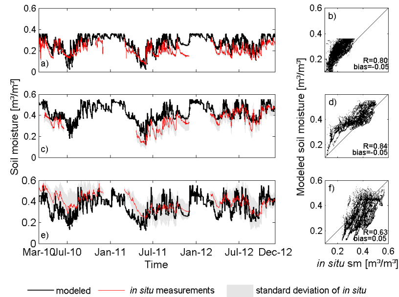
Fig. 2.2: Time series and scatterplots of in situ measurements and model results of soil moisture for a) and b) Selhausen, c) and d) Rollesbroich, e) and f) Wüstebach.
