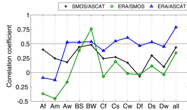
Fig. 3.5: Global correlation of ranks of MRDs of the three soil moisture products for different climate zones. The lines are just for increasing readability and do not imply any functional relationship.
