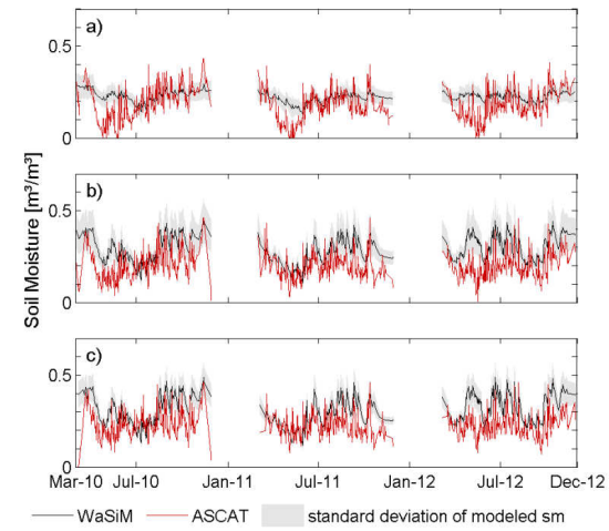
Fig. 2.4: Time series of absolute ASCAT (red) and modeled (black) soil moisture for the pixel that includes a) Selhausen, b) Rollesbroich, c) Wüstebach. Modeled soil moisture is only plotted for time steps with ASCAT observations. The grey background indicates \pm one standard deviation of the spatial averaging of modeled soil moisture.
