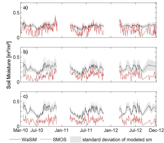
Fig. 2.3: Time series of SMOS (red) and modeled (black) soil moisture for the pixel that includes a) Selhausen, b) Rollesbroich, c) Wüstebach. Modeled soil moisture is only plotted for time steps with SMOS observations. The grey background indicates \pm one standard deviation of the spatial averaging of modeled soil moisture.
