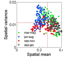
Fig. 3.8: Relationship of \bar{\theta}(t) and \sigma^2(t) for in situ measurements of SCAN in the Cf region in America.
