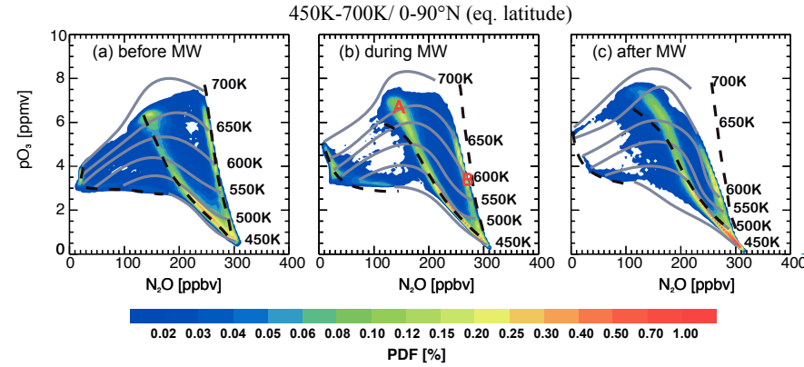
Figure 2.13: Impact of O_3 -chemistry on the temporal evolution of the N_2O - O_3 correlations. The PDFs are calculated from the N_2O - pO_3 correlations of APs with equivalent latitudes 0 – 90^\circ N and potential temperatures 450 – 700 K. The considered time periods are the same as in Fig. 2.11. The dashed black curves fit the maxima of the N_2O - O_3 correlations (PDFs) derived from a CLaMS run with a full stratospheric ozone chemistry. The correlation for passive ozone ( pO_3 ) marked as A ( N_2O near 140 ppbv and pO_3 near 7400 ppbv) and the correlation marked as B ( N_2O near 140 ppbv and pO_3 near 7400 ppbv) show clear differences from the dashed curves showing simulation with full chemistry. The two groups of APs marked by those correlation features have been investigated in more detail of their ozone chemistry (see text).
