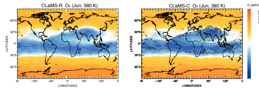
Figure 4.22: Same as Fig. 4.18 but for O_3 only in June. The relative differences up to -10\% , -20\% and -30\% are shown as the black dashed contours.
