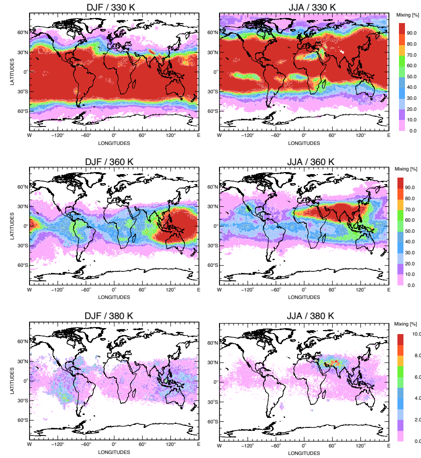
Figure 4.16: Climatology of tropospheric mixing ('state-vert') at \theta=330 K (top), \theta=360 K (middle) and \theta=380 K (bottom) in DJF (left) and in JJA (right). The intensity of tropospheric mixing is quantified as the probability (PDF) that air parcels are affected by the tropospheric mixing scheme.
