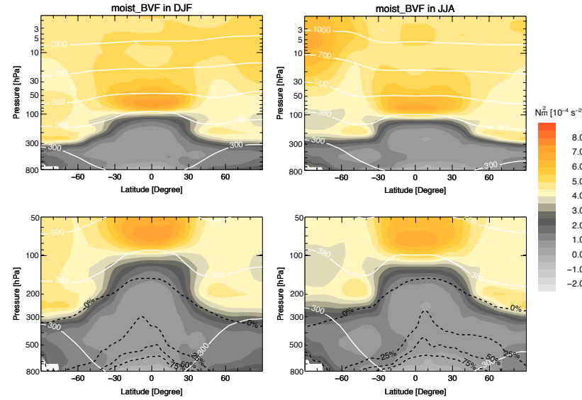
Figure 4.7: The top panel is the same as Fig. 4.1 but for moist Brunt-Väisälä frequency N_m^2 . The bottom panel is the same as top panel but the vertical range is limited in the troposphere and the lower stratosphere. The black dashed contours show the 0%, 25%, 50% and 75% relative difference to the dry Brunt-Väisälä frequency shown in Fig. 4.1.
