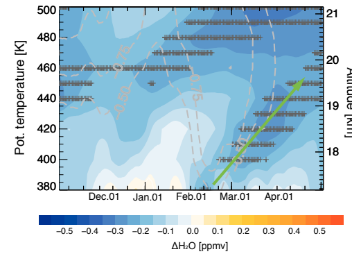
Figure 3.6: Differences of tropical ( 10^{\circ}\text{S} - 10^{\circ}\text{N} ) water vapor (colored) and temperature (gray contours) deseasonalized anomalies derived from the 35-year CLaMS simulation between winters in 2000s and winters in 1990s (2000s minus 1990s). Gray crosses indicate statistical confidence larger than 0.9 as derived from the Monte Carlo test.
