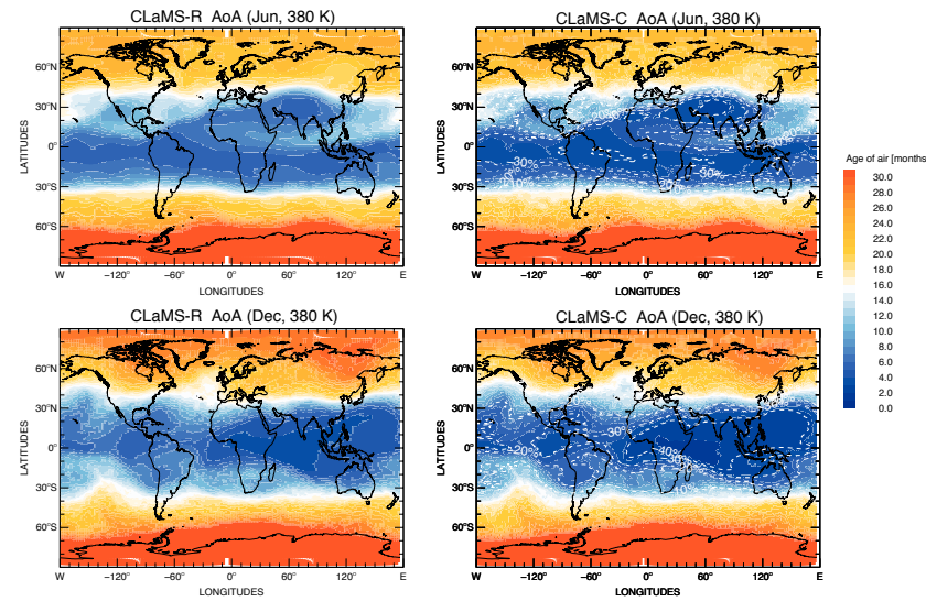
Figure 4.18: Monthly mean AoA at \theta = 380 K for CLaMS-R (left) and CLaMS-C (right) in June (top) and December (bottom). The relative differences of CLaMS-C to CLaMS-R up to -10\% , -20\% , -30\% and -40\% (CLaMS-C < CLaMS-R) are shown as the white dashed contours.
