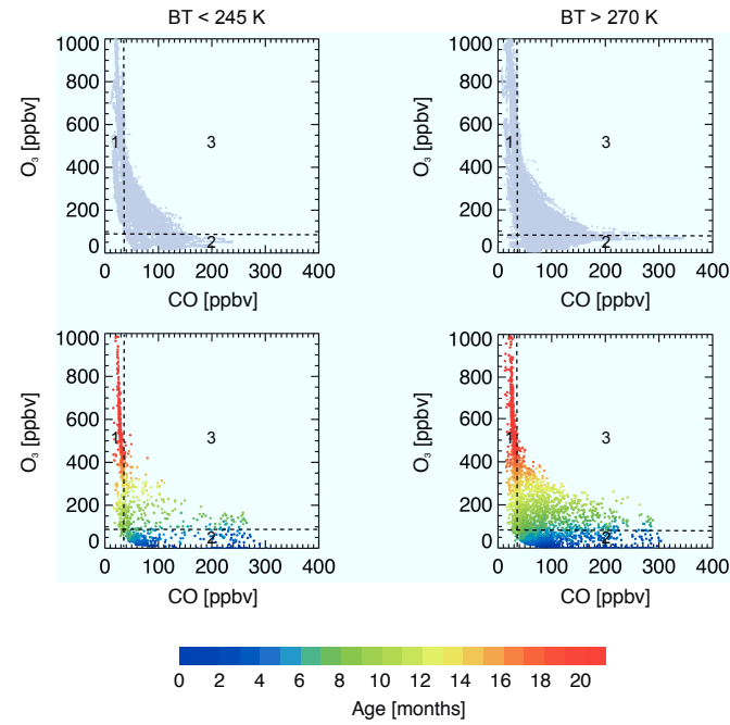
Figure 4.3: Comparison of \text{O}_3 -CO correlation of in-situ measurements (top) with the CLaMS simulation (bottom). The left panel shows all the measurements and simulation when the local brightness temperature (BT) was below 245 K; the right panel shows those when the local BT was above 270 K. The mean age of air calculated with CLaMS is color-coded in the unit of months. The BT for corresponding measurements is interpolated from the CLAUS 0.3^\circ resolution dataset. The dashed lines separate the \text{O}_3 -CO correlation space into 3 regions: area 1 (unmixed stratospheric air where \text{CO} < 35 ppbv), area 2 (unmixed tropospheric air where \text{O}_3 < 75 ppbv) and area 3 (mixed air).
