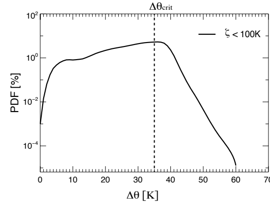
Figure 4.13: The probability distribution functions (PDFs) of \Delta\theta in the tropics ( 30^\circ\text{S} - 30^\circ\text{N} ) for the air parcels in the lowest level of CLaMS ( \zeta < 100\text{ K} \approx 2\text{ km} ) where N_m^2 is negative using the ERA-interim reanalysis data of the year 2008. The restriction used for the current ‘deep convection’ scheme ( \Delta\theta > 35\text{ K} ) is marked as the dash straight line.
