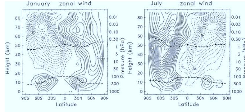
Figure 2.1: Climatological zonal mean zonal winds for (left) Jan and (right) Jul. Zonal winds are from the Unified Radio and Plasma Wave Experiment (URAP) dataset (contour interval 5 \text{ m s}^{-1} , with zero contours omitted). The heavy dashed lines denote the tropopause taken from National Centers for Environmental Prediction (NCEP) and stratopause (defined by the local temperature maximum near 50 km) (Randel et al. , 2004a).
