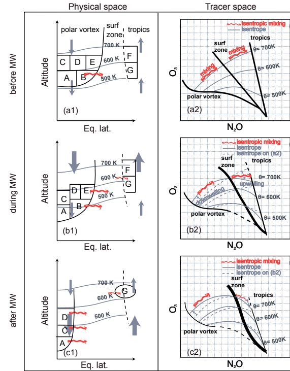
Figure 2.4: Schematic diagram of transport processes shown in physical space (left column) and tracer space ( \text{N}_2\text{O} – \text{O}_3 , right column) before (top), during (middle) and after (bottom) the major SSW. In the physical space (left column), equivalent latitudes are used as the horizontal coordinates to illustrate isentropic mixing (curved red arrows) and cross-isentropic transport (grey vertical arrows). The thickness of the grey arrows indicates the intensity of vertical motion. The characters denote exemplarily the vortex and tropical air masses which interact with the mid-latitude air. Black curves in (a2)–(c2) show respective \text{N}_2\text{O} – \text{O}_3 correlations. Grey lines denote the isentropic levels. In the tracer space, the position of isentropes before (dashed) and after (solid) the major SSW is also marked. The change of the position of a prescribed point in the tracer space along the isentropes quantifies isentropic mixing, whereas motion relative to these isentropes describes the effect of an idealized (mixing-free) cross-isentropic motion (up- or downwelling). Changes of the relative thickness of the different correlation branches mean their enhanced or weakened relative contributions to the composition of the considered part of the atmosphere (dashed lines indicate a possible missing part).
