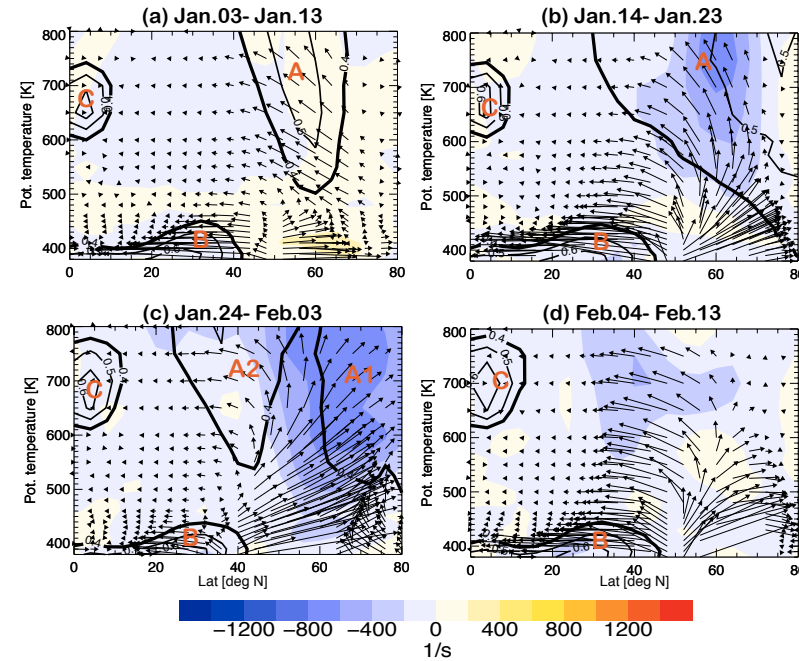
Figure 2.10: EP flux (arrows) and its divergence (coloured bluish). Black contours indicate the mixing intensity larger than 0.4. The panels (a)–(d) show mean values averaged over four time periods: (a) 3–13 January, (b) 14–23 January, (c) 24 January–3 February and (d) 4–13 February.
