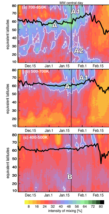
Figure 2.9: CLaMS zonal mean mixing intensity within three layers: (a) 700–850 K, (b) 500–700 K and (c) 400–500 K overlaid by the location of the vortex edge (thick black lines Nash et al. , 1996). The white contours indicate the mixing intensity of 40 %. The letters mark the regions of high mixing intensity and correspond to the letters in Fig. 2.10.
