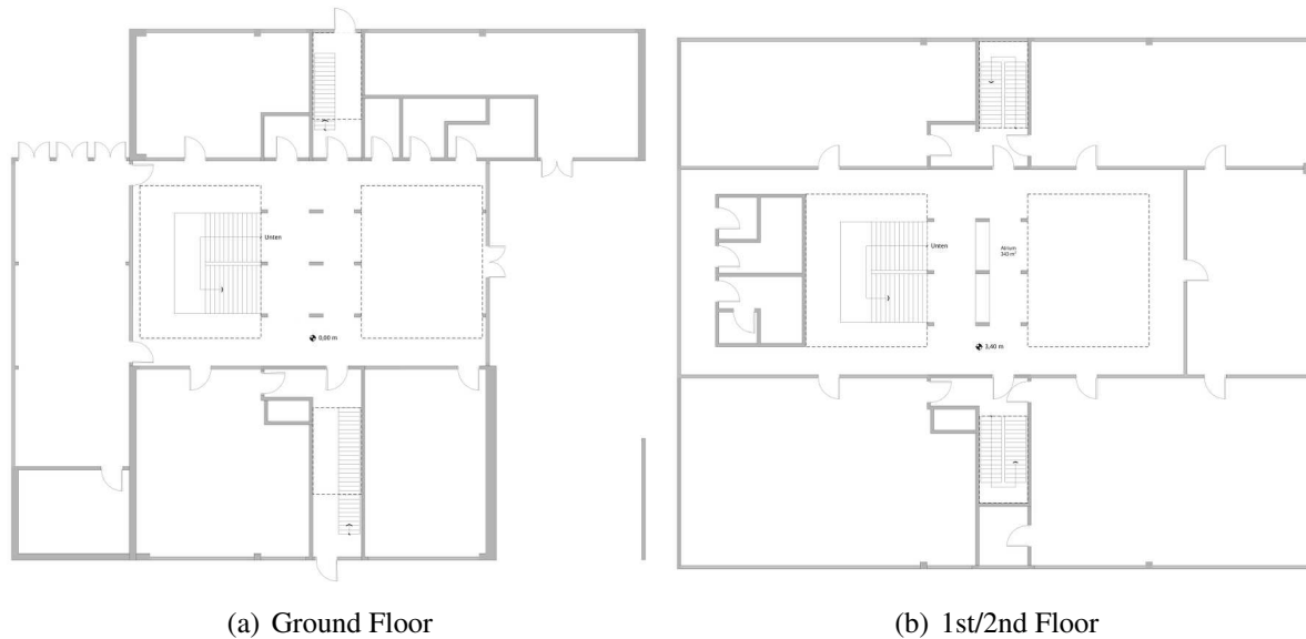
Figure 4: Floor plans of the application example consisting of the ground floor and the two overlying floors.
