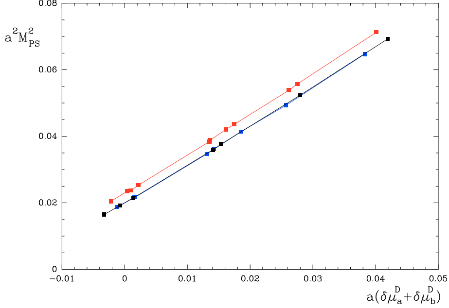
Figure 7. The same data as in figure 6, but this time plotted against Dashen-scheme quark mass.
