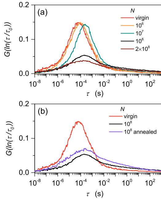
FIG. 10. Switching time distribution calculated at E_m = 4.0 kV/mm for (a) virgin and fatigued 94BNT-6BT + Cu specimens with different level of fatigue N and (b) specimens with N = 10^8 right after fatigue and after fatigue with consecutive annealing for 24 h in air at 400 °C as indicated.
