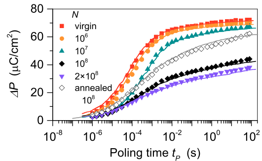
FIG. 9. Switching response at E_m = 4.0\text{ kV/mm} in virgin and fatigued 94BNT-6BT + Cu ceramic as indicated as well as in an annealed sample. Symbols correspond to the experimental results, while solid lines display the IFM-model calculations.
