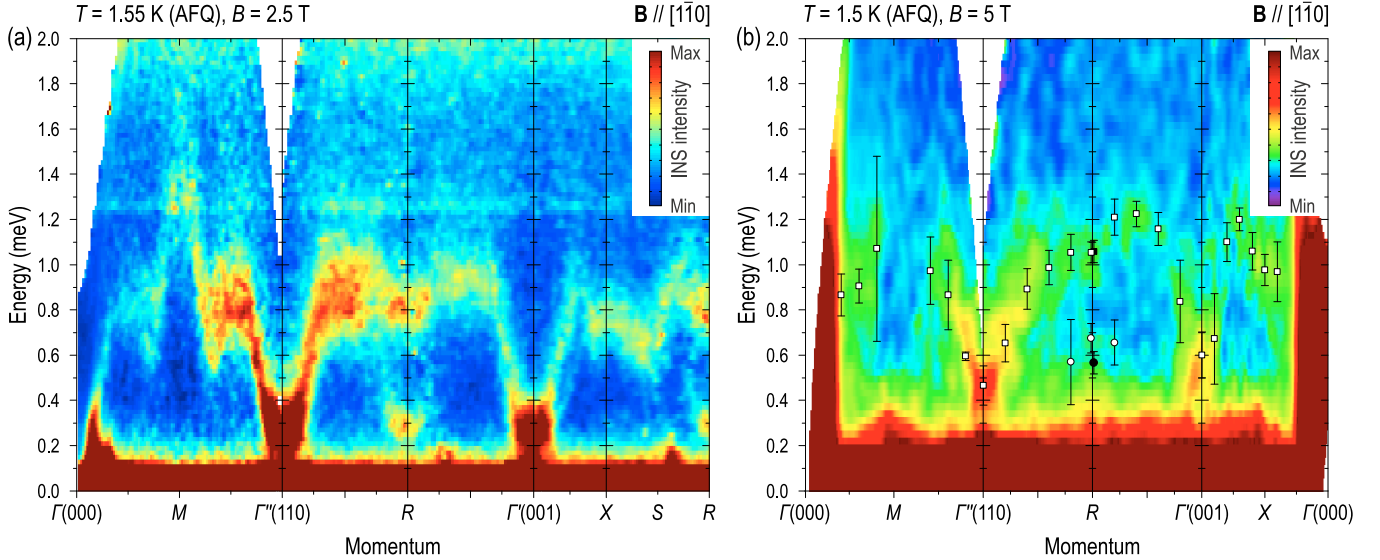
Fig. 2 (color online). Energy-momentum profiles along high-symmetry directions in the AFQ state: (a) B = 2.5 T, (b) B = 5 T. Open markers are determined as peak maxima from the fits. Solid markers at the R(\frac{1}{2}\frac{1}{2}\frac{1}{2}) point were obtained from the interpolation of peak positions from Ref. 22. Background contamination from the He exchange gas was subtracted from the data in panel (b), as explained in the Supplemental Material [46]. Because of the high-level background coming from the magnet, the field-induced low-energy magnetic excitation cannot be clearly resolved at this field.
