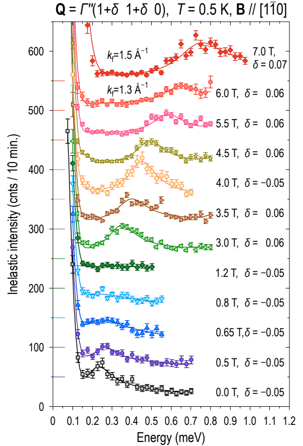
Fig. 1 (color online). INS spectra measured near the zone center \Gamma''(110) at a slightly incommensurate wave vector as indicated in the legend, to avoid contamination from the Bragg tail. The spectra are shifted vertically for clarity with horizontal lines at the left indicating the background baseline for each spectrum. Solid lines represent Lorentzian fits on top of a nonmagnetic background.
