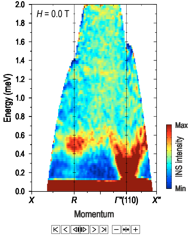
Fig. S1. Animation illustrating magnetic field dependence of the magnon spectrum along high-symmetry directions in \text{CeB}_6 . Each frame consists of three color maps integrated along straight segments connecting the X(00\frac{1}{2}) , R(\frac{1}{2}\frac{1}{2}\frac{1}{2}) , \Gamma''(110) , and X''(11\frac{1}{2}) points, which we combined to form a continuous polygonal path in reciprocal space. The controls at the bottom of the figure can be used to modify the frame rate, pause the animation, or browse through individual frames.
