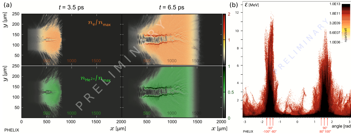
Figure 1: EPOCH-simulated data (PHELIX): (a) Temporal evolution of the normalized electron- and ^4\text{He}^{2+} ion-number densities for t = 3.5 \text{ ps} (left column) and t = 6.5 \text{ ps} (right column) after the laser pulse entered the simulation box at the left boundary. (b) Angular \text{He}^{2+} ion-energy distribution for t = 6.5 \text{ ps} .
