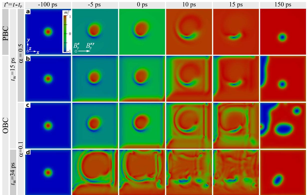
Figure 2. Snapshots of the system during the dynamical switching induced by a single magnetic field pulse: The color represents the out-of-plane component of the magnetization, m_z^i in the top atomic layer at each lattice site for the simulated domain of 100 \times 100 \times 3 spins. The coordinate system and the color map for m_z^i are shown in the initial snapshot of panel a. The sequence of the snapshots in (a) corresponds to periodic boundary conditions (PBC) in the xy -plane, while in (b–d) open boundary conditions (OBC) are used. The magnetic field pulse of amplitude B_0 = 1 T is applied along the direction defined by \theta = 50^\circ and \varphi = 0^\circ . The pulse width t_w = 15 ps, and 34 ps, damping parameter \alpha = 0.5 and 0.1 as marked on the left panel of the figure, see also open circles in Fig. 6. For these simulations the coupling constants have been fixed to J = 0.5 meV/atom, K/J = 0.2 , D/J = 0.24 .
