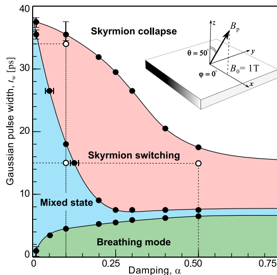
Figure 6. Switching diagram for square domain in terms of damping \alpha and magnetic pulse width t_w : Each area corresponds to the regime of excitation: breathing mode (green), skyrmion switching (red), mixed state (blue) and skyrmion collapse (white). Open circles correspond to the parameters used for the simulations illustrated by the snapshots in Fig. 2.
