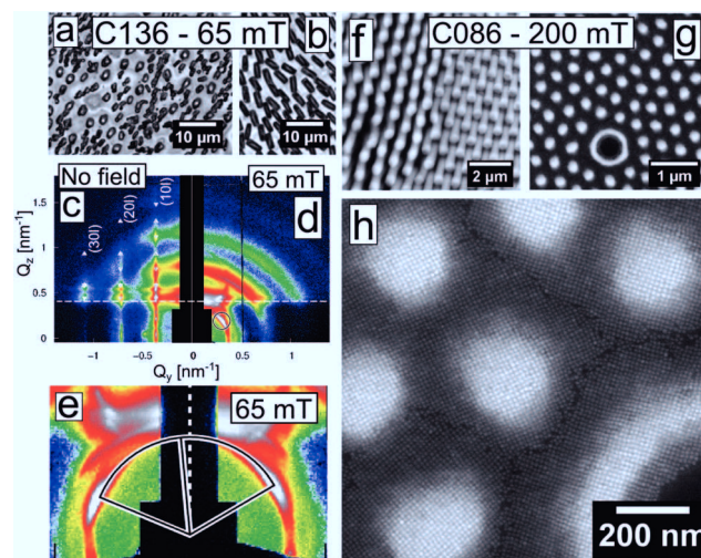
Fig. 6 Ferrohydrodynamic instabilities in nanocube assemblies. Light microscopy image showing (a) arrays of oriented mesocrystals and (b) collapsed pillars composed of C136 nanocubes assembled in a field of \mu_0 H_{\text{app}} = 65 mT. GISAXS patterns of C136 assembled under (c) zero field, indexed to a sc lattice and (d) under a magnetic field of \mu_0 H_{\text{app}} = 65 mT, destroying the mesoscale ordering with respect to the substrate reference plane. One reflection of the SAXS component is highlighted beneath the Yoneda line. (e) Detail of the central portion of the SAXS component shown in (d). The tilt angle ( \approx 5^\circ ) relative to the substrate is highlighted. (f–h) Assemblies of C086 in a strong magnetic field ( \mu_0 H_{\text{app}} = 200 mT). Hexagonal array of (f) longer pillars and (g) protrusions composed of nanocubes. A toroidal nanocube structure can be seen in (g). (h) A magnified portion of the area in (g), showing the ordering in the torus and the protrusions near the substrate surface. Note that the centre of the torus is devoid of nanocubes.
