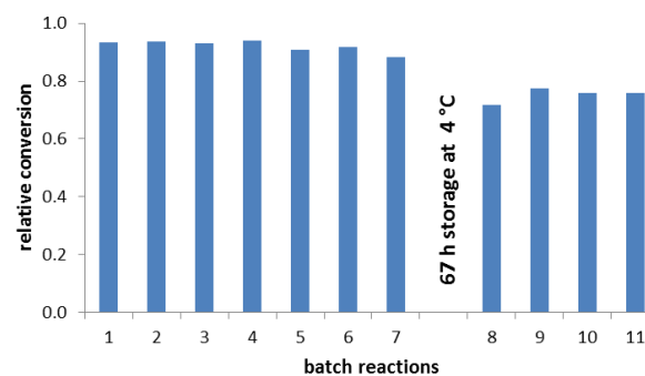
Figure 39: Repetitive batches for the formation of 2-Cl-Phe with AtPAL2-CBM immobilized on Avicel. Reaction conditions: 22 mM 2-Cl-CA in 2.5 M (\text{NH}_4)_2\text{CO}_3 , pH 8.9, 30 °C, 0.5 g Avicel with about 5.1 mg immobilized AtPAL2-CBM, 10 ml volume, 1 h reaction time, single measurements.
