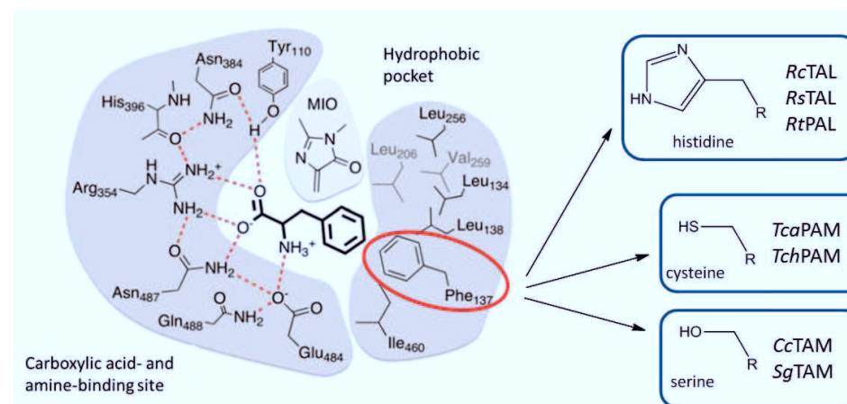
Figure 11: Active site of PcPAL with bound substrate L-Phe (adapted from [80] ) and differences in the selectivity switch region (Phe 137) in other MIO-dependent wt enzymes.
