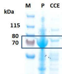
Figure 47: Pellet fraction (P) and CCE after sonification of 1.5 g wet E. coli cells containing CcTAM K2E-CBM in 5 ml Tris-HCl buffer, 10 x 30 s sonification on ice, centrifugation; 1 \mu l sample, 12 \mu l buffer, 5 \mu l NuPage LDS Sample Buffer 4x, 2 \mu l NuPage Reducing Agent 10x; 2 min 99°C, 10 \mu l loaded onto gel; 200 V, 100 mM 15 W, 60 min; 1 h in Coomassie staining, destaining in water.
