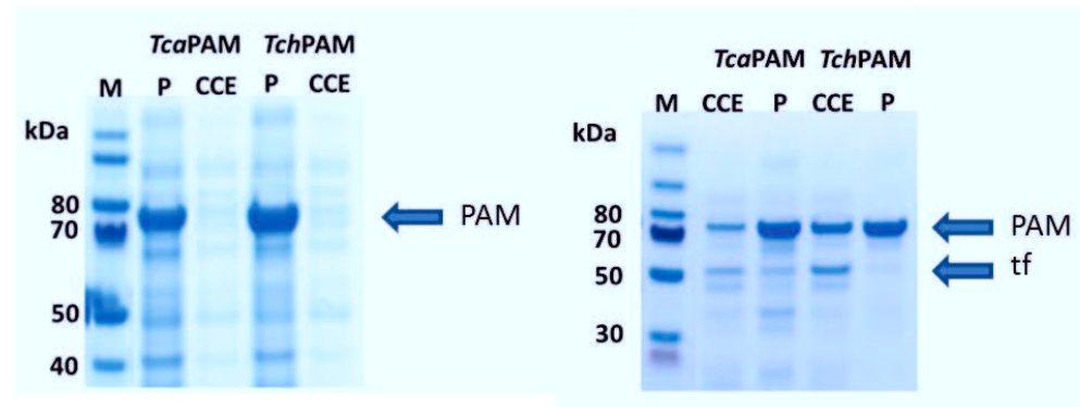
Figure 19: SDS-PAGE analysis of soluble and insoluble fractions after PAM gene expression without chaperones (left) and after coexpression with chaperone 5 containing the trigger factor (tf) (right). Analysis conditions see 3.3.3 and 3.4.1, Marker: PAGE PageRuler™ (Plus) Prestained Protein Ladder. CCE: crude cell extract; P: pellet after disruption. Tca PAM: 77.6 kDa, Tch PAM: 76.4 kDa, trigger factor: around 56 kDa.
