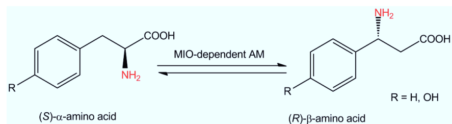
Figure 12: Physiological reaction of MIO-dependent aminomutases [84] . The stereochemistry of the \beta -amino acid depends on the enzyme used and can also be S -selective.
