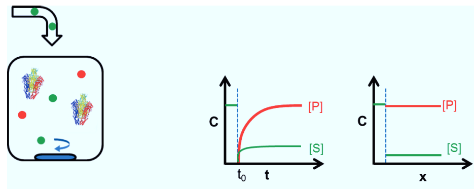
Figure 3: Schematic presentation of a fed-batch reactor using isolated enzyme (left) and respective time- and space dependent concentration profiles (right). t: time, C: concentration, x: space, [P] product concentration (red), [S] substrate concentration (green).
