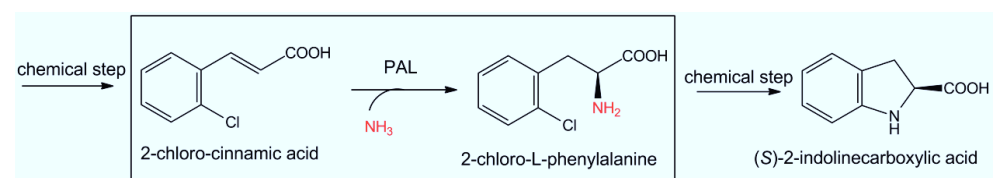
Figure 13: Process for the production of (S)-2-indolinecarboxylic acid by DSM
