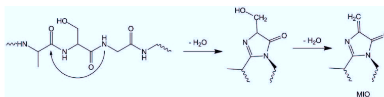
Figure 8: Formation of the MIO prosthetic group (adapted from [71] ).
