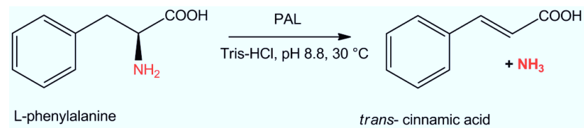
Figure 14: Deamination of L-phenylalanine to trans -cinnamic acid catalyzed by PALs.
