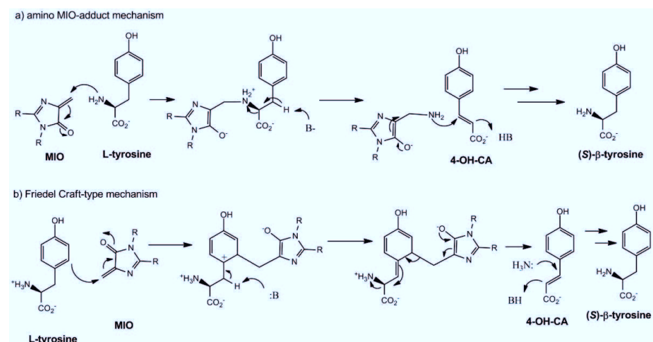
Figure 9: Proposed reaction mechanisms for MIO-enzymes (adapted from [74] )
