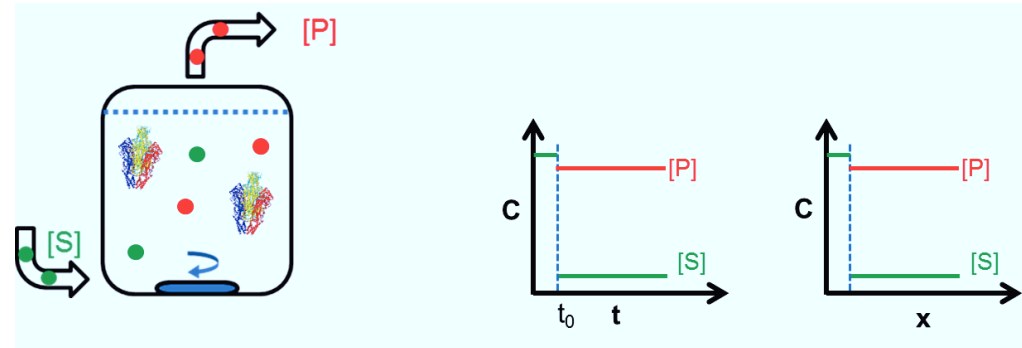
Figure 4: Schematic presentation of an enzyme membrane reactor using isolated enzyme. The biocatalyst is retained by a membrane (left, dotted line) and respective time- and space dependent concentration profiles (right). t : time, C : concentration, x : space, [P] product concentration (red), [S] substrate concentration (green).
