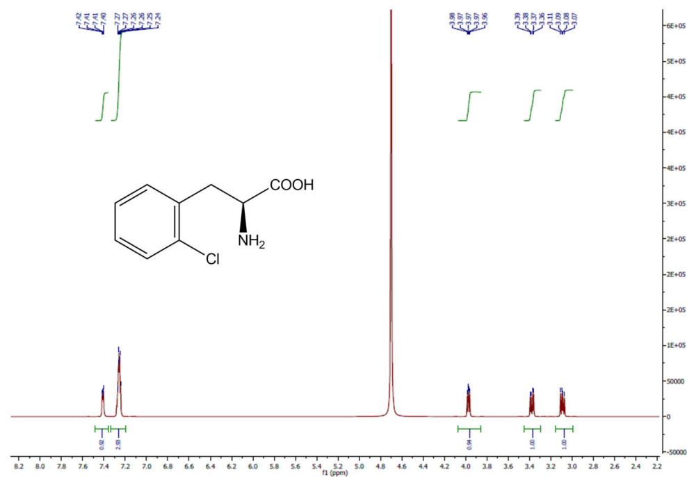
Figure 17: ^1\text{H-NMR} (600 MHz, \text{D}_2\text{O} ) of 2-Cl-L-Phe: \delta = 3.08 (dd, J = 14.4, 8.71 , 1 H, \text{CH}_2 ), 3.37 (dd, J = 14.4, 6.1 , 1 H, \text{CH}_2 ), 3.97 (m, 1 H, CH), 7.24-7.27 (m, 3 H, CH), 7.40-7.42 (m, 1 H, CH).
