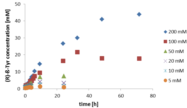
Figure 51: (R)-β-Tyr formation from 4-OH-CA with whole cells containing CcTAM . Reaction conditions: 5 - 200 mM 4-OH-CA in 2.5 M (NH 4 ) 2 CO 3 , pH 8.9, 30 °C, 1 ml volume, 1200 rpm, cell load: 100 mg/ml.
