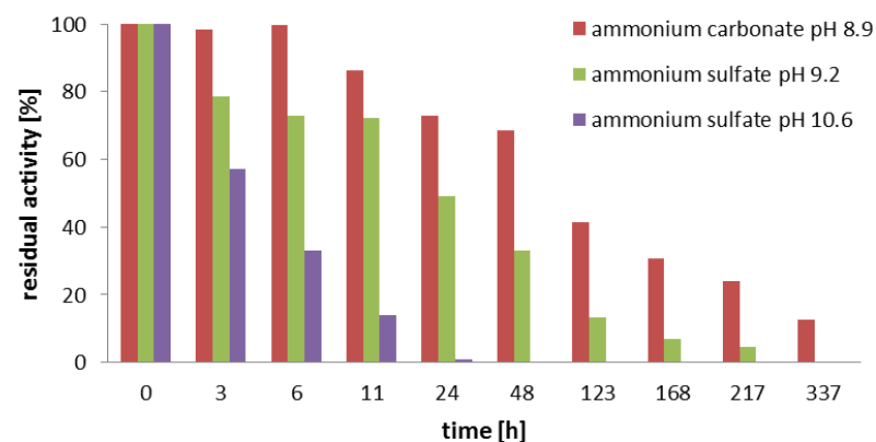
Figure 25: Residual volumetric activity after incubation of At PAL2 in ammonium carbonate (pH 8.9) and ammonium sulfate (pH 9.2 or pH 10.6). Incubation conditions: 8-9 mg lyophilized enzyme in 1.5 ml of the respective buffer at 30 °C and 300 rpm. At each time point samples were taken and transferred to a 1 cm cuvette to follow the deamination of L-Phe (3.4.3.1). The volumetric activity at the beginning was set to 100 %.
