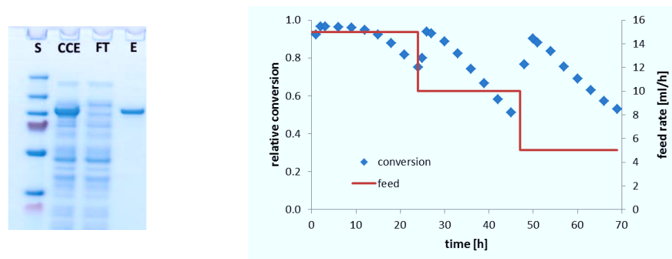
Figure 42: Left: SDS PAGE analysis of AtPAL2-CBM binding to an Avicel filled column reactor, 6.5 \mu\text{g} of each fraction was applied to the SDS gel, S: PageRuler Prestained Plus Protein Ladder, CCE: crude cell extract, FT: flow through, E: elution fraction with deionized water. Right: Relative conversion and feed rate in the amination of 2-Cl-CA in a plug-flow reactor (XK 16/20 chromatography column, 20 cm x 1.6 cm). Reaction conditions: 25 mM 2-Cl-CA in 2.5 M (\text{NH}_4)_2\text{CO}_3 , pH 8.9, 30 ^\circ\text{C} , 1 g Avicel with 10.1 mg immobilized AtPAL2-CBM, flow rate 15-5 ml/h (right picture). Product formation was tracked with HPLC (3.4.4.1), single measurements.
