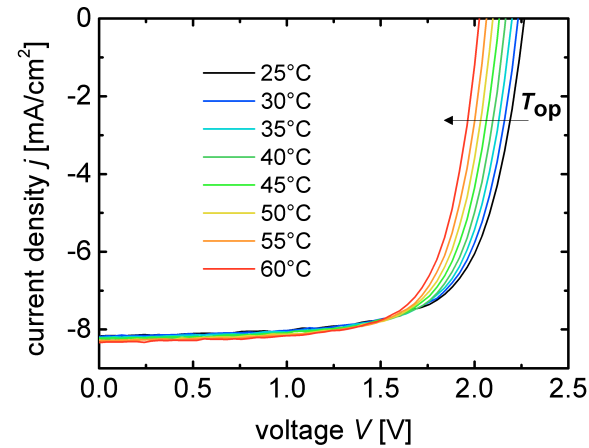
Fig. 5.18 Current density-voltage j - V curves of the a-Si:H/a-Si:H/ \mu c-Si:H triple junction solar cell at various operating temperatures T_{\text{op}} . The temperature range between 25 °C and 60 °C was investigated in steps of 5 °C.
