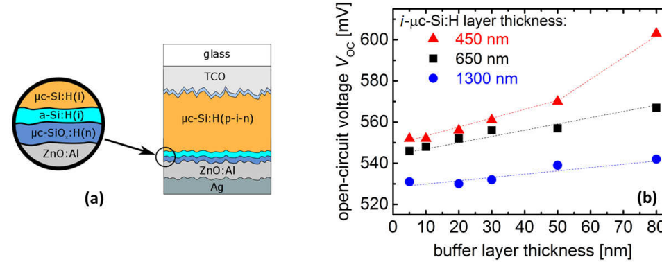
Fig. 5.7 (a) Schematic drawing of the \mu\text{c-Si:H} solar cell with the incorporated n-i buffer layer. (b) Open-circuit voltage V_{OC} of \mu\text{c-Si:H} solar cells as a function of n-i buffer layer thickness (5, 10, 20, 30, 50, 80 nm) for different intrinsic \mu\text{c-Si:H} absorber layer thicknesses (blue circles: 1300 nm, black squares: 650 nm, red triangles: 450 nm). All absorber layers were deposited at SC = 5\% . The maximum error in the V_{OC} determination is below 5 mV.
