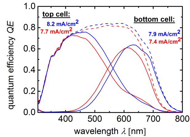
Fig. 5.12 Quantum efficiency measurements of the 130/180 and of the 130/130 a-Si:H/a-Si:H tandem junction solar cells from Table 5.3, respectively. The photocurrent densities of the top and bottom cell, J_{QE,top} and J_{QE,bot} are calculated from the QE curves and placed near the related measurements.
