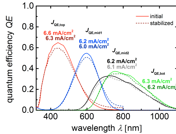
Fig. 5.17 Quantum efficiency measurement of a-Si:H/a-Si:H/ \mu\text{c-Si:H} / \mu\text{c-Si:H} quadruple junction devices corresponding to cell Q3 from Table 5.6 in initial and stabilised state (after 1000 hours light soaking time). Initial sub cell photocurrent densities calculated from the QE curves are placed near the related measurements.
