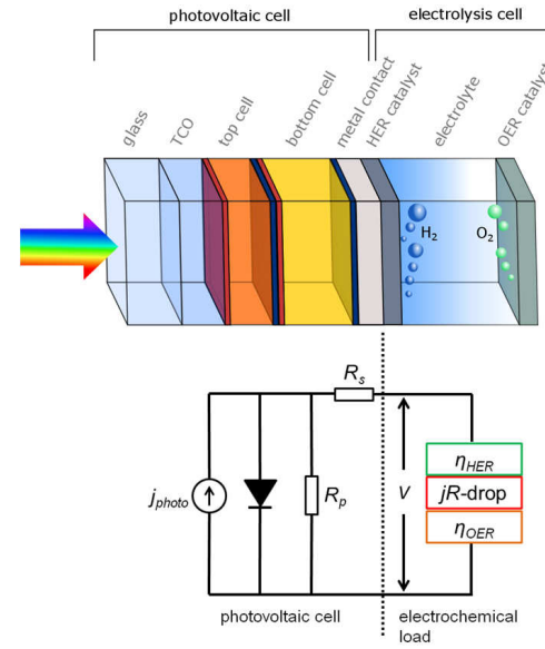
Fig. 4.3 Schematic drawing of a tandem junction based PV-EC device with its photovoltaic and electrochemical components. Below, the equivalent circuit used to model the PV-EC device is depicted. The photovoltaic cell is connected in series with the electrolysis cell, which represents the electrochemical load of this device, including the current-dependent overpotentials for the HER and OER, \eta_{\text{HER}}(j) and \eta_{\text{OER}}(j) respectively, and the electrolyte ohmic drop jR . The photocurrent density j_{\text{photo}} is generated by the photovoltaic cell. The parallel and the shunt resistances of the photovoltaic cell are denoted by R_p and by R_s , respectively.
