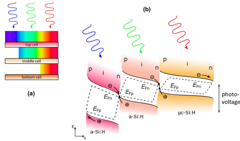
Fig. 2.6 (a) Illustration of the spectral distribution in a multijunction solar cell structure, for the example of a triple junction cell. (b) Band diagram of a pin multijunction solar cell under illuminated conditions (as an example a triple junction solar cell is shown). Holes and electrons from the a-Si:H top and middle cell, and the \mu\text{c-Si:H} bottom cell, respectively, have to recombine at the n -/ p -interfaces to ensure a continuous current. The interfaces are called recombination junctions. The sum of the splitting of the quasi-Fermi levels E_{Fn} and E_{Fp} of the top, middle and bottom cell defines the photovoltage of the multijunction cell.
