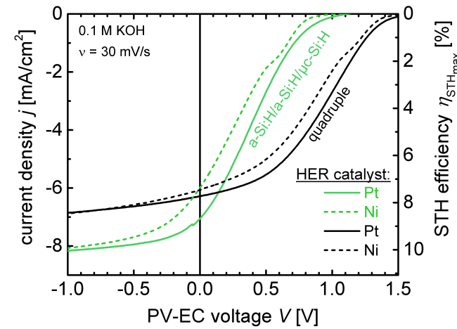
Fig. 6.6 Linear sweep voltammetry measurements of PV-EC devices based on a-Si:H/a-Si:H/ \mu c-Si:H triple and quadruple junction photocathodes with a \text{RuO}_2 counter electrode for the OER reaction. For the HER reaction, 150 nm of Ni (dotted curves) and Pt (solid curves) were deposited on top of the Ag solar cell contacts, respectively. The measurements were conducted in 0.1 M KOH at 30 mV/s. The right ordinate depicts the achievable STH efficiency as a function of the photocurrent density at 0 V (see Eq. 4.4).
