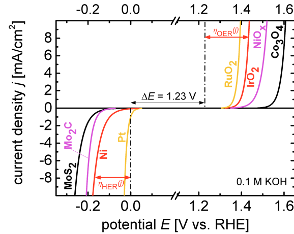
Fig. 6.12 Modeled current density-voltage curves of the HER and OER catalysts considered in this section. The curves were computed via Eq. 2.14 using the Tafel parameters provided in Table 6.3. As example, the overpotentials for Ni ( \eta_{\text{HER}}(j) ) and for \text{IrO}_2 ( \eta_{\text{OER}}(j) ) are indicated.
