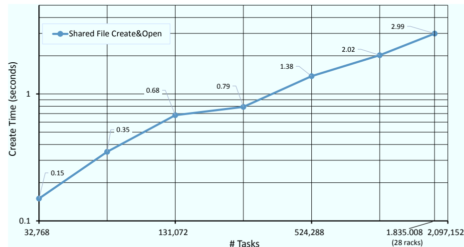
Figure 4.3: Creating and opening SIONlib container file in parallel on JUQUEEN with one file per I/O-bridge node.
