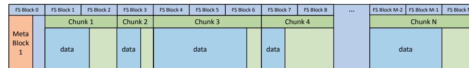
Figure 3.8: Simple and preliminary structure of the SIONlib file container. The chunks are assigned to the application tasks and their size is extended to be aligned to file-system blocks. The metadata block stores information about chunk sizes and fill rates.
