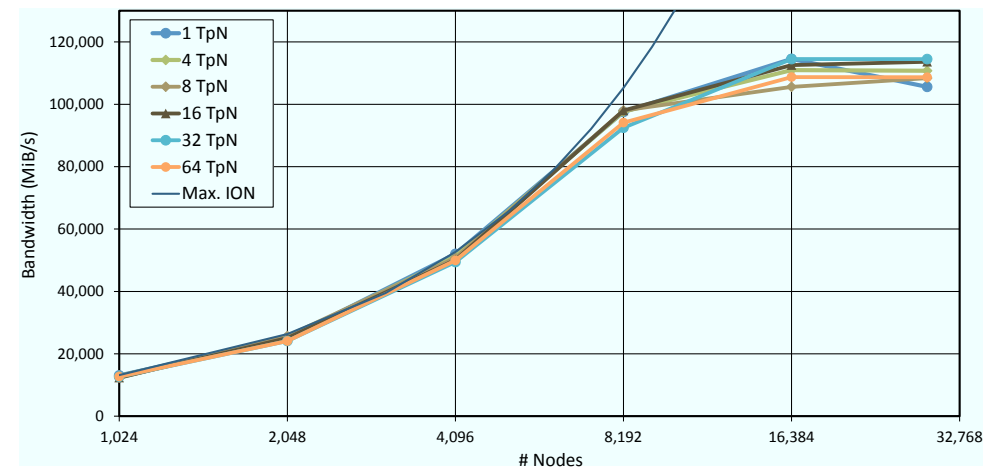
Figure 4.12: Comparison of write bandwidth on JUQUEEN for different number of tasks per node (TpN). 'Max. ION' shows the maximum I/O bandwidth, which can be achieved by that number of nodes (1-64 tasks per node, 256 MiB file data per node).
