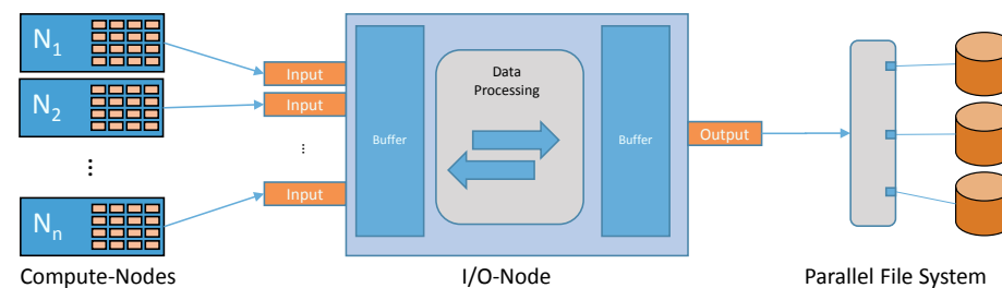
Figure 2.1: Abstract model of a simple I/O infrastructure.
