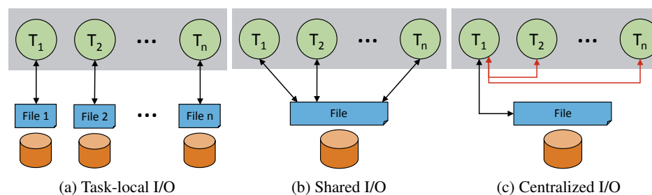
Figure 1.3: Different parallel I/O approaches, using individual files per task or a shared file.
