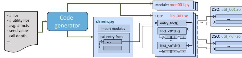
Figure 6.2: The Pynamic code generator creates the Python driver script and the DSOs. In addition, Pynamic generates also a set of utility libraries. Their functions will be called randomly from the functions of the DSOs.
