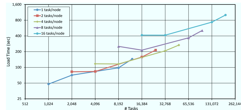
Figure 2.10: Load times of a dynamically linked application on Blue Gene/Q system JUQUEEN for different number of tasks per compute node and scaled up to a size of twelve racks using an NFS file system.
