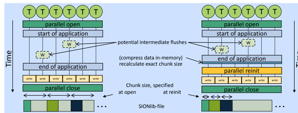
Figure 3.14: Example of using the SIONlib reinit feature in Scalasca. The instrumented application records event traces in memory buffers. The use of the SIONlib reinit function reduces the chunk size of the forehandedly opened file to the actual required sizes (right) compared to the original scheme (left).
