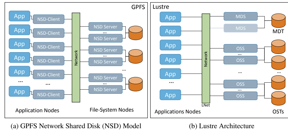
Figure 1.6: General structure of GPFS and Lustre.
