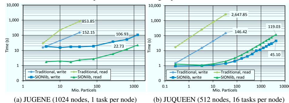
Figure 4.17: Time needed by MP2C for writing and reading restart files at small scale on JUGENE and JUQUEEN with and without using SIONlib.
