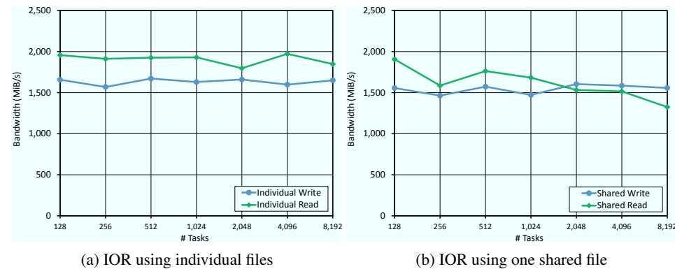
Figure 4.4: Baseline measurement with tasks using one I/O node on JUQUEEN with IOR (1-64 tasks per node, 2 GiB file data per node).
