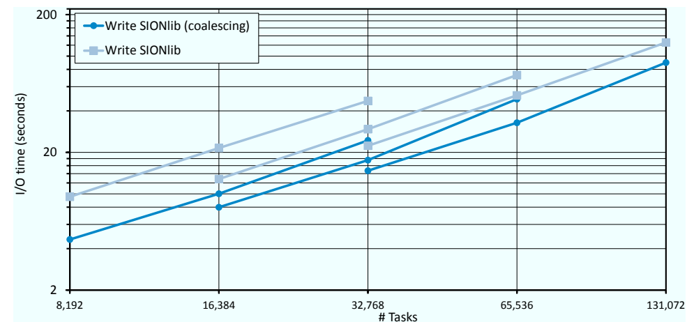
Figure 4.22: I/O timings for Scalasca's trace-file generation using standard SIONlib support and using SIONlib support with coalescing I/O. The tests were repeated for different number of tasks per node on one midplane, on one rack, and on two racks of JUQUEEN (3 curves, 16-64 tasks per node).
