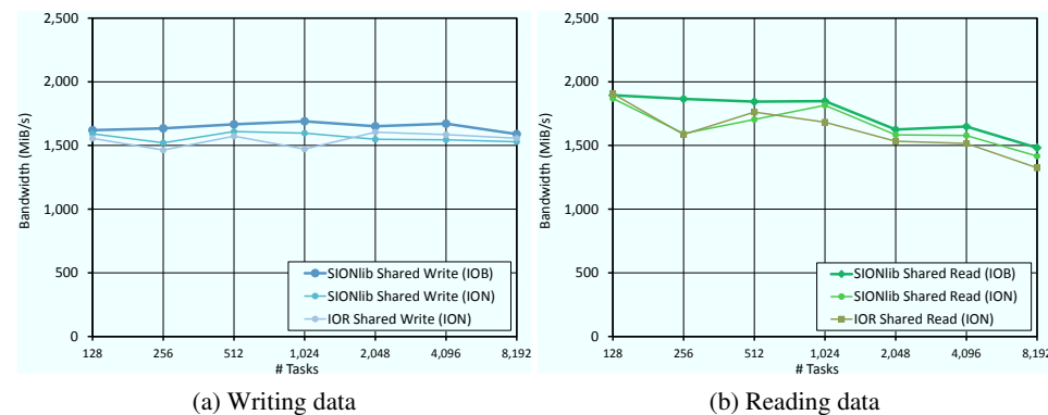
Figure 4.6: Comparison of IOR and SIONlib, including the SIONlib's multi-file approach (IOB) for baseline measurement with tasks using one I/O node on JUQUEEN (1-64 tasks per node, 2 GiB file data per node).
