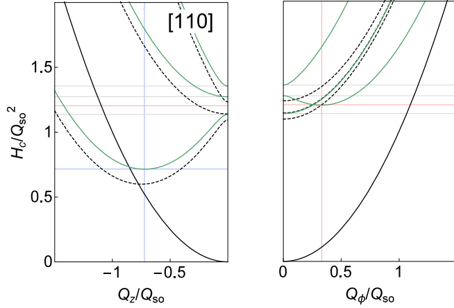
FIG. 4. Spectrum of the Cooperon Hamiltonian for [110] nanowires with parameter configurations \lambda_1 = 0.3 and \lambda_2 = 0.1 for B = \kappa = 0 (green). Dashed lines correspond to vanishing Rashba SOC and black solid line to the singlet mode. The grid lines are plotted by use of the approximate formulas \Delta_\chi^{[110]} (gray), \delta_\phi^{[110]} for Q_\phi^{\min,[110]} (red), and \delta_z^{[110]} for Q_z^{\min,[110]} (blue). The grid lines are plotted using the approximate formulas derived in Sec. III B 2.
