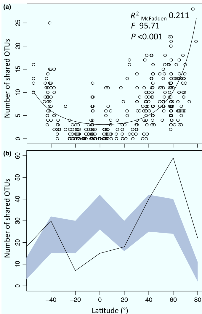
Figure 1 Fungal operational taxonomic units (OTUs) shared between Antarctica and comparison sites across different latitudes. Negative values on the x-axis denote latitudes south of the equator. (a) The relationship between the number of fungal OTUs shared with the Antarctic sites and latitude of comparison sites. (b) The observed (black line) and expected number of fungal OTUs shared with Antarctic sites at different latitudinal ranges (see Table S3). The shaded area shows the 95% confidence set of shared fungi from a distribution of 1000 randomly assembled Antarctic communities. The scales of the y-axes differ between the two plots as (a) shows the number of fungi shared with individual sites, and (b) shows the total number of fungi shared with all sites within a latitudinal range.
