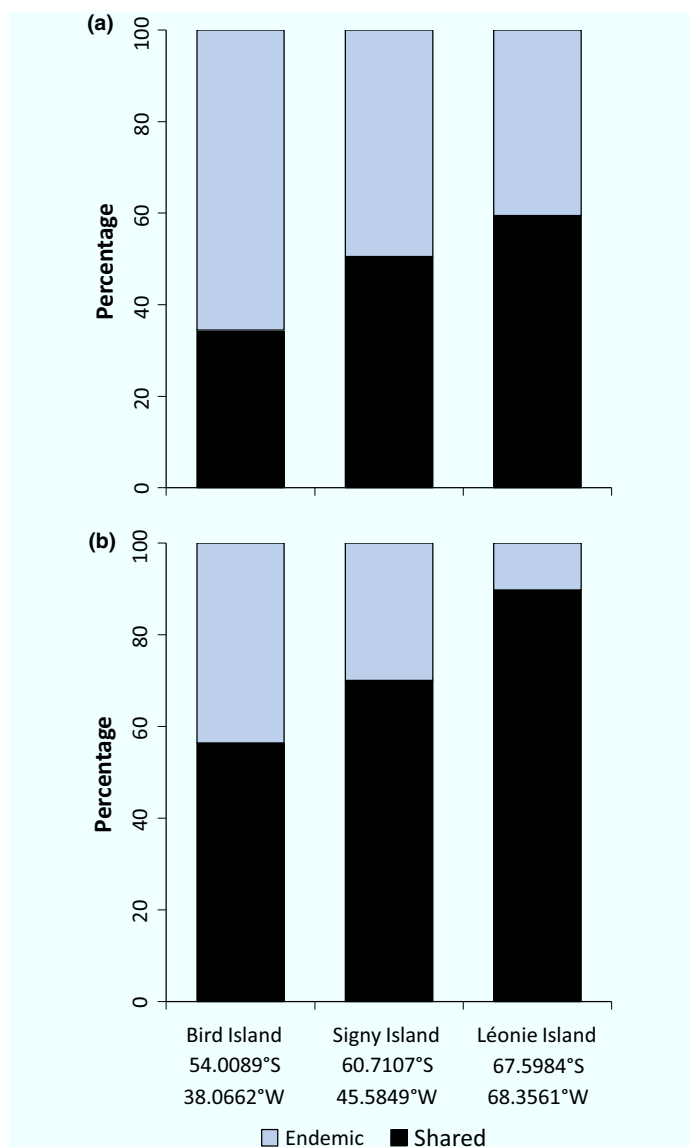
Figure 2 Percentage of Antarctic fungal operational taxonomic units (OTUs) that were endemic to Antarctica or shared with other regions of the world. (a) Percentage richness of Antarctic fungal OTUs (i.e. number of unique taxa) that either matched, at 97% similarity, a sequence found in a data set from another region of the world ('shared'), or were only found in the Antarctic data set ('endemic'). (b) Percentage abundance of Antarctic fungal OTUs (i.e. number of sequences obtained) in each category of shared or endemic.
