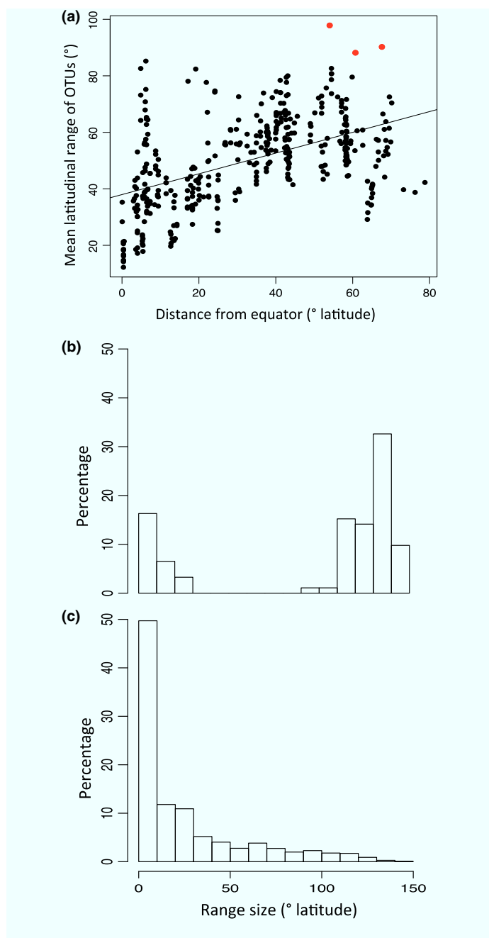
Figure 4 Characteristics of latitudinal range sizes of Antarctic fungal operational taxonomic units (OTUs). (a) Relationship between the mean latitudinal range of OTUs found at each site against the distance of the site from the equator. Points representing the three Antarctic islands are coloured in red. (b, c) Distribution of latitudinal range sizes of (b) Antarctic OTUs and (c) all fungal OTUs from worldwide geographic locations. Bin sizes are 10° latitude.
