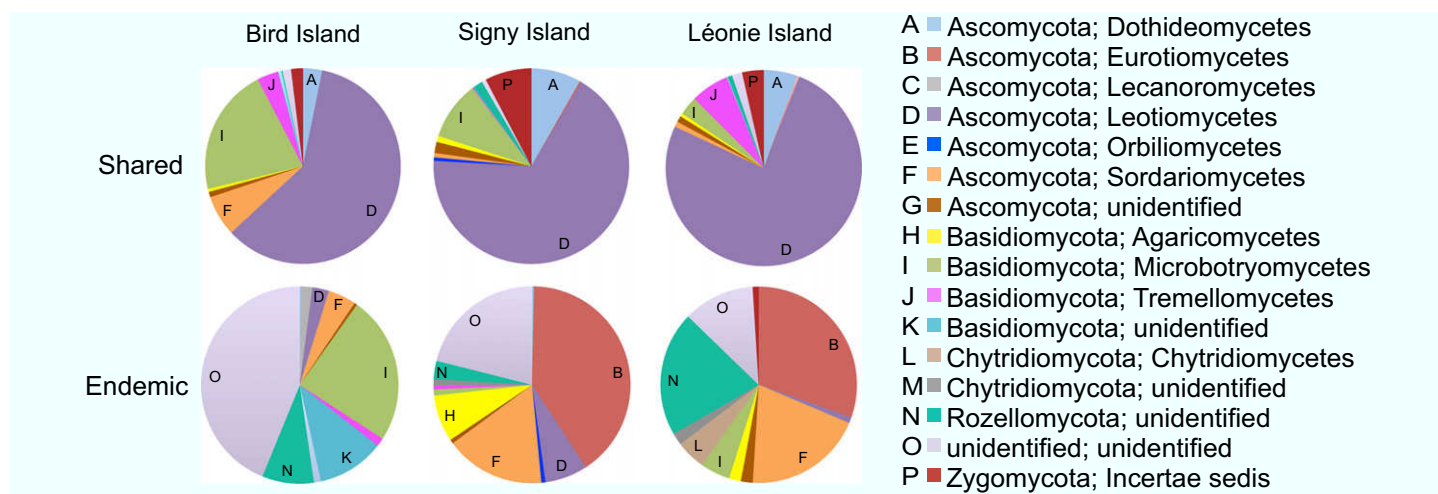
Figure 3 Percentage abundances of 1000 sequences that fell into different taxonomic classes across three Antarctic islands. The top row represents the abundance of Antarctic operational taxonomic units (OTUs) that matched at 97% similarity, sequences in datasets from other parts of the world ('shared'), while the bottom row represents the abundance of those OTUs that were only present in the Antarctic dataset ('endemic'). Segments representing more than 2.5% of the total are labelled with a letter to aid identification.
