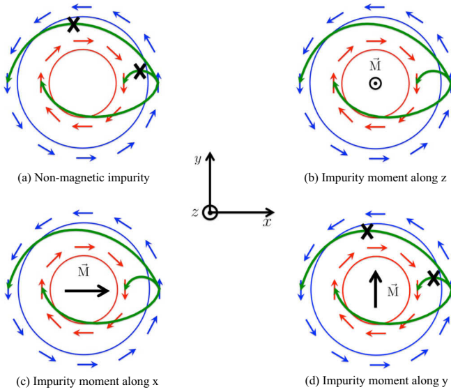
FIG. 3. Fermi-surface scattering processes of Rashba electrons at a (a) nonmagnetic impurity, (b) magnetic impurity with an out-of-plane magnetic moment, (c) in-plane magnetic moment pointing along the x direction, and (d) along the y direction. The transitions between circles with different colors are interband transitions, while transitions between circles with the same color are intraband transitions. The green arrows indicate the connection between the initial and final state. The crosses indicate prohibited scattering processes, while the black arrows at the center of the Fermi contours represent the direction of the impurity magnetic moment.
