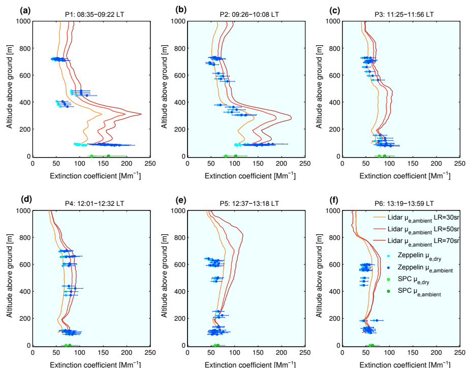
Figure 8. Extinction coefficients for profiles P1 – P6 at different times of day. The lines reflect lidar results for assumed LRs of 30, 50 and 70 sr in orange, red and dark red, respectively. The dots describe in situ results. In light and dark blue, dry and ambient airborne extinction coefficients are shown while the light and dark green dots represent the dry and ambient ground-based results, respectively.
