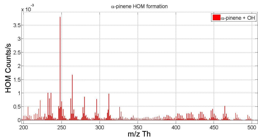
Figure A1. Example mass spectrum from α-pinene photochemical HOM formation entire HOM range.
