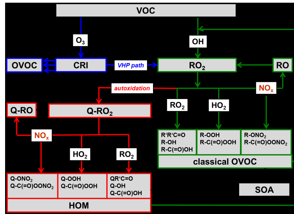
Figure 1.4 Pathways of VOC oxidation. Ozonolysis (blue arrows) also leads to Criegee reactive intermediates (CRI) which on several pathways can form OVOC, similar to those from OH. The vinylhydroperoxide (VHP) path leads to peroxy radicals which can undergo autoxidation. The green frames indicate the established OVOC formation pathway via peroxy radicals (RO 2 ) induced by the OH radical. The red frames show the newly discovered additional pathway via autoxidation (H-shift + O 2 addition). The HOM termination scheme is supposedly similar to the classical scheme, however, the very fast autoxidation process led to higher O/C and functionalization as indicate by using Q. The introduction of NO x in both subsystems increases the importance of alkoxy radicals. OH can sequentially oxidize OVOC to higher oxidation products. Once the vapour pressure is sufficiently low, HOMs (and OVOC) condense and form SOA.
