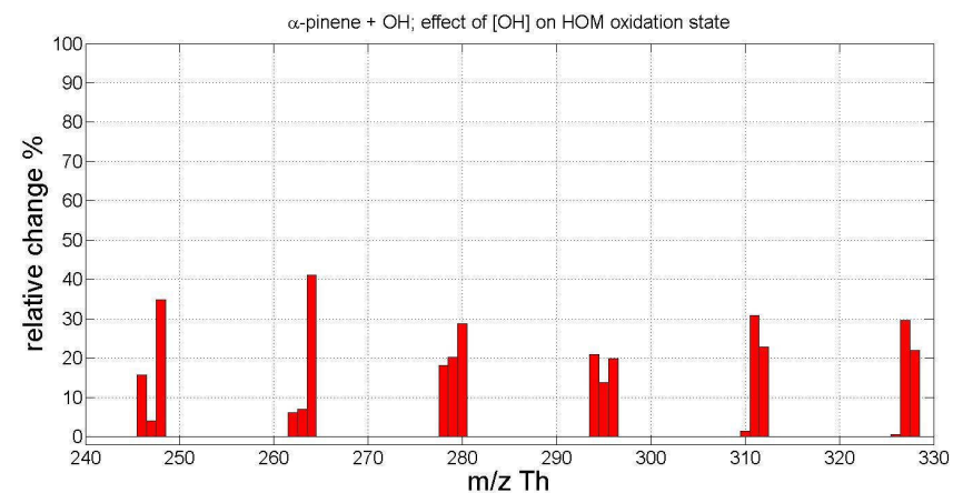
Figure 3.6 Relative increase of selected HOM compounds (order in clusters: ketones, peroxy radicals, hydroperoxides) when comparing \alpha -pinene HOM formation at low and high [OH] shown in Figure 3.5. There is no higher relative increase in closed shell end products with higher oxygen content at higher [OH]. There seems to be a tendency in peroxy radicals of OH enhancement towards higher masses, but as the signals of peroxy radicals are low compared to the other products, small changes may magnify artificially high.
