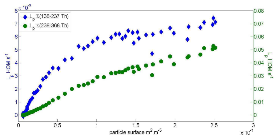
Figure 6.9 Average loss rates of HOMs as a function of particle surface. Green circles show the data for HOMs with higher number of O atoms (238-368 Th), right y-axis. Blue diamonds show the data for HOMs with masses between 138 and 237 Th i.e. for HOMs with lower numbers of O atoms, left y-axis.
