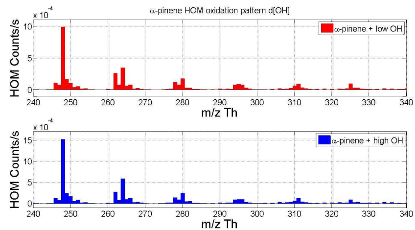
Figure 3.5 Upper panel shows \alpha -pinene HOM formation under lower [OH] conditions ( 1.92 \cdot 10^7 \text{ cm}^{-3} ), and lower same for higher OH concentration ( 4.8 \cdot 10^7 \text{ cm}^{-3} ). If HOM formation would be a result of sequential OH oxidation, an assumption would be that the relative intensities in the lower panel (high [OH]) would be shifted towards higher masses, i.e. higher oxidation states, when compared to the lower [OH] case. The total intensity of HOM formation has increased, but there is no indication that there is higher production of more oxidised HOM molecules. Note the difference in Y-axes.
