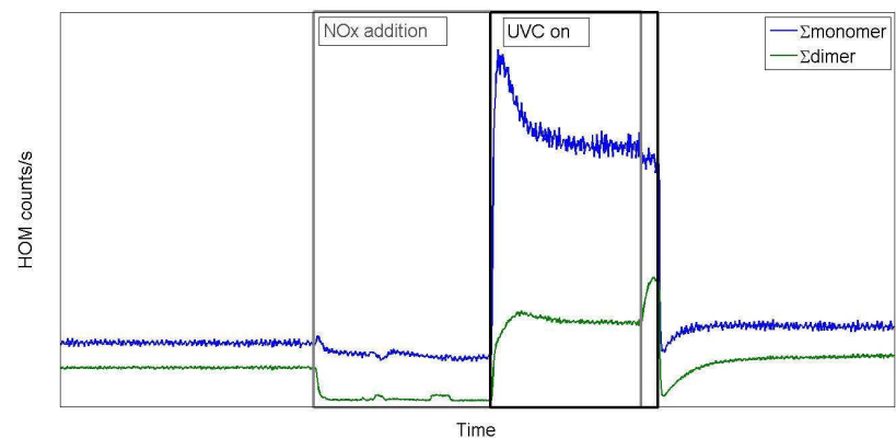
Figure 2.7 Example of NO x dependence experiment run. After NO x addition is started, steady state is waited before starting OH production by switching on UVC lamp. UVA lamp is on during NO x addition to photolyse NO 2 into NO. Ending of a NO x experiment varied, either first stopping NO x addition, or OH production, depending on the goal of the experiment. Time scale is in hours.
