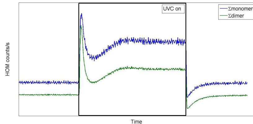
Figure 2.6 Example of experiment run without \text{NO}_x . After chamber has reached steady state under ozone, UVC lamp is turned on to start OH production. Experiment is continued until chamber has reached (pseudo) steady state under OH regime, then UVC lamp is turned off, and experiment ended. Example shown here is with \alpha -pinene HOM production. Time scale is in hours.
