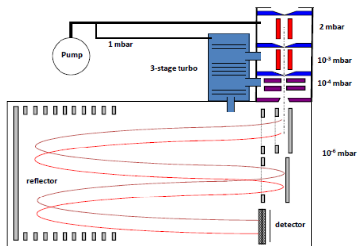
Figure 2.2 Schematic figure of APi-TOF-MS (Junninen et al., 2010). There is no ionization method at this stage; ionization happens at an additional inlet figuration (Figure 2.3). Sampling is done at atmospheric pressure, after which the sample is focused and air is pumped out to reach low pressure ( < 10^{-6} mbar) as used at the TOF region. Time-of-flight mass spectrometer (TOF-MS) is used to mass separate and detect ions. Normal operating mode of TOF-MS in the experiments was the V-mode, which gives somewhat lower mass resolution (3000-4000 Th/Th compared to c. 8000 Th/Th at W-mode), but has better sensitivity, and allows higher time resolution. In experiments shown here, only the V-mode was used. Critical orifice (300 \mu\text{m} ) limits the sample flow into the APi-TOF-MS system to approximately 800 mLPM.
