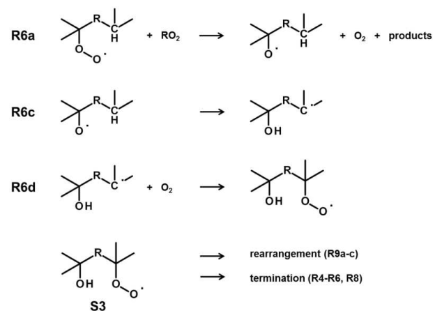
Figure 1.2 Alkoxy-peroxy pathway of alkoxy radical (Mentel et al., 2015).
