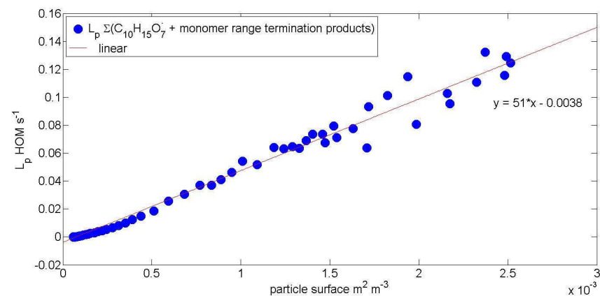
Figure 6.8 Loss rates of the sum of C_{10}H_{14}O_6 (ketone), C_{10}H_{15}O_7 (peroxy radical) and C_{10}H_{16}O_7 (hydroperoxide) as a function of particle surface.
