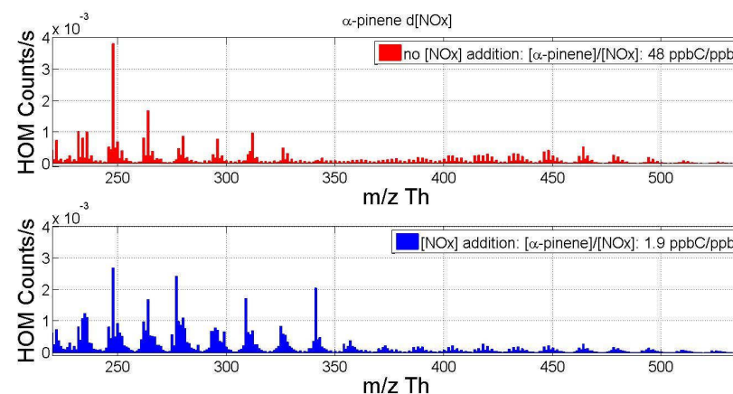
Figure 5.5 Comparison of HOM pattern for low NO_x (upper) and high NO_x (~36 ppb) conditions. Due to addition of NO_x and the subsequent OH recycling, the [OH] in the low NO_x case is 4.6 \cdot 10^7 \text{ cm}^{-3} , and during NO_x addition 4.9 \cdot 10^7 \text{ cm}^{-3} , similar enough to be unlikely to have major effect on the formation rates. The total [monomer] without NO_x is 0.02 counts/s, and total [dimer] 0.012 counts/s. With NO_x addition the total [monomer] increased to 0.04 counts/s, while the [dimers] decreased slightly, to 0.011 counts/s.
