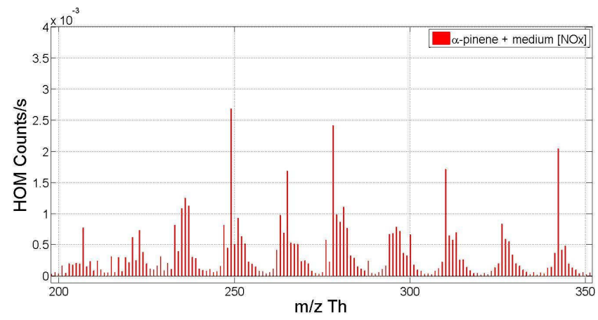
Figure A4. Example mass spectrum from \alpha -pinene photochemical HOM formation with \text{NO}_x monomer range.
