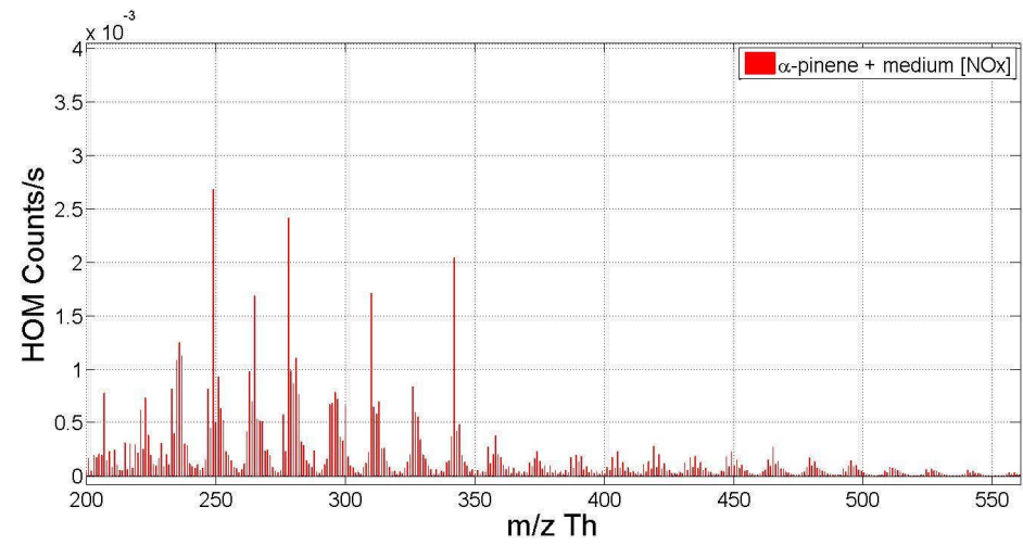
Figure A3. Example mass spectrum from \alpha -pinene photochemical HOM formation with \text{NO}_x entire HOM range.
