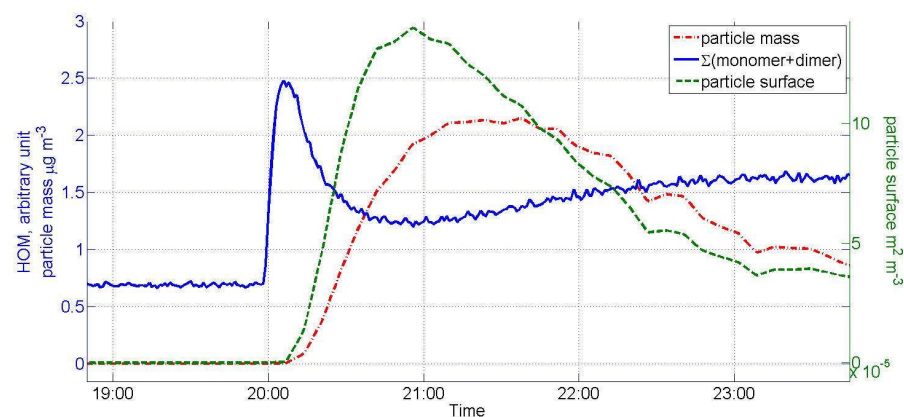
Figure 6.2 Temporal shape of HOM concentrations and particle mass and surface. HOM signal intensities typically show a rapid increase as OH is produced leading to a burst of HOM formation. Green tracer shows the slower increase of particle surface in the chamber. After enough particle surface has been produced to add significantly to sink strength, the HOM concentrations decrease until a maximum in particle surface and a minimum in gas phase concentrations of HOMs is reached. Thereafter, particle surface decreases again, probably due to coagulation which offers the HOMs less particle surface to condense on. Eventually a steady state is reached. For clarity the HOM signal was scaled up.
