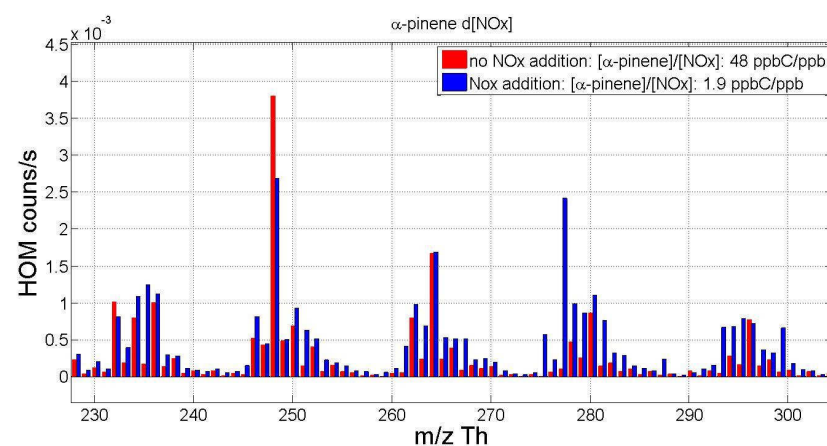
Figure 5.1 Comparison spectra of \alpha -pinene HOM formation pattern under very low \text{NO}_x (red) and high \text{NO}_x conditions (blue). Experimental conditions were [\alpha\text{-pinene}] = 1.45 ppb in the low \text{NO}_x experiment and 1.7 ppb in the high \text{NO}_x experiment, respectively. Measured [\text{NO}_x] during low \text{NO}_x experiment was 0.3 ppb, which gives a ratio [\alpha\text{-pinene}]/[\text{NO}_x] = 48 ppbC/ppb, and at high \text{NO}_x [\text{NO}_x] = 8.7 ppb and 1.9 ppbC/ppb, respectively.
