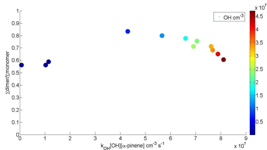
Figure 4.8 Ratio of total dimer to total monomer production as a function of oxidation rate. The Colour indicates the [OH] concentration during measurements. The three points at oxidation rates around 1 \text{ cm}^3 \text{ s}^{-1} or lower were measured at very low [OH] , and thus were likely dominated by ozonolysis. It can be seen that in the ozonolysis dominated system monomer production is proportionally higher than dimer production. Quickly after introducing OH into the system, the relative contribution from monomers decreases, and at k_{OH}[OH][VOC] 4 \cdot 10^7 \text{ cm}^3 \text{ s}^{-1} the relation is 0.9. After this the contribution from dimers lessens slightly, but remains higher than during ozonolysis. The comparison of separate monomer and dimer production rates as function of k_{OH}[OH][\alpha\text{-pinene}] (oxidation rate) is shown in Figure 4.1.
