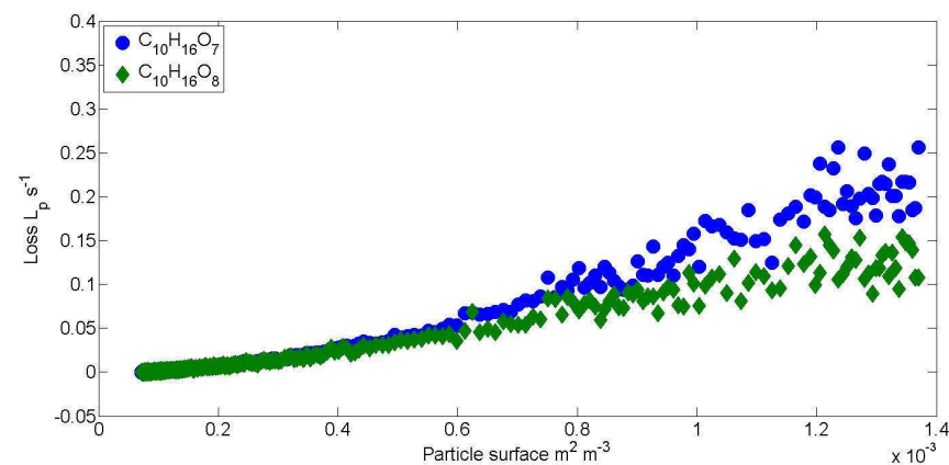
Figure 6.6 Loss rates of HOM from \alpha -pinene as a function of particle surface. [ \alpha -pinene], [OH] and [ O_3 ] were kept constant and particle surface was varied by changing concentration of ammonium sulphate seed (concentration up to 60 \mu\text{g m}^{-3} ). Using all data for the two hydroperoxides shown to determine their effective uptake coefficients would lead to unrealistic high numbers of around 2 to 3 per collision.
