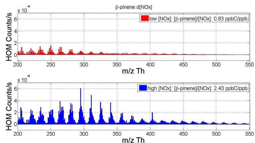
Figure 5.11 Overview of \beta -pinene HOM formation pattern. Upper panel shows \beta -pinene photochemical HOM formation without \text{NO}_x addition ( [\text{NO}_x] \sim 0.75 \text{ ppb} ), lower panel portraits an example of \beta -pinene HOM formation pattern under moderate \text{NO}_x addition (4.1 ppb). OH concentrations in both cases are comparable ( 4.60 \cdot 10^7 at low \text{NO}_x case, and 5.80 \cdot 10^7 with \text{NO}_x ), while \beta -pinene concentrations are 0.06 ppb and 1.0 ppb, respectively. Introducing \text{NO}_x into the system increases HOM formation in monomer range, and causes a shift towards higher oxidation state end products. Compared to \alpha -pinene the higher fragmentation of \beta -pinene is also evident under \text{NO}_x conditions, and can be seen as more “crowded” mass spectra. The monomer range is also seemingly extended towards dimer masses. Total monomer concentration without \text{NO}_x addition is 0.004 counts/s and dimer concentration 0.001 counts/s. With [\text{NO}_x] monomers are 0.02 counts/s and dimers 0.006 counts/s.
