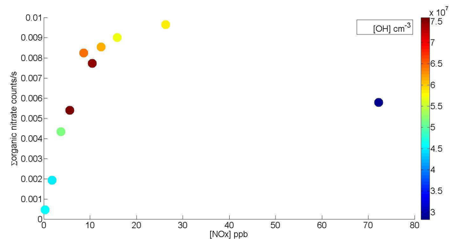
Figure 5.8 Total nitrate HOM production as a function of [NO x ]. Colour code indicates [OH]. Organic nitrate concentration increases rapidly in near-linear way until reaching 80-90% of maximum value at 10-15 ppb [NO x ], after which the formation slows down significantly, but continues to increase until ~30 ppb [NO x ], and then slowly decreases, most likely due to decreasing peroxy radical formation caused by decreased [OH].
