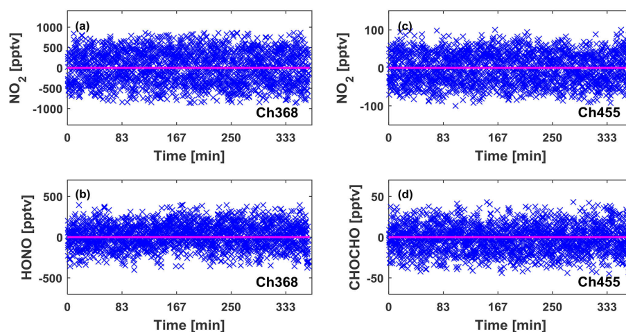
Figure 9. Spectral retrievals for Ch 368 (NO 2 and HONO; left panels) and Ch 455 (NO 2 and CHOCHO; right panels) for zero air measurements acquired during 8–14 June 2014 for CARE Beijing-NCP 2014. Each point represents a 10 s average.
