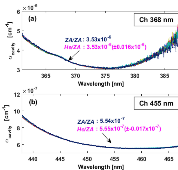
Figure 4. Cavity loss, \alpha_{\text{Cavity}}(\lambda) = (1 - R(\lambda))/d determined using two methods: (1) He and dry zero air (He/Za; magenta) and (2) Za/Za at two different pressures (Za/Za; dark blue). The data are from one SENEX research flight on 5 July 2013. The mean ( \pm 1\sigma ) at 368 and 455 nm pixels for 13 repetitions of He/Za during level flight legs are (3.534 \pm 0.016) \times 10^{-6} and (5.551 \pm 0.017) \times 10^{-7} \text{ cm}^{-1} , respectively, shown as magenta text with varying colored lines. The estimation at those wavelengths from Za/Za using 390 and 812 hPa pressure ( 3.53 \times 10^{-6} and 5.54 \times 10^{-7} ) is in good agreement with He/Za.
