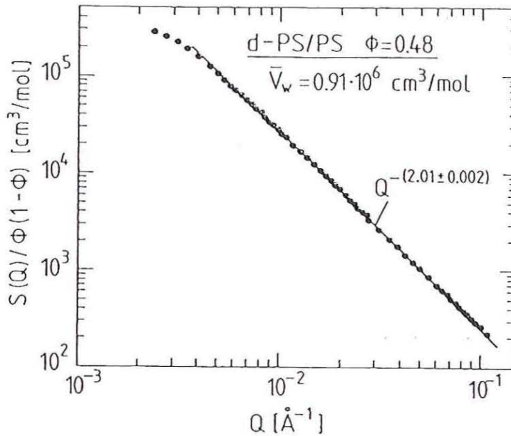
Figure 14.5: Structure factor of a 50% mixture of polystyrene in double logarithmic representation. The power law behavior at large is described by statistical chain
