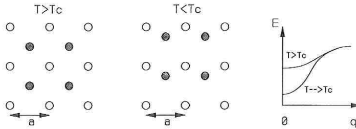
Figure 10 Schematic picture of a displacive phase transition occurring at the zone center and the corresponding dispersion curve.
