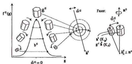
Fig. 18.19: Representation of a texture component g^c by a Gaussian distribution function f(g) of halfwidth b^c . \omega^c denotes the deviation of crystallite orientations from g^c (at \omega^c = 0^\circ ). n^c represents a sample fixed axis (see [10])
