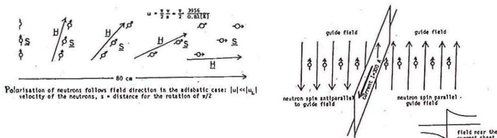
Figure 4.2: Left: \omega \ll \omega_L (adiabatic case), the orientation of the neutron spin follows the field direction; right: \omega \gg \omega_L , the neutron spin keeps its orientation for sudden field changes.[6]
