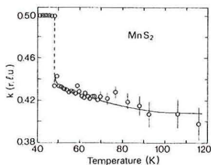
Fig. 16.9: Temperature variation of the incommensurate component.
