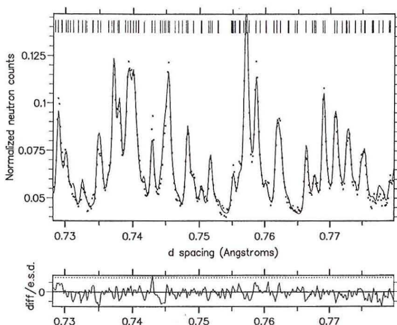
Fig. 9. Powder diffractogram of benzene: (b) enlarged section from 0.73 \text{ \AA} \leq d \leq 0.78 \text{ \AA} The calculated d_{hkl} -values are indicated by the small lines at the top of the upper graph. The quality of the refinement can be judged from the difference in between experimental data and profile calculation in the lower graph.
