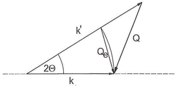
Figure 10.1: Scattering triangle.
