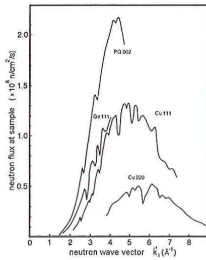
Fig. 9.7: Monochromatic flux at the IN8 (ILL) for various materials as a function of k [3]
