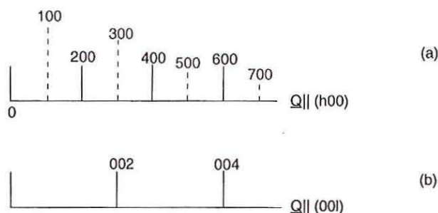
Fig. 16.3: Schematic plot of a neutron diffraction diagram for the antiferromagnet of fig. 16.2. Top: along the (h00) direction; bottom: along (00l) . Magnetic Bragg reflections are indicated by the broken lines. The height of the lines is representative for the scattered intensity.
