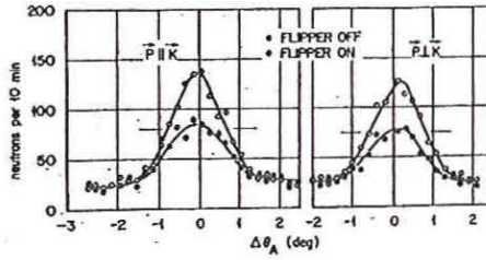
Figure 4.7: Nuclear-spin incoherent scattering from vanadium obtained by rocking the analyzer crystal through the elastic position. The flipper off data are proportional to the (++) cross section and the flipper on data are proportional to the (-) cross section. In contrast to magnetic scattering the result is independent of the neutron polarization with respect to the scattering vector \underline{Q} . [7]
