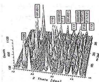
Fig. 18.14: Variation of reflection intensities with \varphi rotation ( \chi fixed) of a quartzite sample measured with a large linear detector in Jülich
