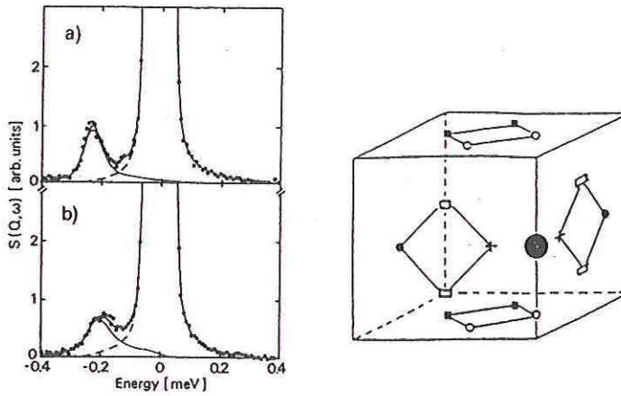
Figure 17.5: Left: Tunnel spectrum of H trapped by O in \text{Nb(OH)}_{0.002} . T=0.1\text{K} . Instrument: IN6, ILL. Top: superconducting, bottom: normal conducting state.
