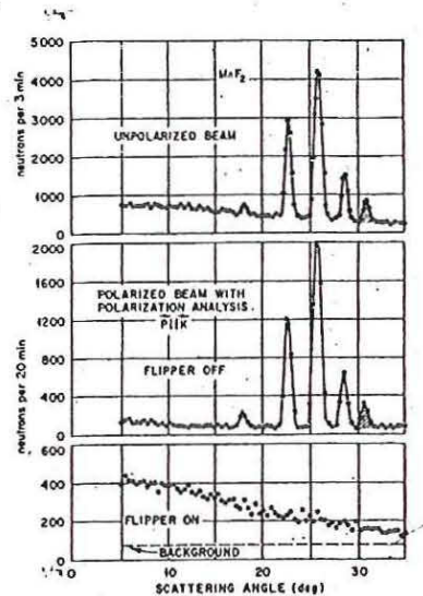
Figure 4.9: Separation of the paramagnetic scattering from \text{MnF}_2 in a powder diffraction pattern.[7]
