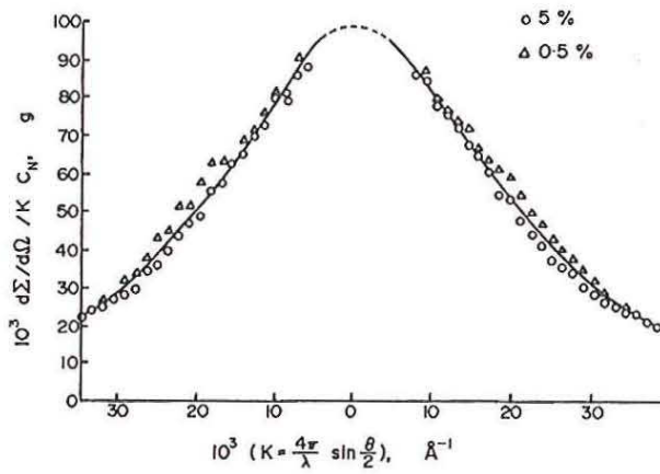
Figure 5.6: Partial differential cross section for protonated polystyrene in a deuterated polystyrene matrix [7]. The concentration of the protonated component is 5% (o) and 0.5% (Δ) respectively. The curve is a fit with the Debye function.
