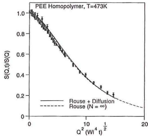
Figure 15.12: Single chain structure factor from PEE melts as a function of the Rouse scaling variable.
