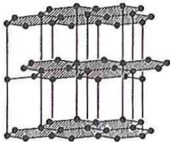
Fig. 18.2: Graphite structure built up by plane sheets of C atoms (hatched) arranged perpendicular to the hexagonal c-axis
