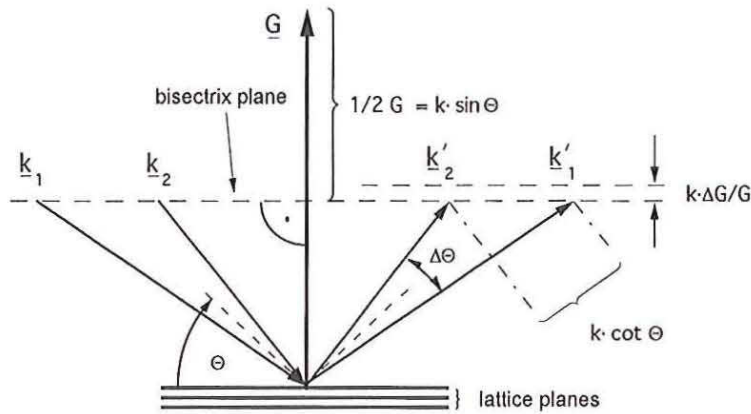
Fig.9.5: Illustration for the selection of scattered wave vectors and their divergence as determined by the modulus G and the scattering angle. \Delta\Theta is of the order of 10^{-4} .
