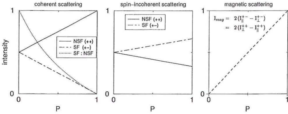
Figure 4.4: Non-ideal experimental conditions for polarization analysis shown for coherent, spin-incoherent and paramagnetic scattering. The polarization factor of the instrument, P < P_{ideal} = 1 , can be determined from the flipping ratio SF:NSF for a coherent scatterer, and one can extrapolate to the ideal conditions.
