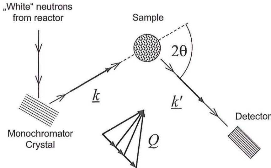
Figure 5.2: Schematic set-up of a diffraction experiment. The inset shows the relation between incident and final wave vectors \underline{k} , \underline{k}' and the scattering vector \underline{Q} .
