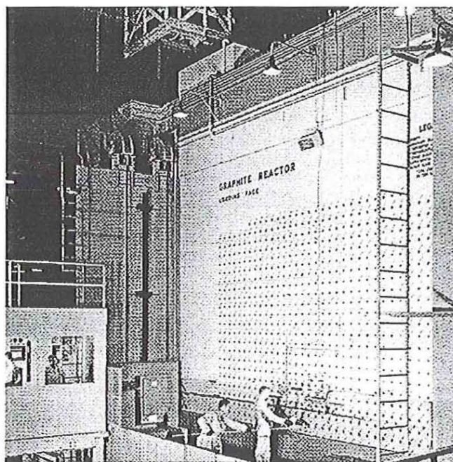
Figure 2.2: View of the Oak Ridge Graphite Reactor.
