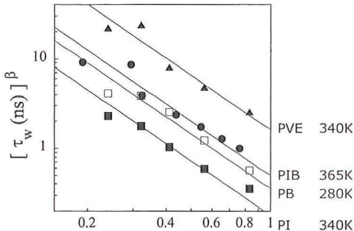
Figure 15.7: (\tau_{KWW})^\beta for 4 different polymers as a function of Q . The solid lines display a Q^2 power law.
