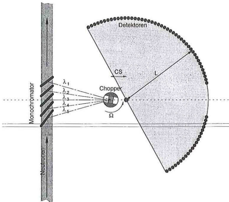
Figure 10.9: TOF-spectrometer with time-focussing.
