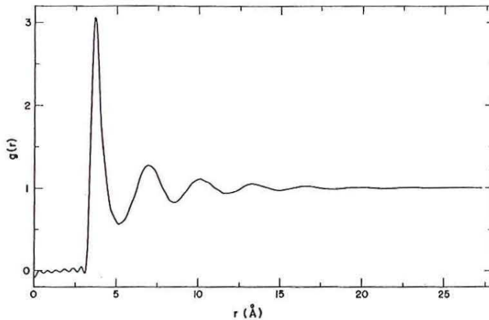
Figure 5.5: The pair correlation function g(r) of liquid Argon calculated by inverse Fourier transform from the data in figure 5.4 [7].
