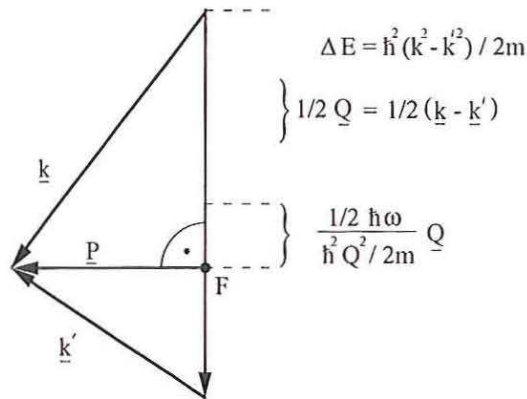
Fig.9.2: Geometrical relation between wave vectors \underline{k} and \underline{k}' on the one hand side to momentum- \hbar \underline{Q} and energy transfer \hbar\omega on the other hand. Since (\underline{k}, \underline{k}') represents 6 dimensions, yet (\underline{Q}, \omega) 4 dimensions, only, arbitrary solutions of vector \underline{P} on the plane perpendicular to \underline{Q} result for a given (\underline{Q}, \omega) -point.
