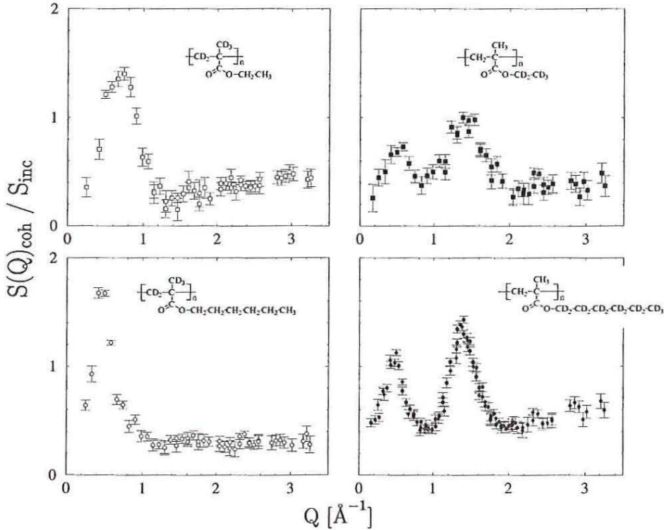
Figure 4.17: Coherent structure factor of a partially deuterated polymer. Note that by separation of the coherent and incoherent scattering one obtains a precise absolute intrinsic calibration. Two measurements are displayed in the figure ( bottom right ) [with \lambda = 3.3 \text{ \AA} (diamonds) and \lambda = 5.3 \text{ \AA} (circles)] demonstrating the excellent reproducibility of the data. The peak at lower Q is due to inter-chain correlations between different polymer “backbones” and the peak around Q \approx 1.4 \text{ \AA}^{-1} can be related to intra-chain correlations along the polymer, the ones between the side-chains of a polymer.
