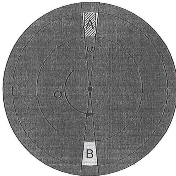
Figure 10.7: Disc chopper.
