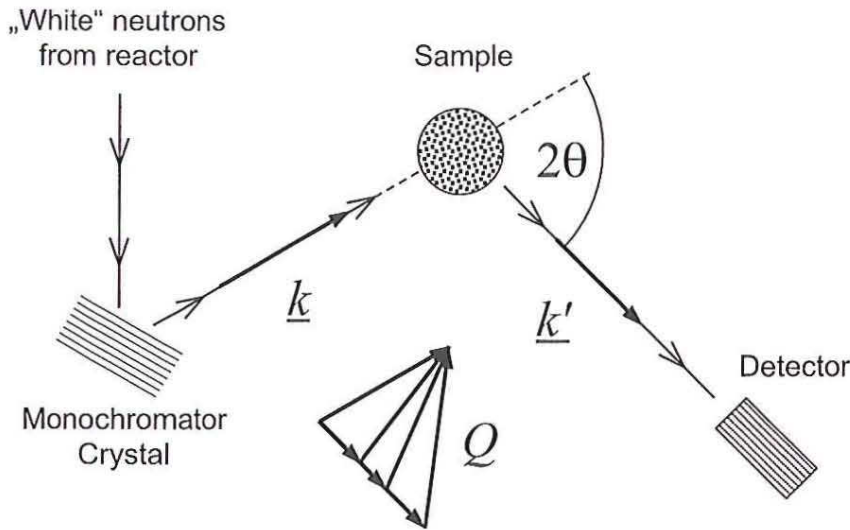
Figure 5.2: Schematic set-up of a diffraction experiment. The inset shows the relation between incident and final wave vectors \underline{k} , \underline{k}' and the scattering vector \underline{Q} .
