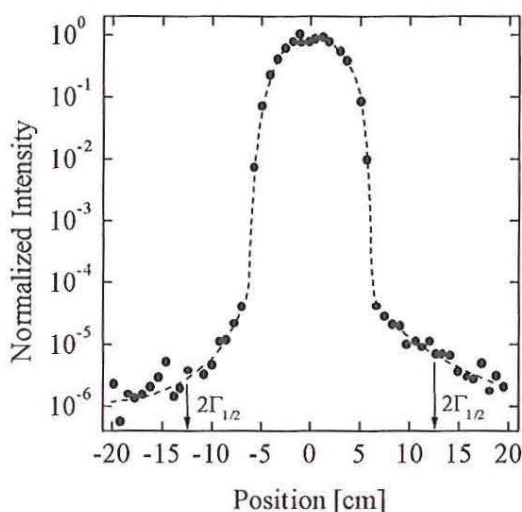
Figure 8.4: Resolution curve for a given configuration
