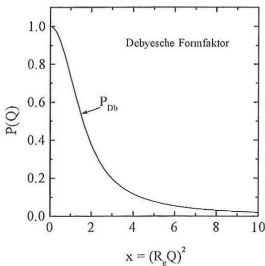
Figure 14.3: Debye form factor of a linear chain
