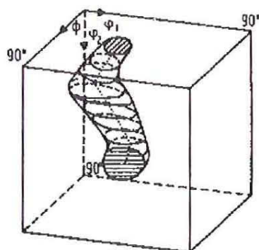
Fig. 18.9: ODF of a Cu rolling texture represented by an equilevel orientation surface in the 3-dim
