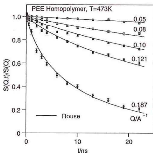
Figure 15.11: Single chain structure factor from a PEE melt at 473\text{K} . The solid lines represent a joint fit with the Rouse model.
