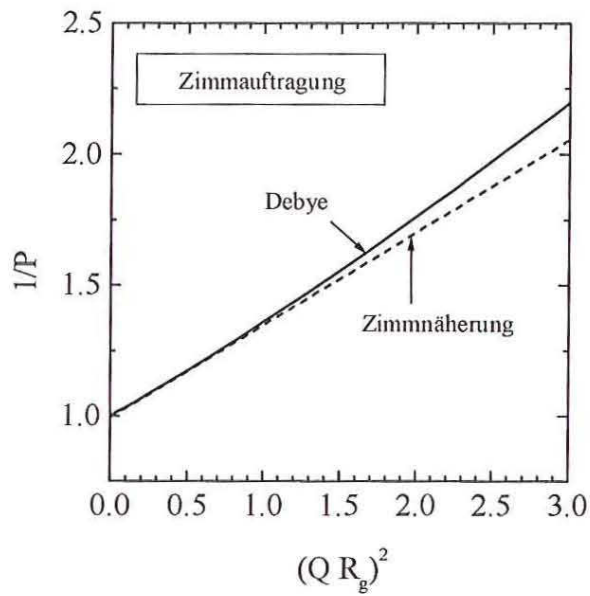
Figure 14.4a: So-called Zimm representation: Within the Zimm approximation the plot of 1/P versus Q^2 gives a straight for the Debye form factor. The slope of the straight line is proportional to R_g .
