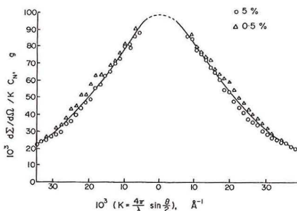
Figure 5.6: Partial differential cross section for protonated polystyrene in a deuterated polystyrene matrix [8]. The concentration of the protonated component is 5% (○) and 0.5% (Δ) respectively. The curve is a fit with the Debye function.
