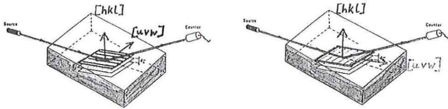
Fig. 19.18: Scattering experiment with scattering vector \underline{\varepsilon} = [hkl] perpendicular to scattering plane (hkl) (hatched) yields no information on the orientation of any [uvw] inside the plane
