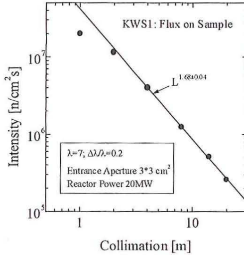
Figure 8.3: Sample intensity for different length of collimation
