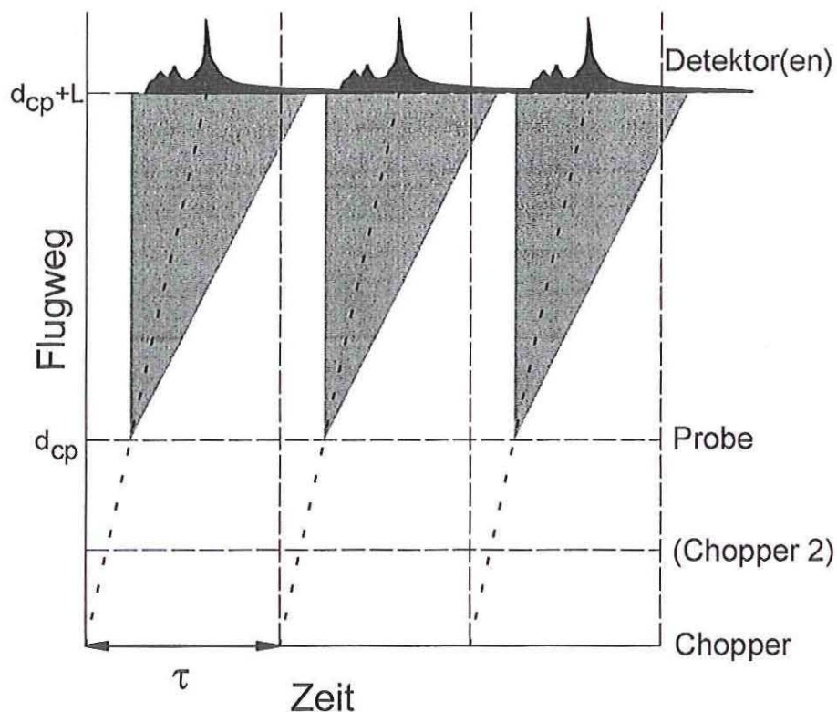
Figure 10.3: Path(Flugweg)-time(Zeit) diagram.
