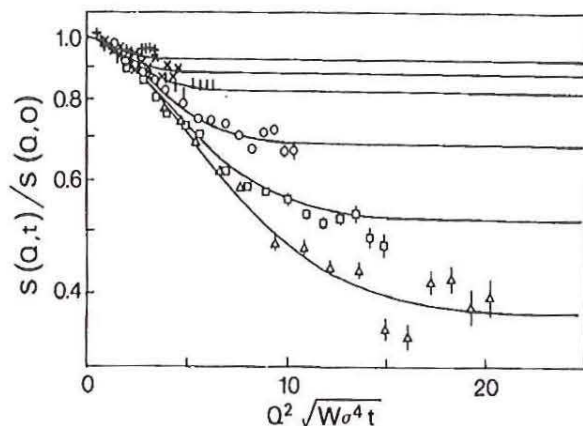
Figure 15.18: Data from Fig.15.17 in a scaling representation as a function of the Rouse variable ( \sigma \equiv \ell )
