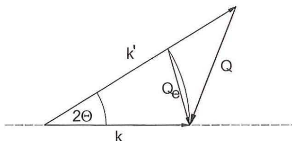
Figure 10.1: Scattering triangle.
