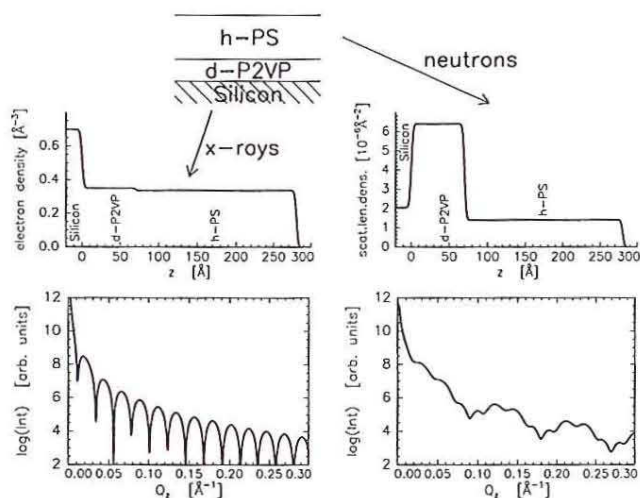
Figure 6.11: Comparison of an x-ray (left column) and a neutron (right column) reflectivity of a polymer bilayer ( 210 \text{ \AA} polystyrene [PS] on 70 \text{ \AA} deuterated polyvinylpyrrolidone [d-P2VP] on a silicon substrate). The x-ray contrast between the two polymers given by the electron density is only about 5%.
